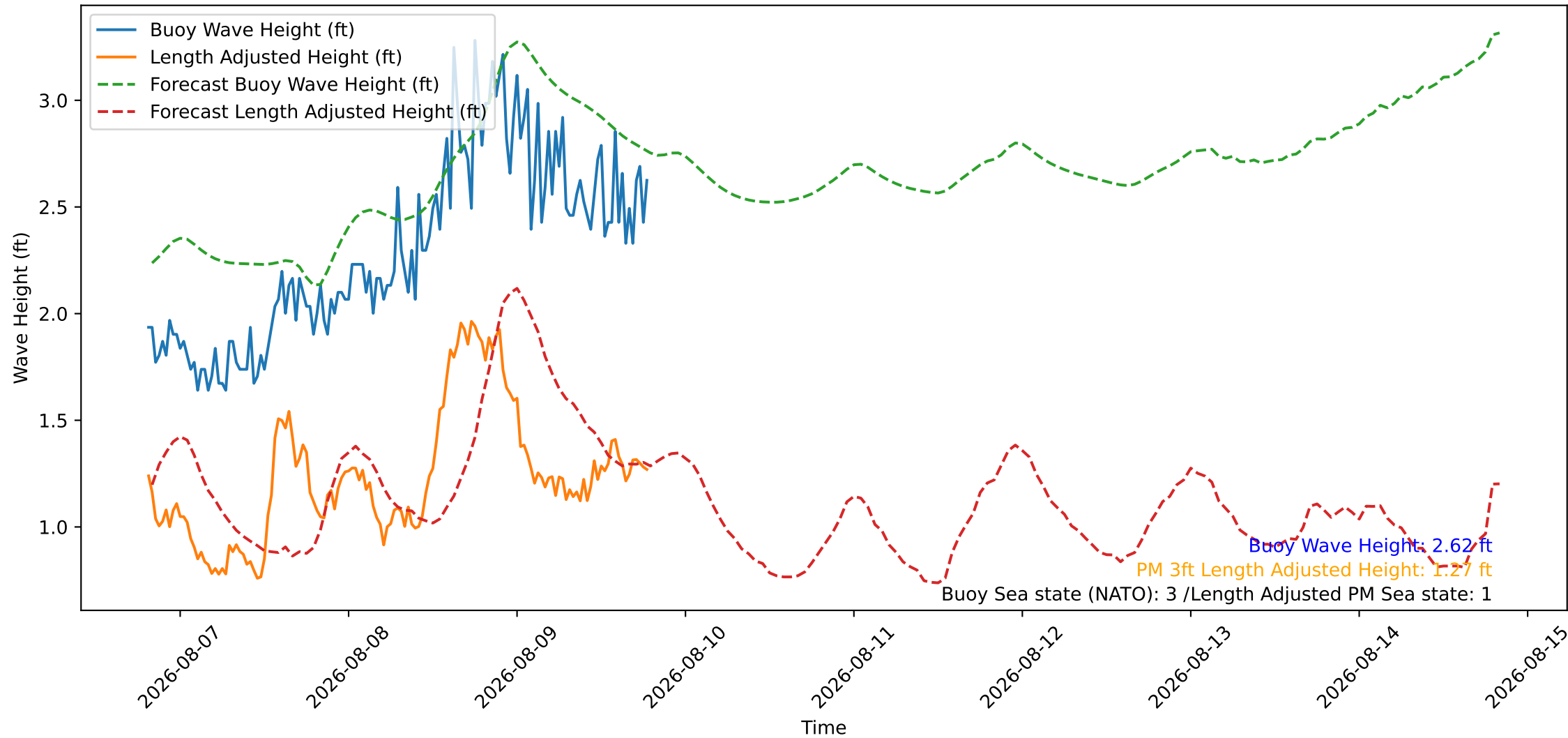
Wave Heights over Time for Oceanside Harbor at 2026-08-09 19:30:26
