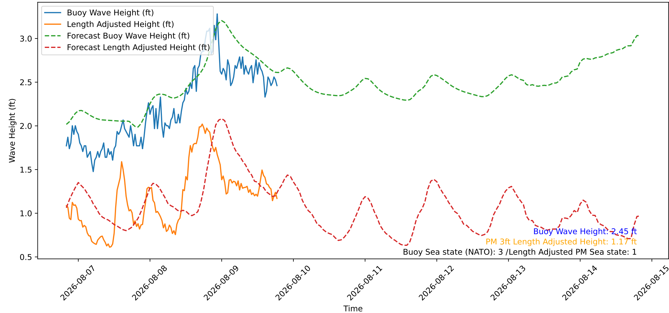
Wave Heights over Time for Red Beach at 2026-08-09 19:30:46
