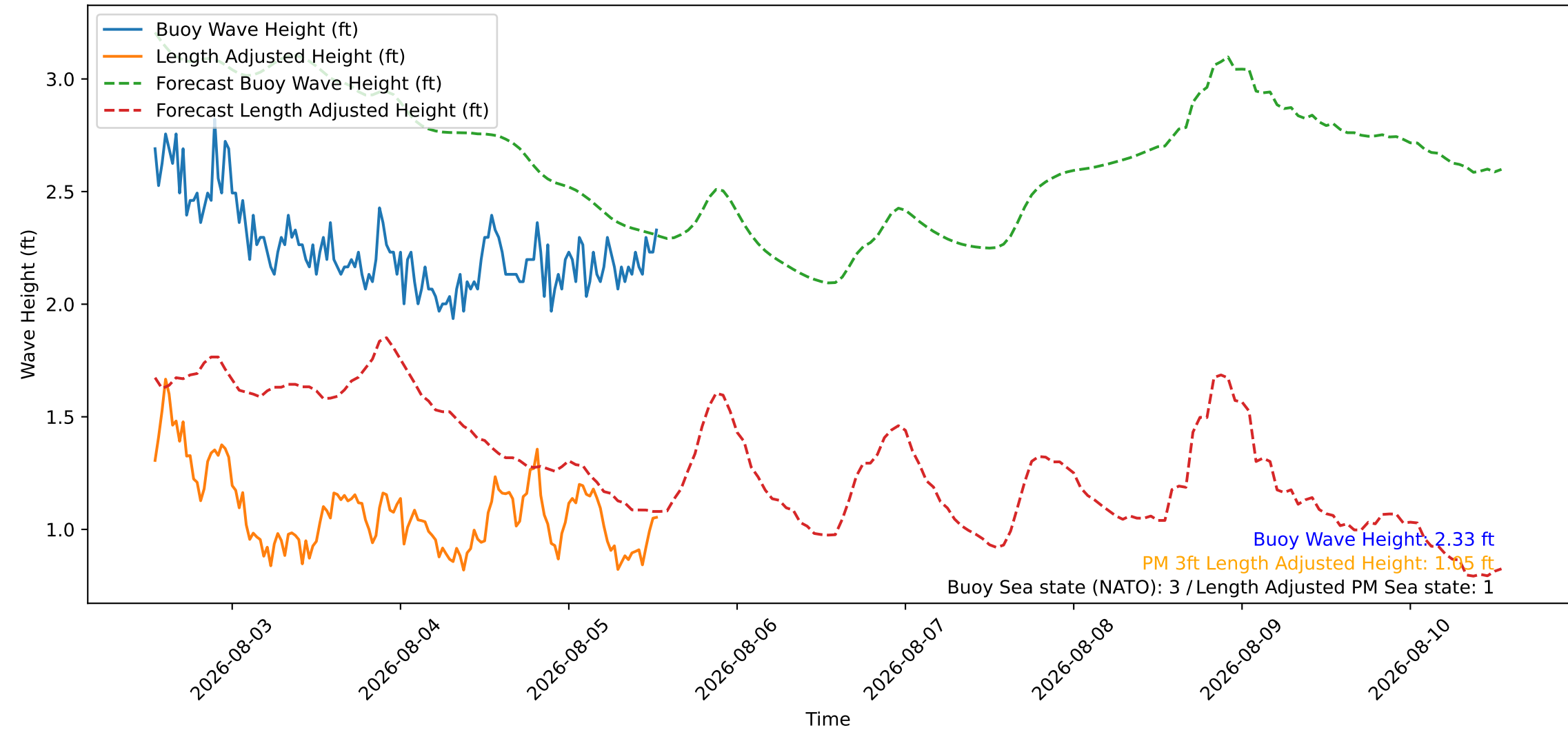
Wave Heights over Time for Green Beach at 2026-08-05 13:11:08
