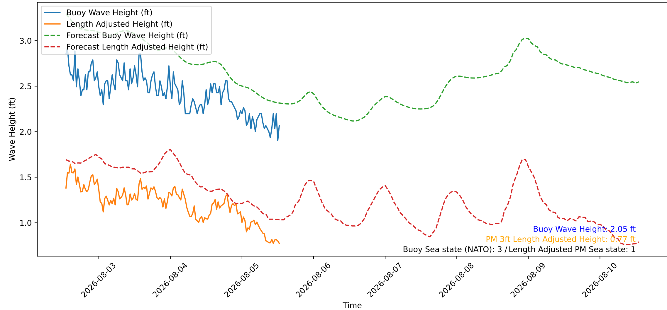
Wave Heights over Time for Oceanside Harbor at 2026-08-05 13:10:26
