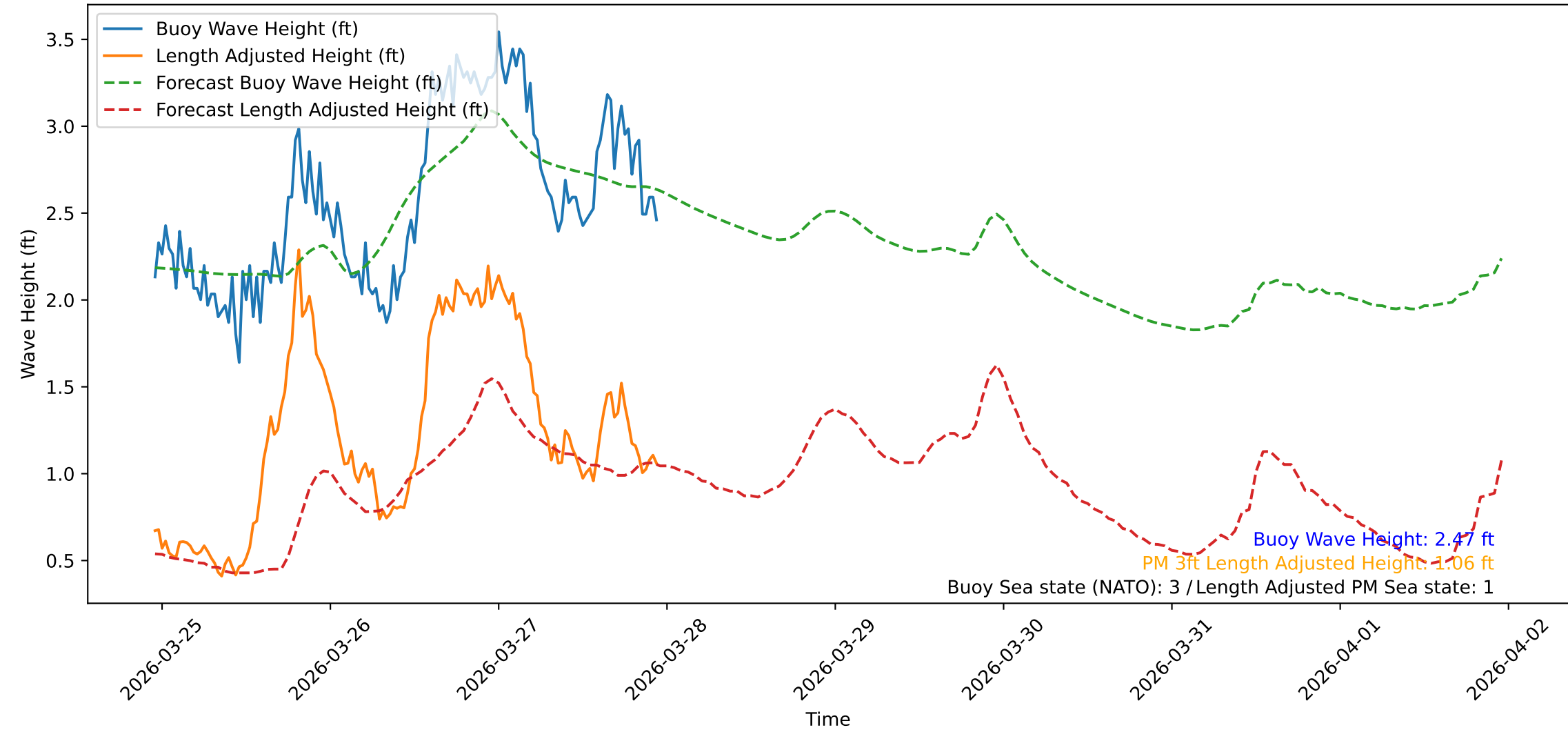
Wave Heights over Time for Green Beach at 2026-03-27 23:11:09
