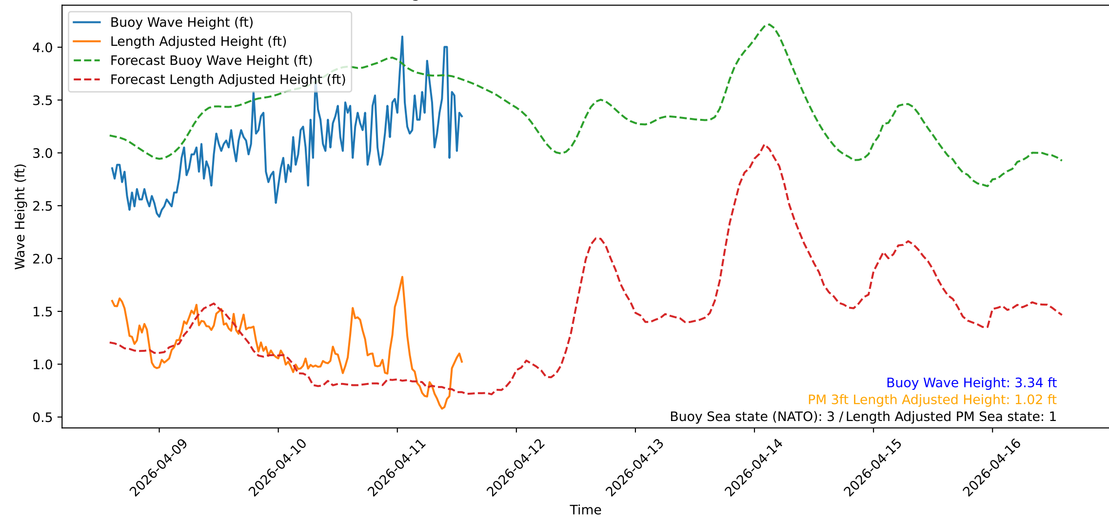
Wave Heights over Time for Red Beach at 2026-04-11 14:10:50
