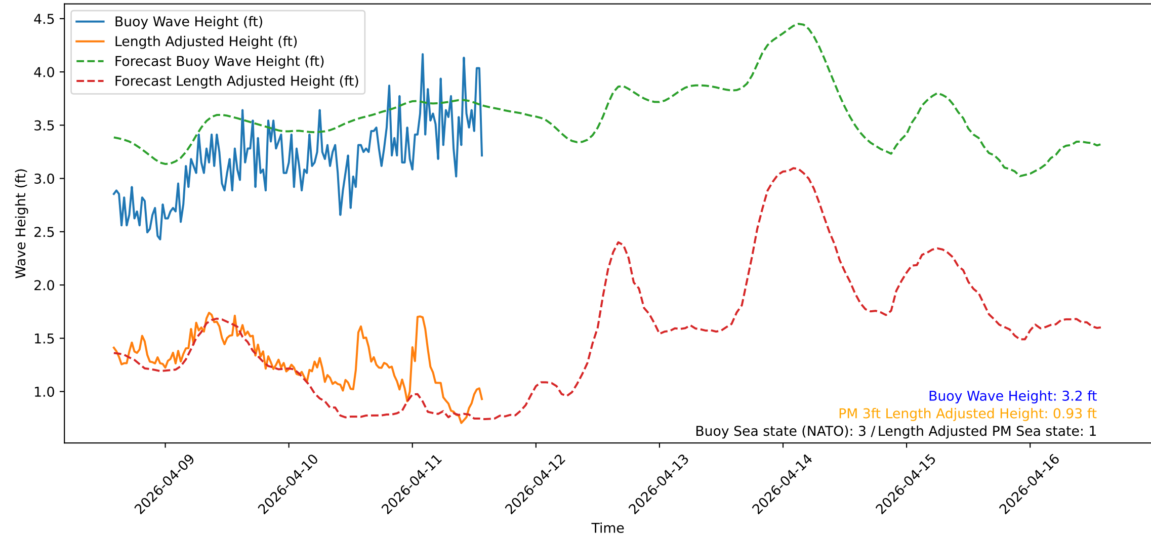
Wave Heights over Time for Oceanside Harbor at 2026-04-11 14:10:31
