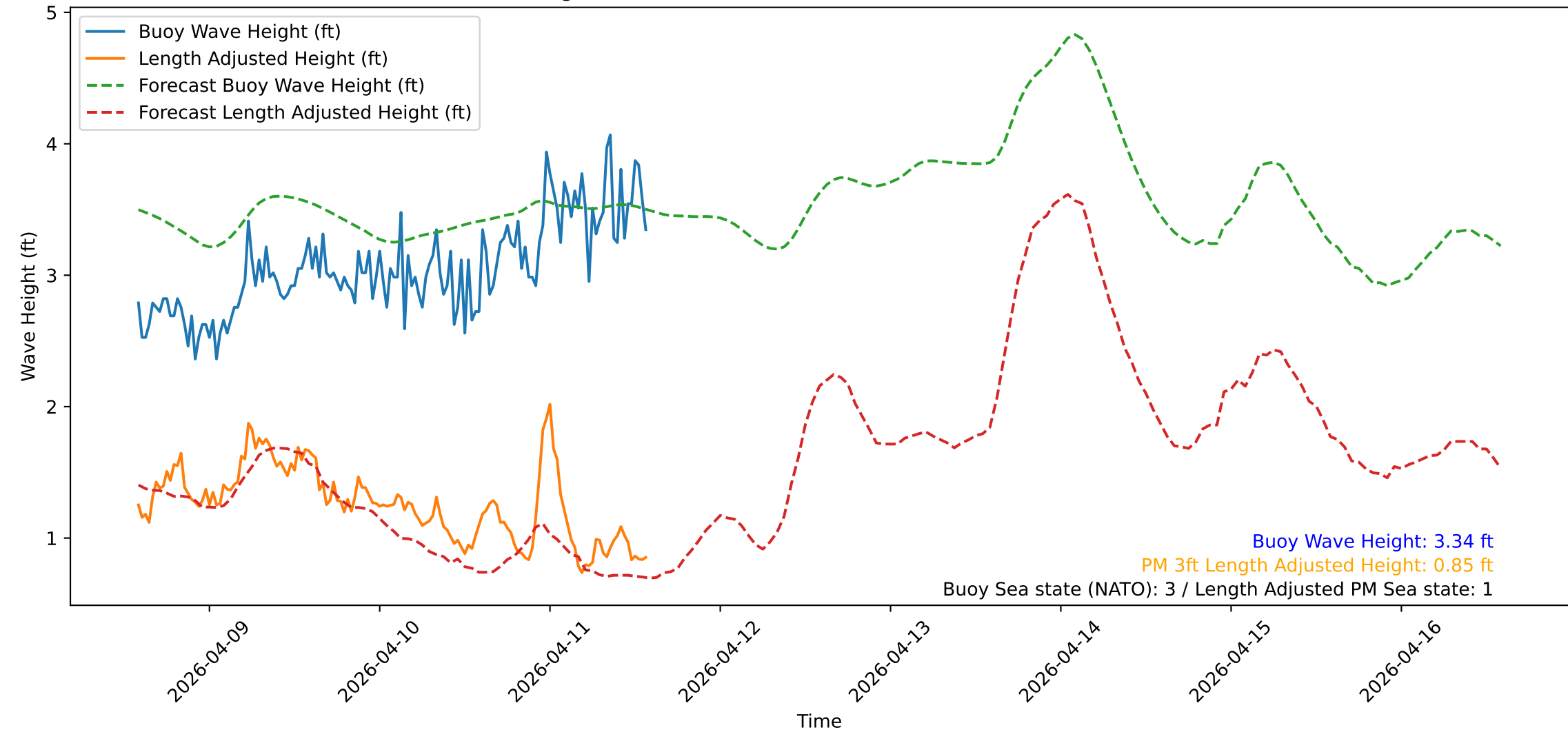
Wave Heights over Time for Green Beach at 2026-04-11 14:11:12
