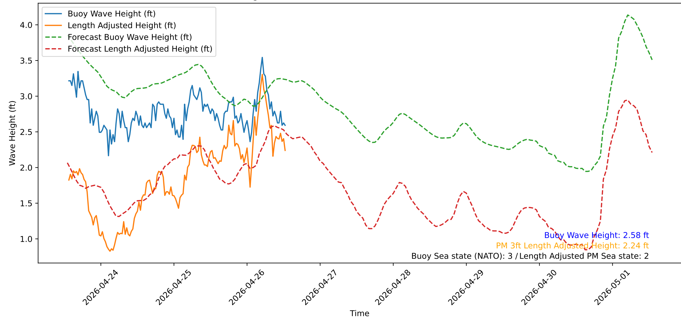
Wave Heights over Time for Red Beach at 2026-04-26 13:20:52
