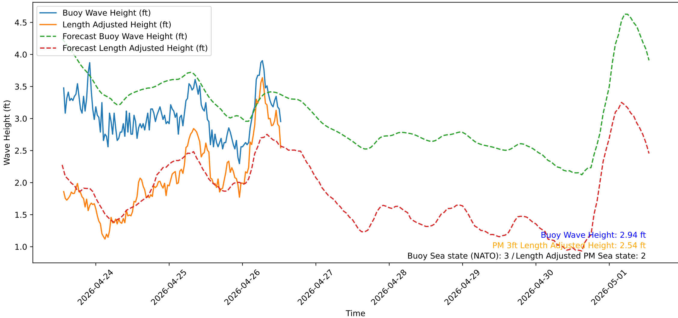
Wave Heights over Time for Oceanside Harbor at 2026-04-26 13:20:32
