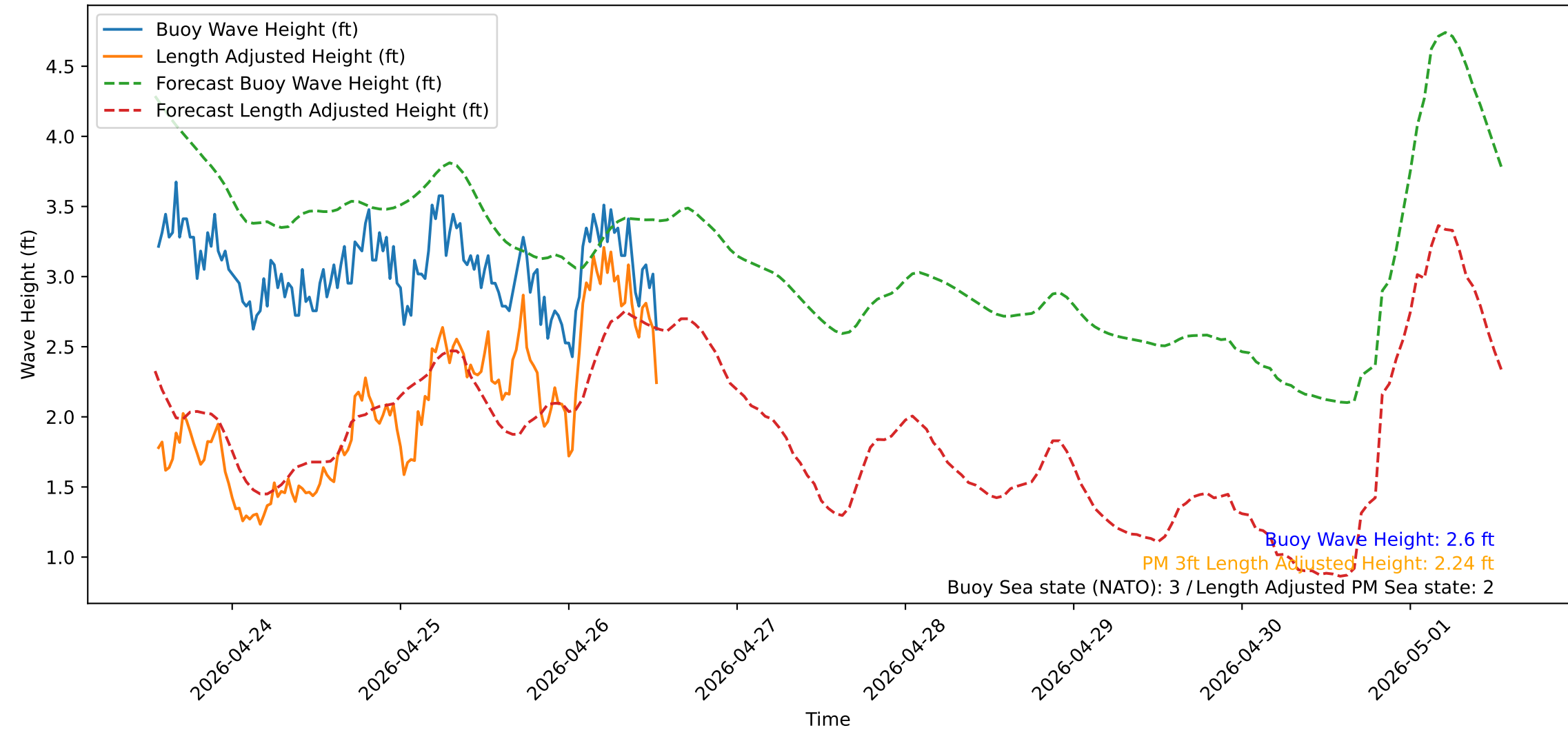
Wave Heights over Time for Green Beach at 2026-04-26 13:21:14
