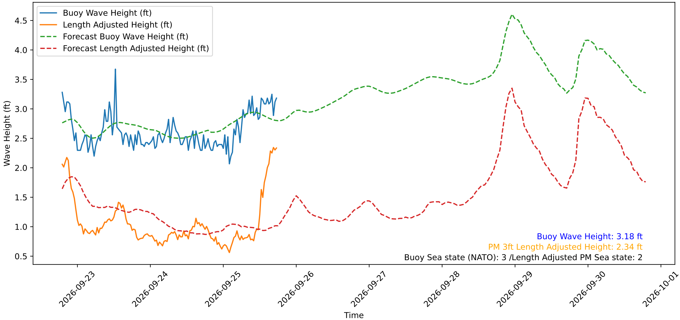
Wave Heights over Time for Red Beach at 2026-09-25 18:30:48
