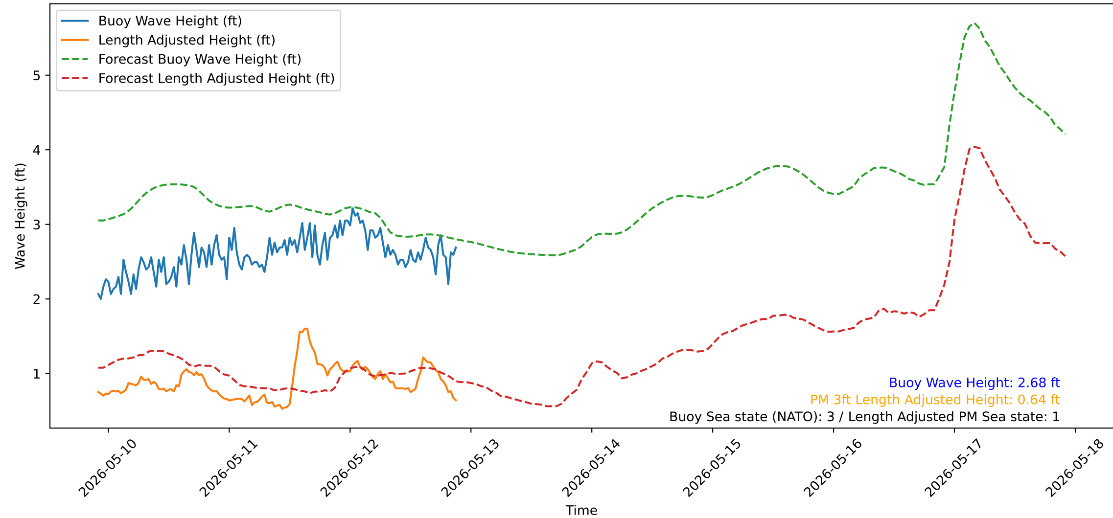
Wave Heights over Time for Red Beach at 2026-05-12 21:40:52
