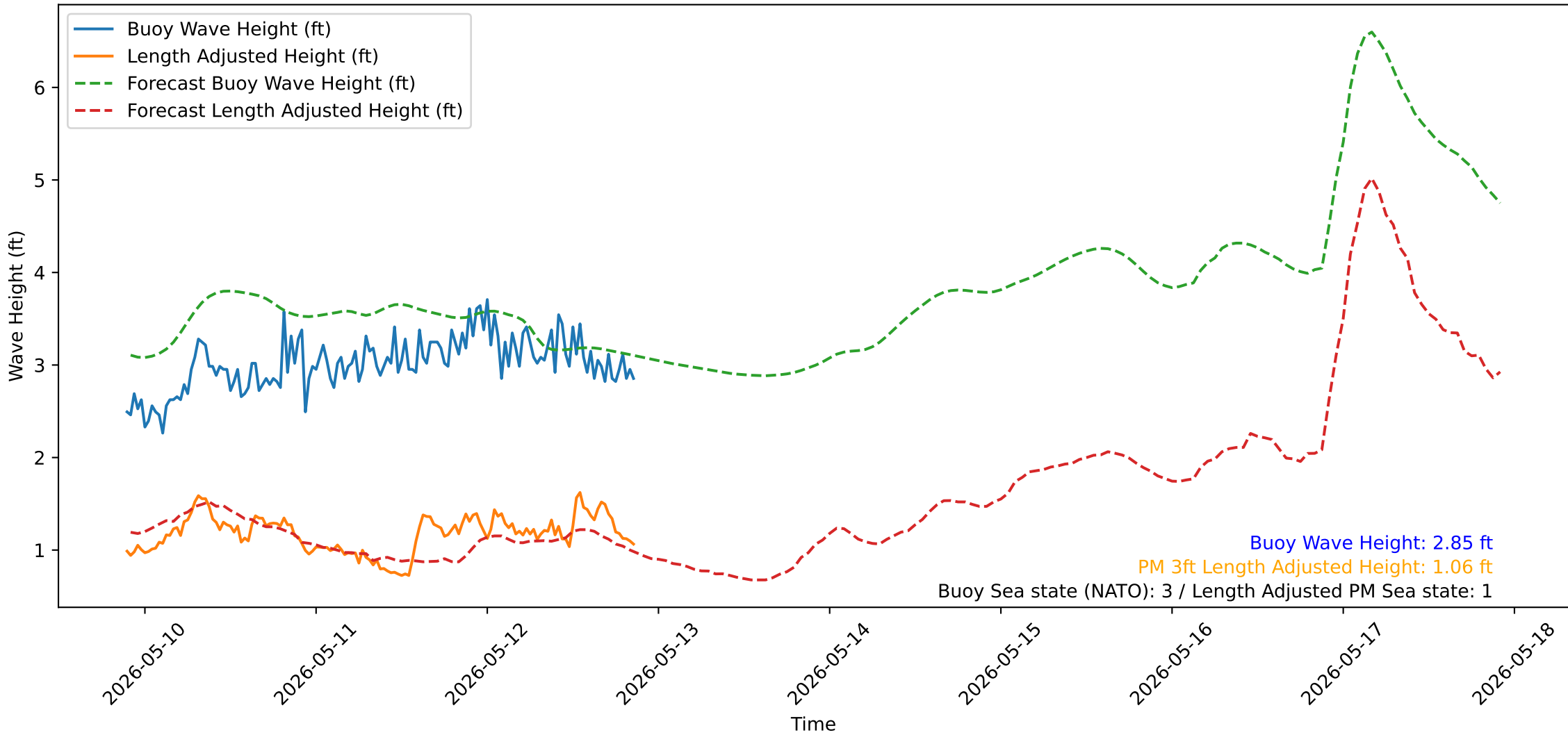
Wave Heights over Time for Oceanside Harbor at 2026-05-12 21:40:32
