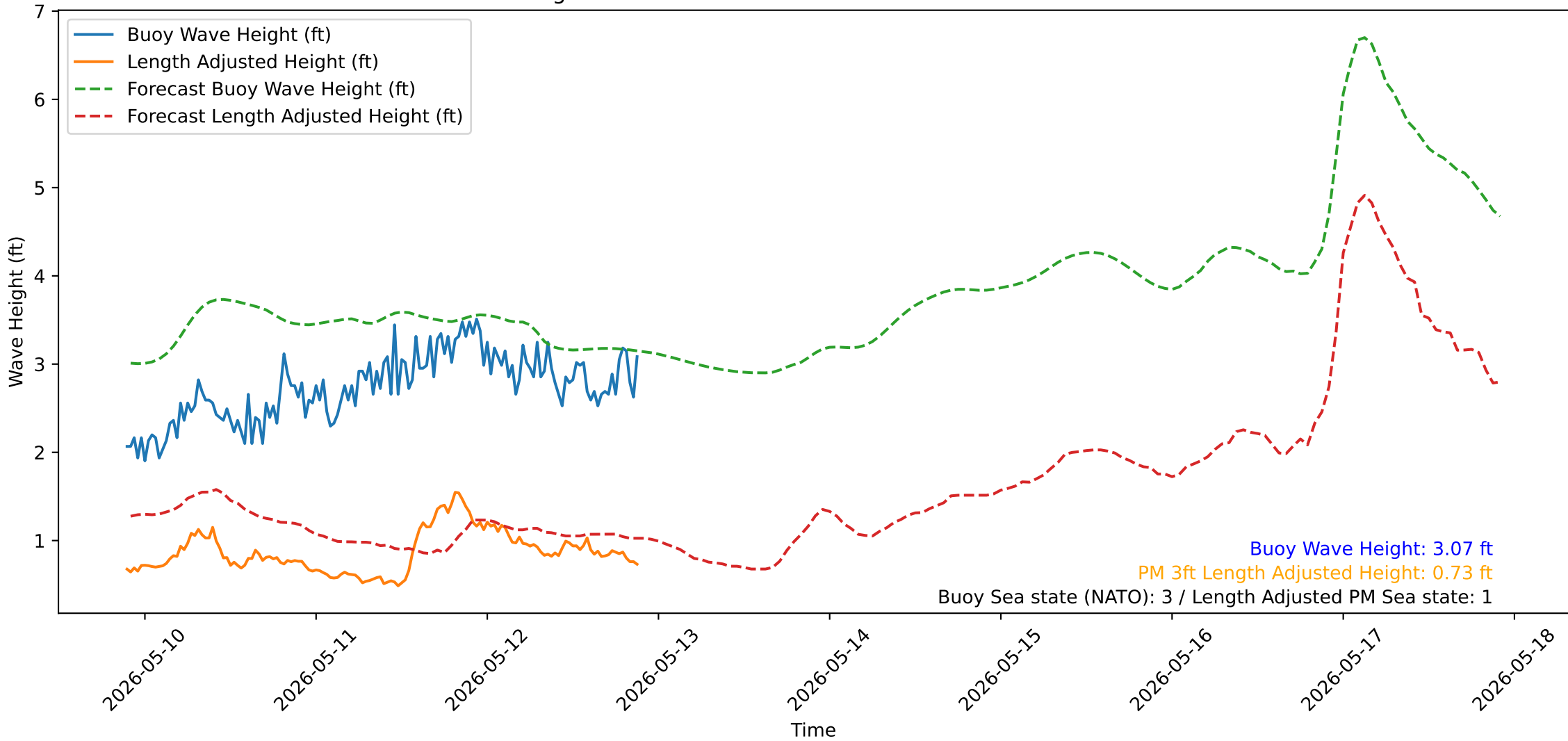
Wave Heights over Time for Green Beach at 2026-05-12 21:41:15
