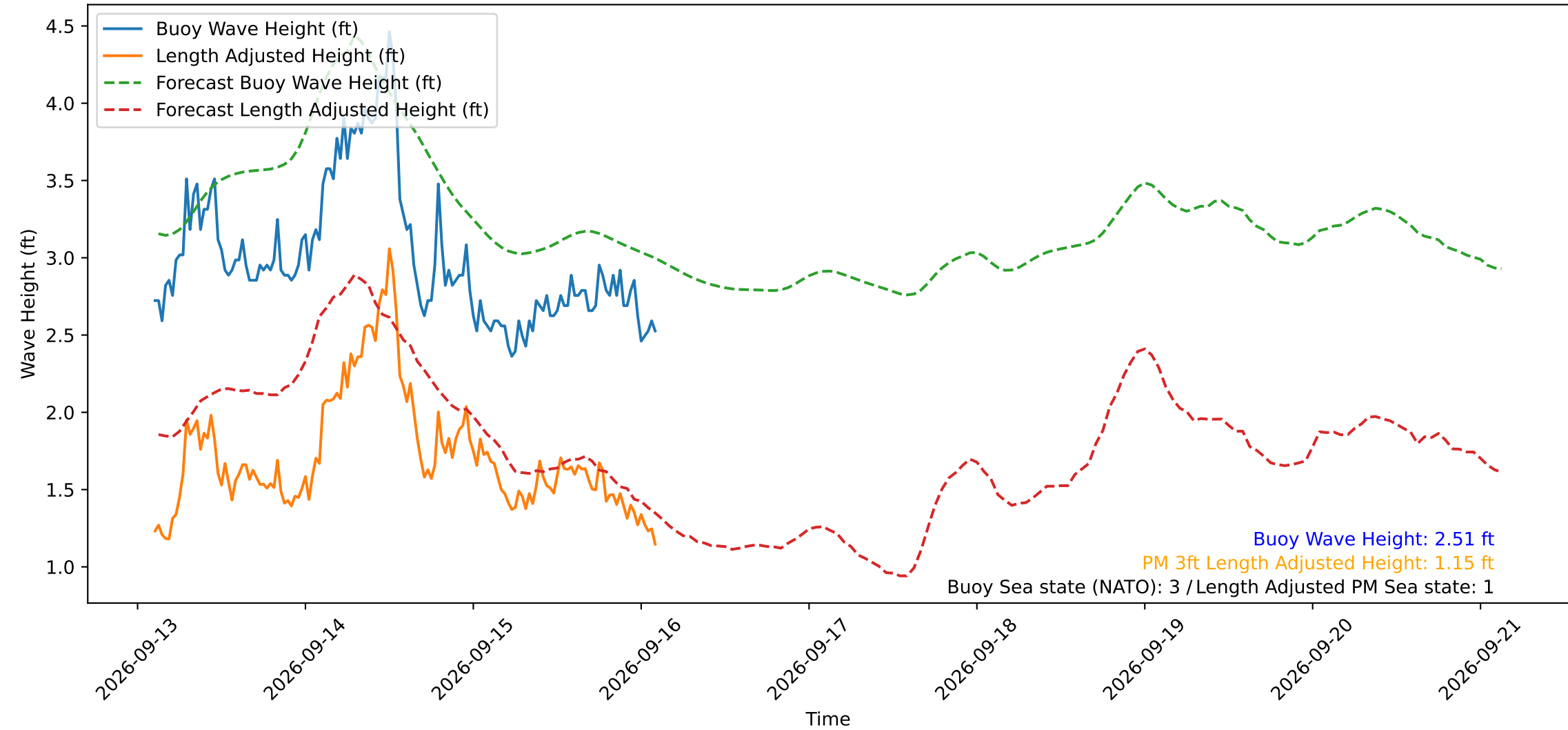
Wave Heights over Time for Oceanside Harbor at 2026-09-16 02:40:29
