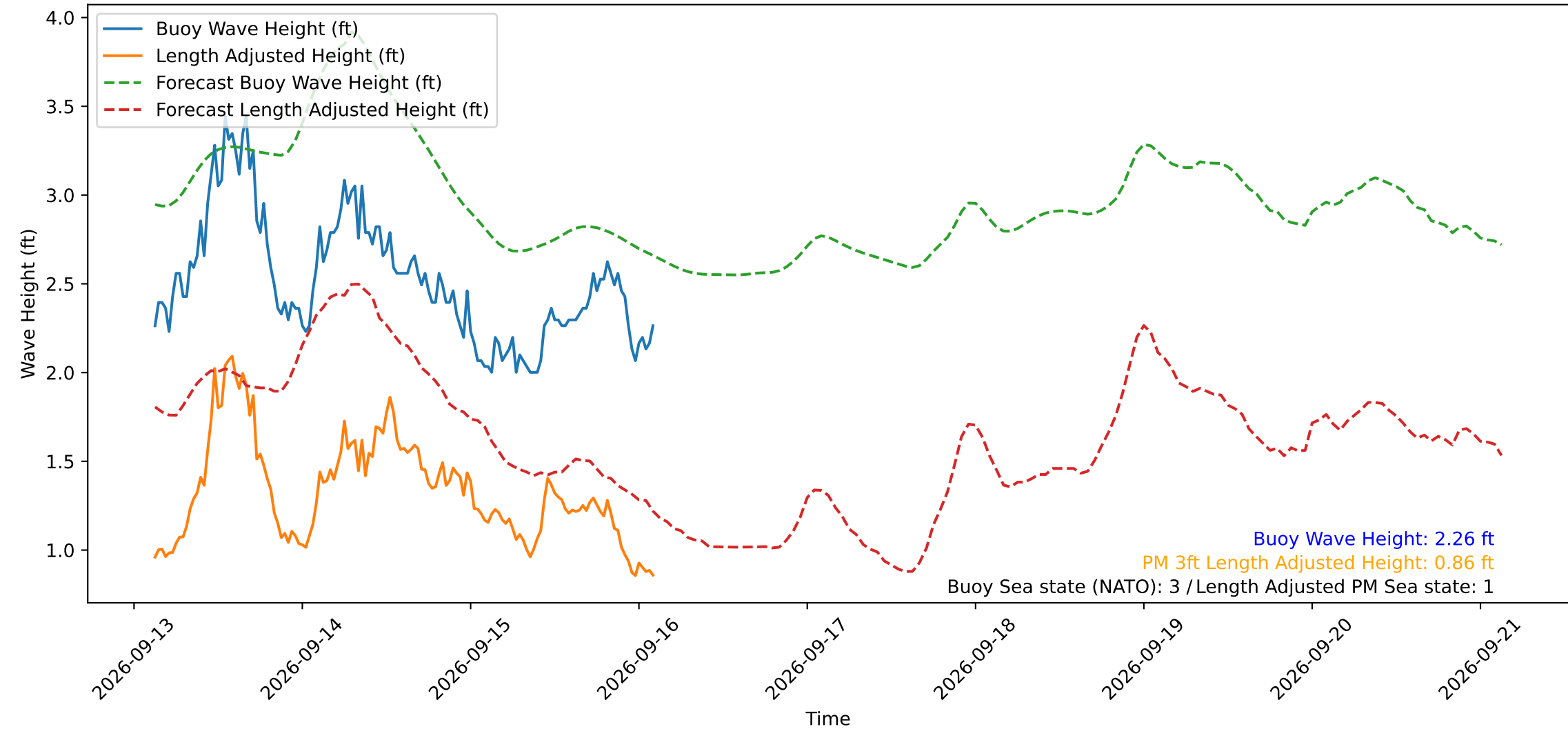
Wave Heights over Time for Red Beach at 2026-09-16 02:40:49
