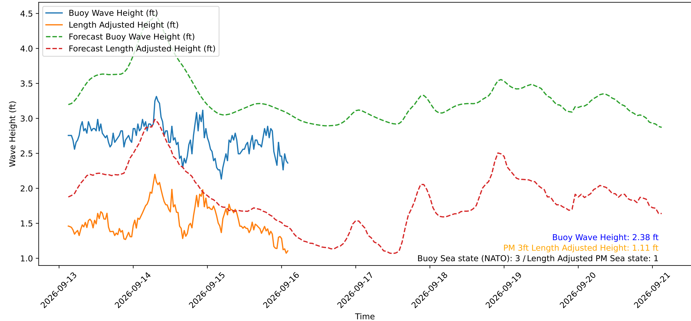
Wave Heights over Time for Green Beach at 2026-09-16 02:41:11
