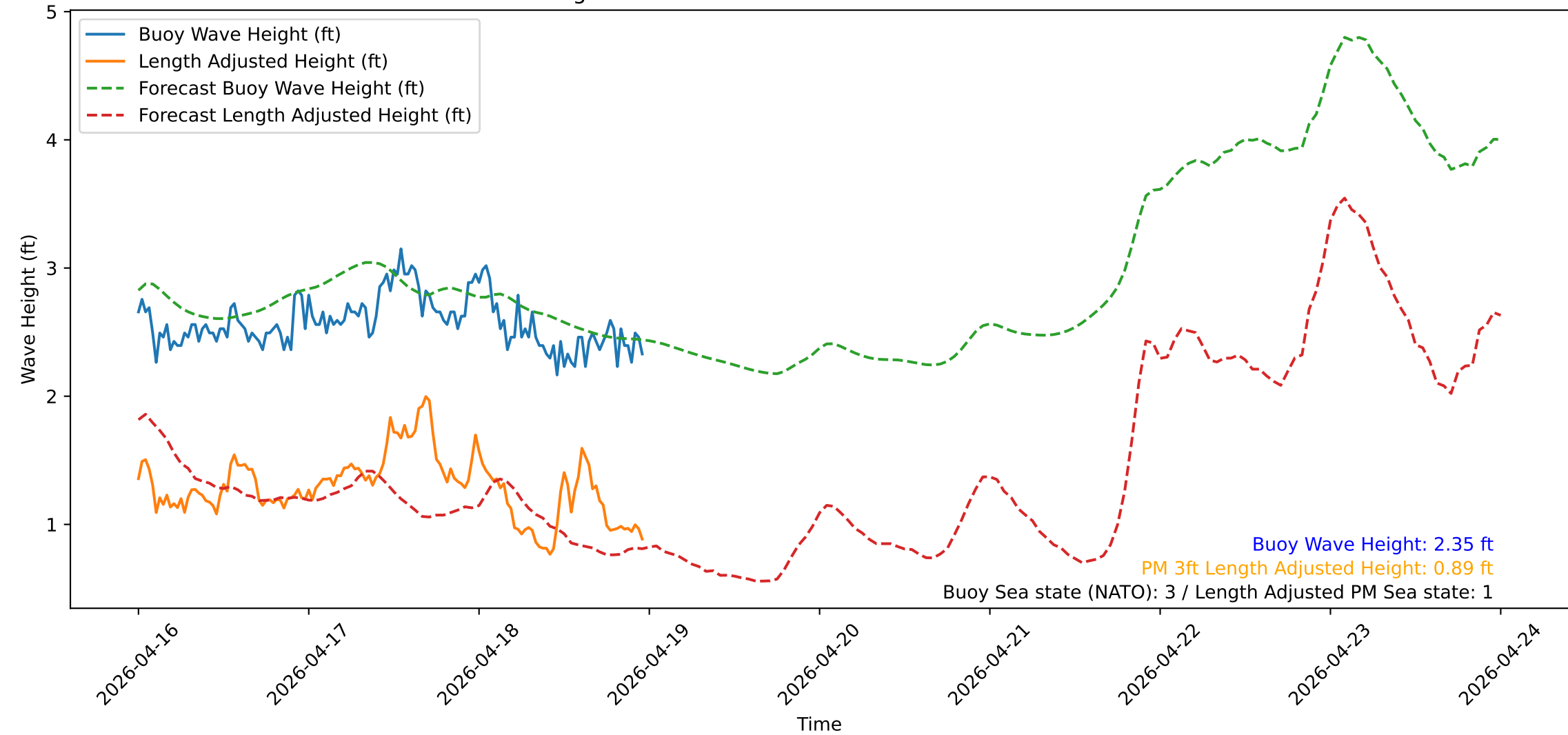
Wave Heights over Time for Red Beach at 2026-04-18 23:40:50
