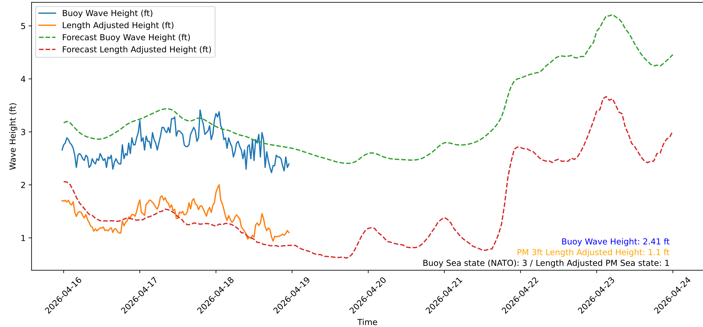
Wave Heights over Time for Oceanside Harbor at 2026-04-18 23:40:31
