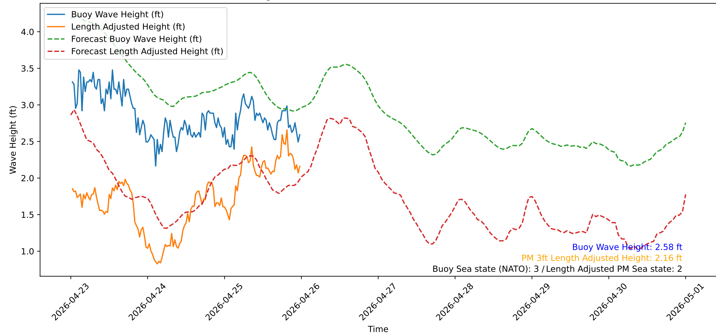
Wave Heights over Time for Red Beach at 2026-04-26 00:20:51
