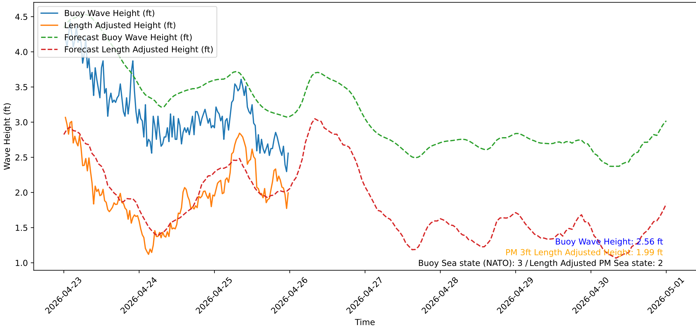
Wave Heights over Time for Oceanside Harbor at 2026-04-26 00:20:31
