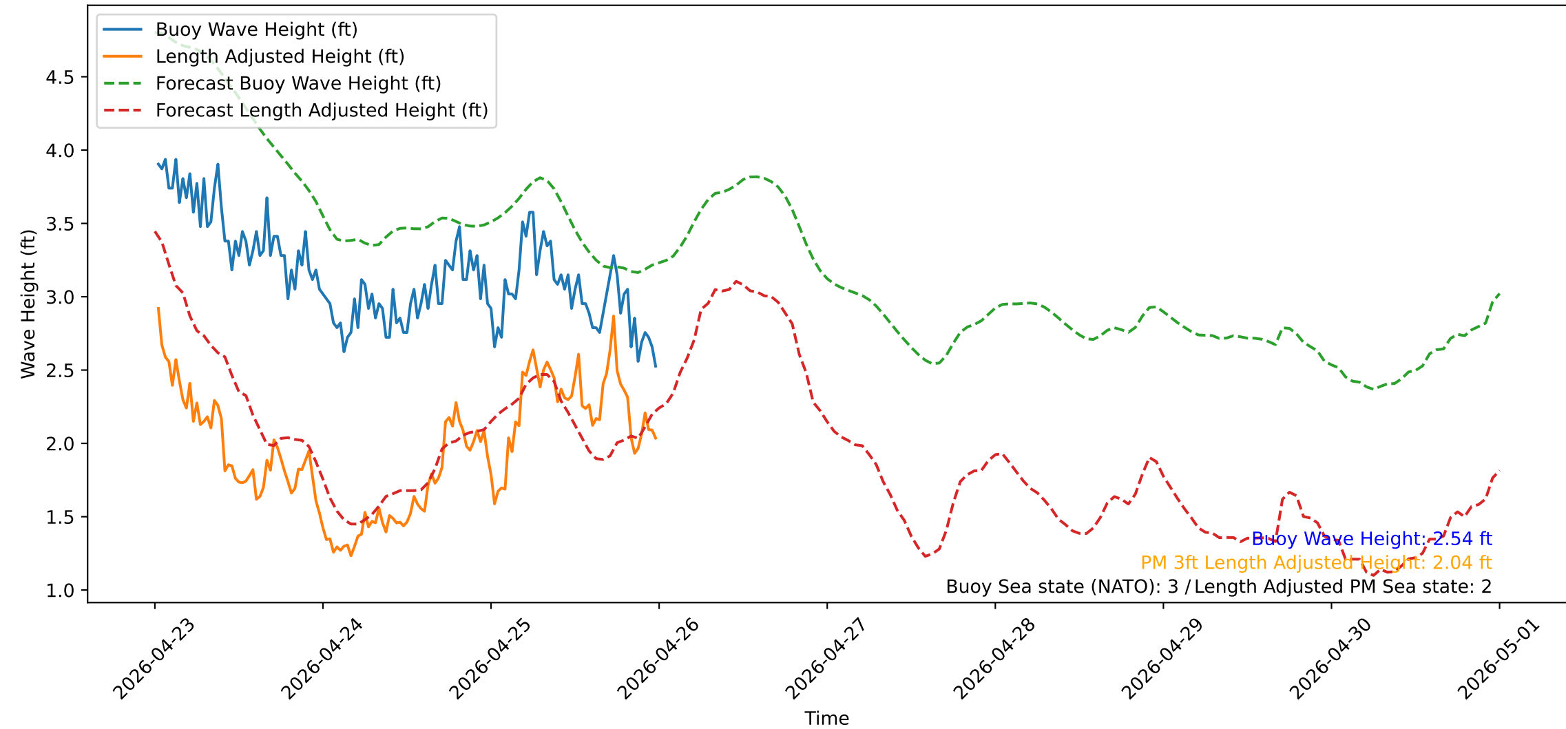
Wave Heights over Time for Green Beach at 2026-04-26 00:21:13
