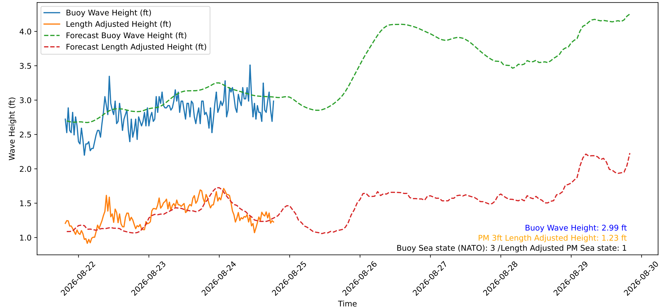
Wave Heights over Time for Oceanside Harbor at 2026-08-24 19:30:30
