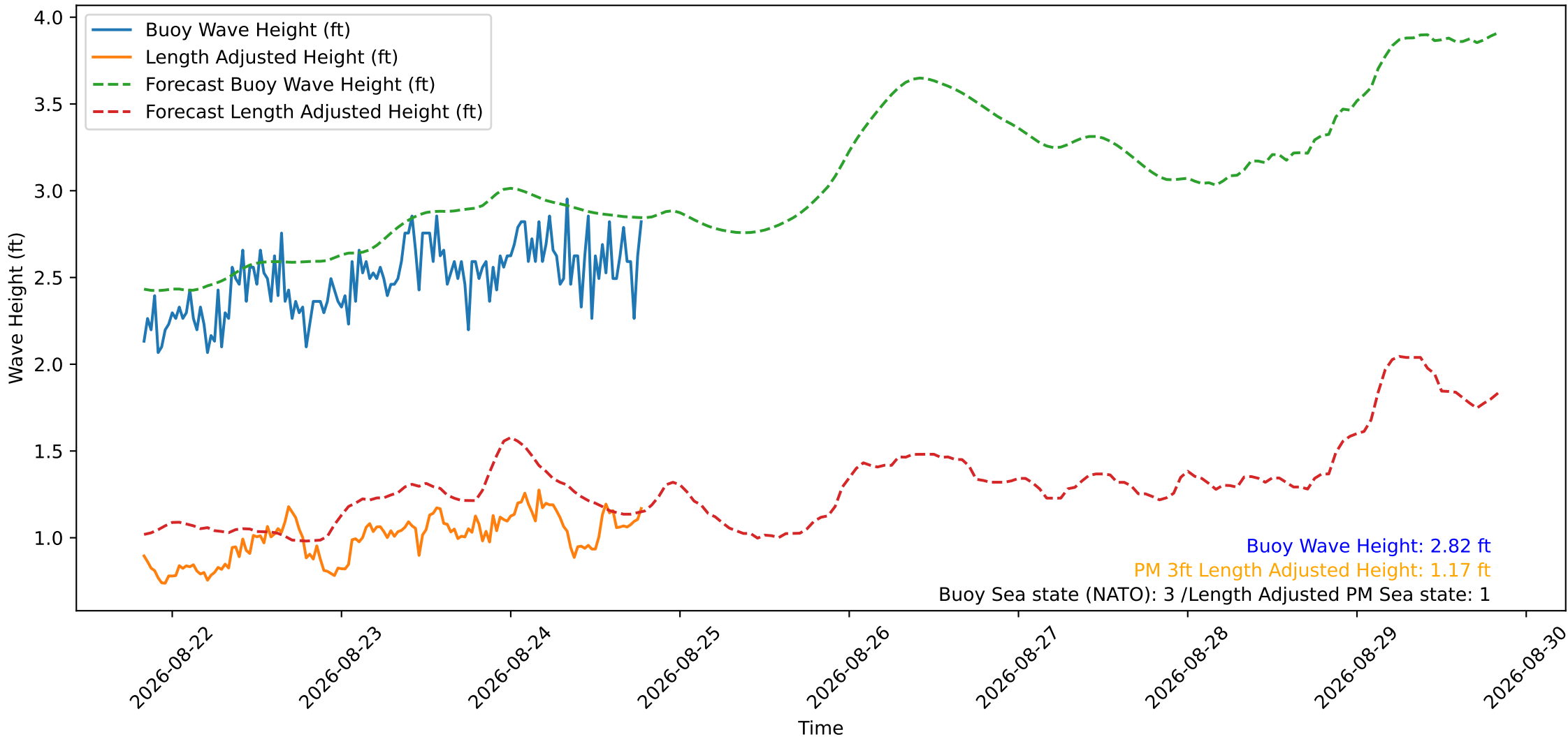
Wave Heights over Time for Red Beach at 2026-08-24 19:30:50
