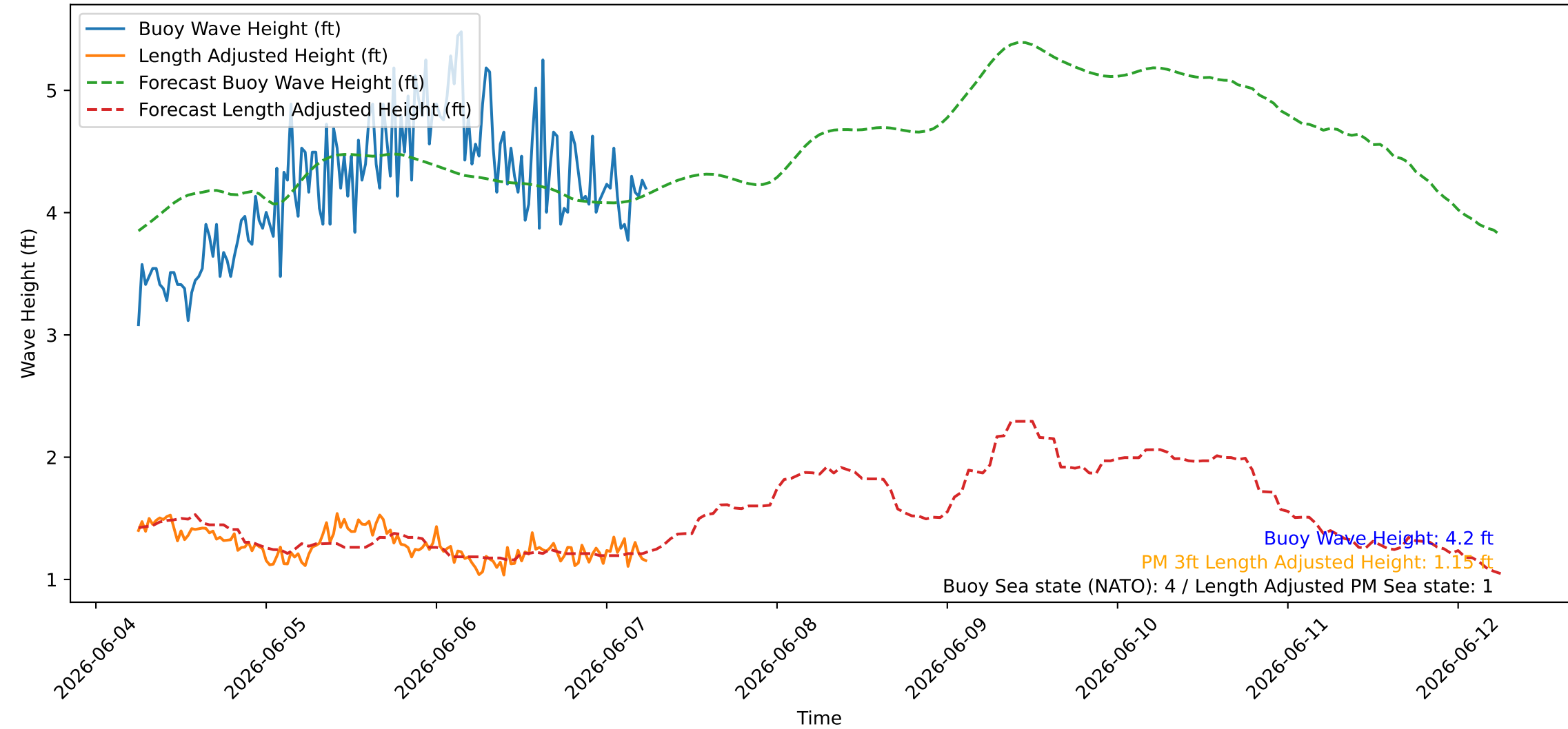
Wave Heights over Time for Oceanside Harbor at 2026-06-07 06:10:26
