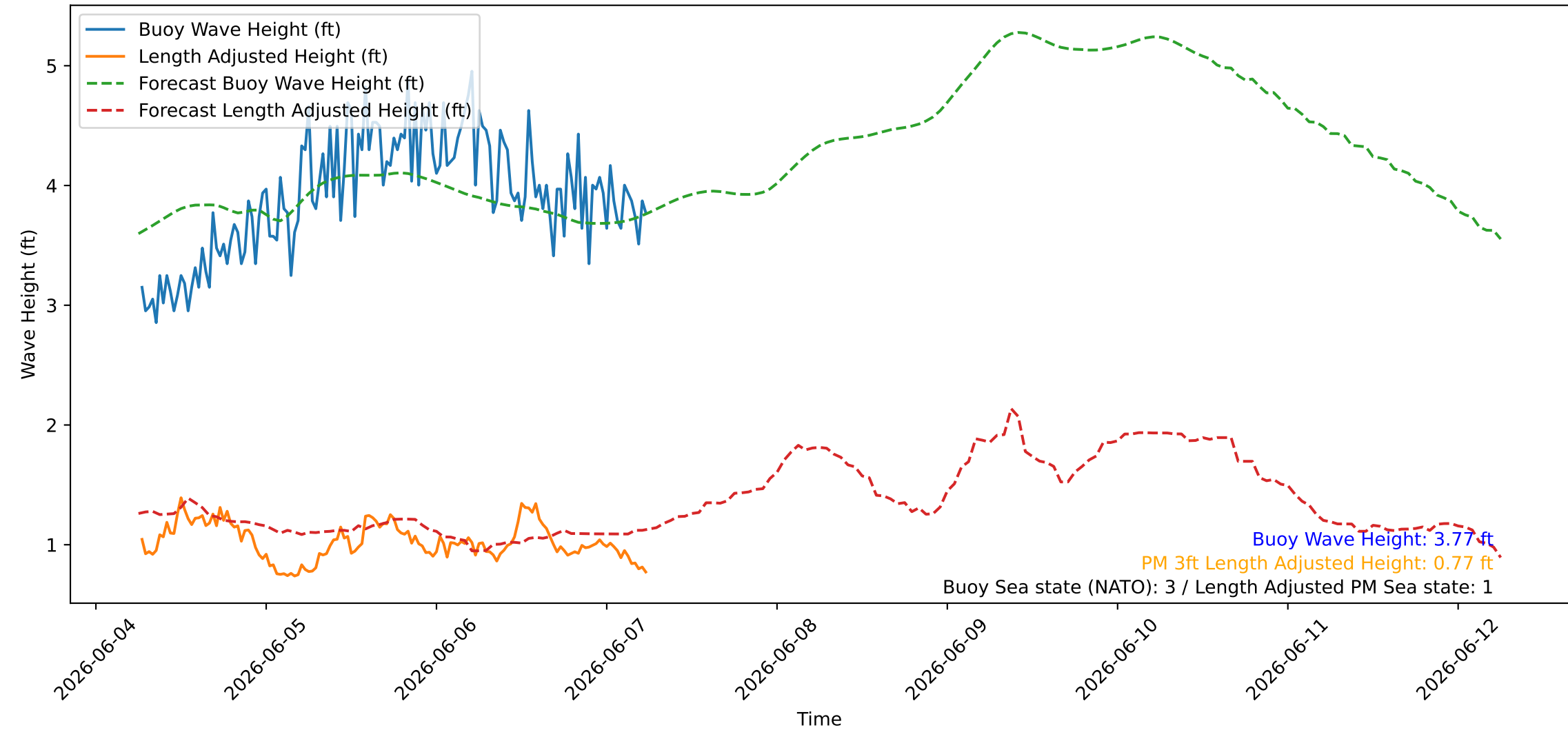
Wave Heights over Time for Red Beach at 2026-06-07 06:10:46
