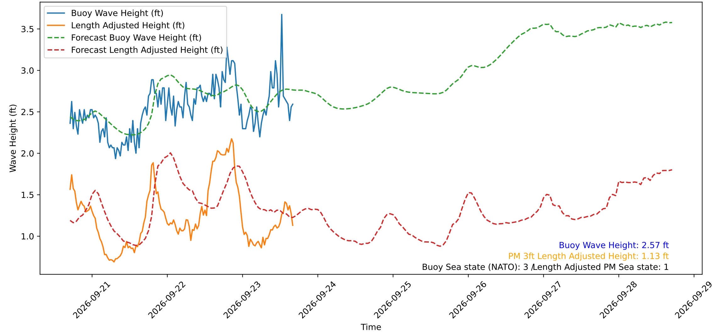
Wave Heights over Time for Red Beach at 2026-09-23 16:40:49
