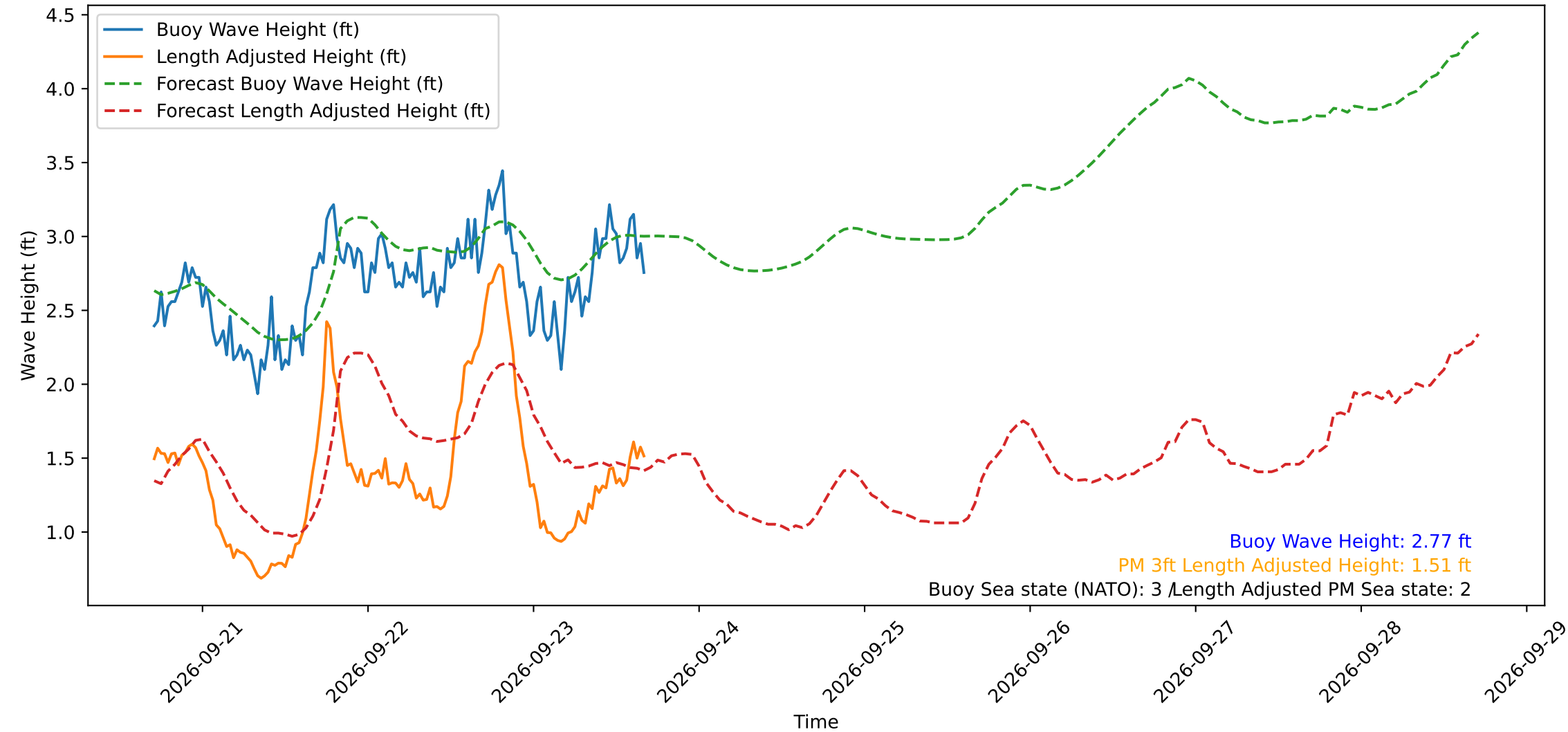
Wave Heights over Time for Green Beach at 2026-09-23 16:41:11
