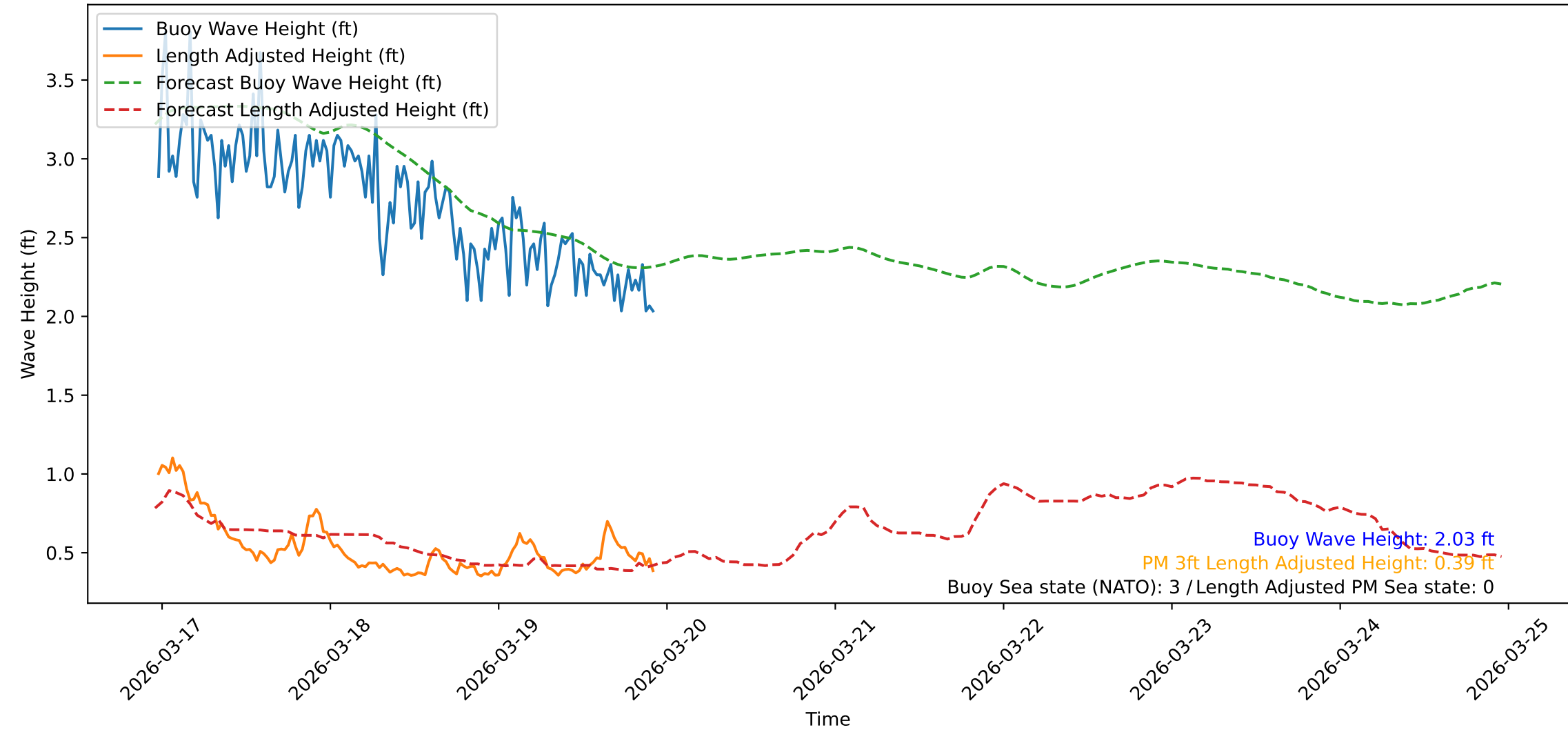
Wave Heights over Time for Red Beach at 2026-03-19 23:00:48
