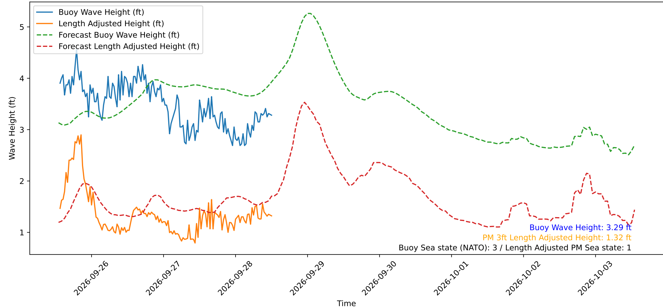
Wave Heights over Time for Green Beach at 2026-09-28 13:01:13
