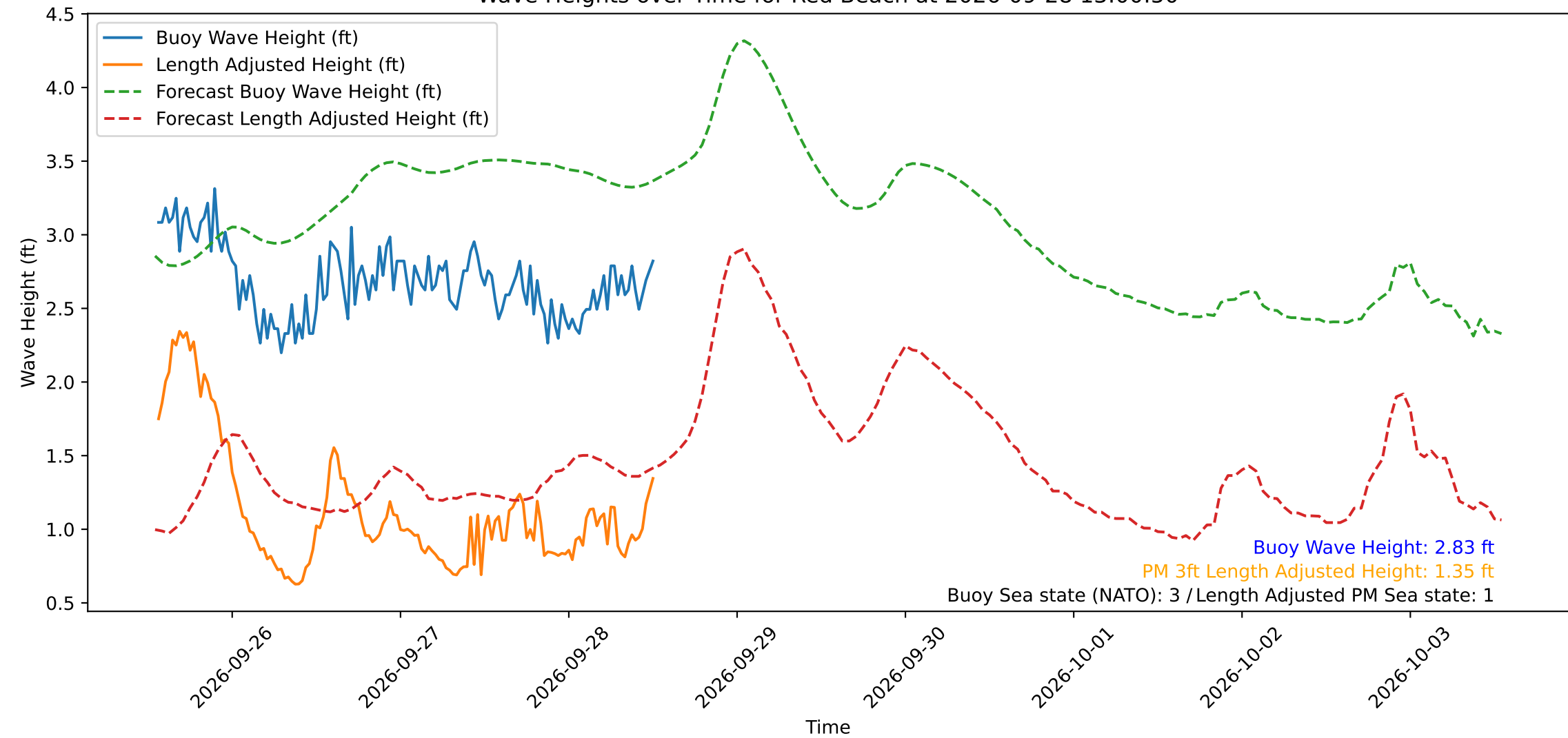
Wave Heights over Time for Red Beach at 2026-09-28 13:00:50
