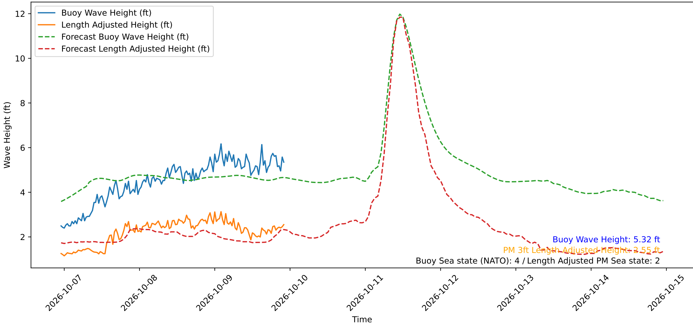
Wave Heights over Time for Green Beach at 2026-10-09 22:51:13
