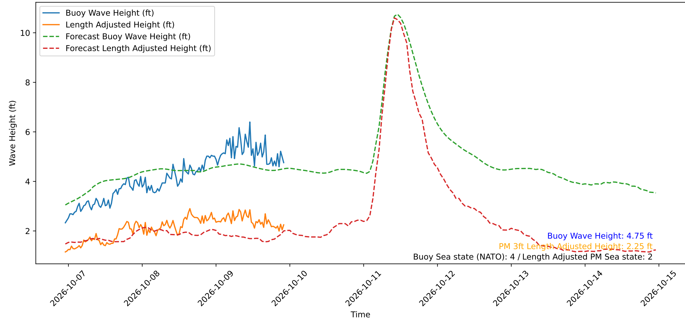
Wave Heights over Time for Oceanside Harbor at 2026-10-09 22:50:29
