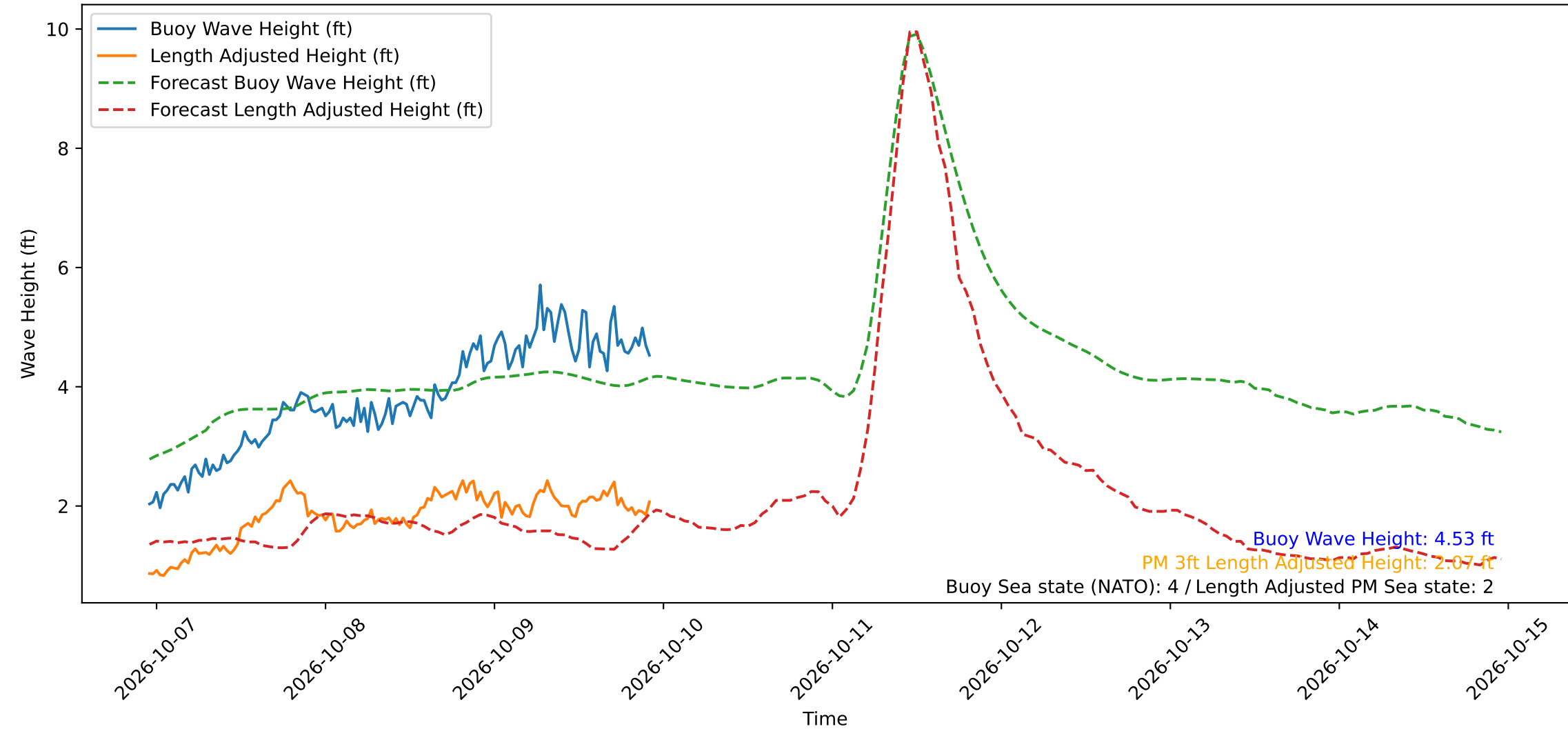
Wave Heights over Time for Red Beach at 2026-10-09 22:50:49
