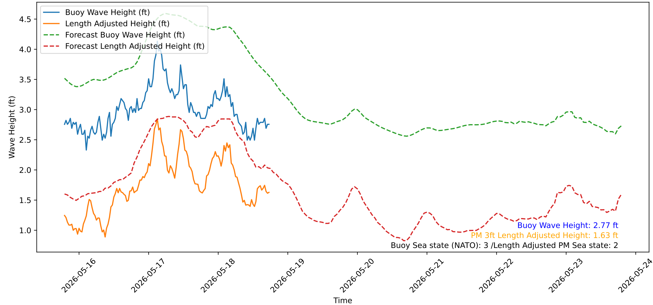
Wave Heights over Time for Red Beach at 2026-05-18 18:30:51
