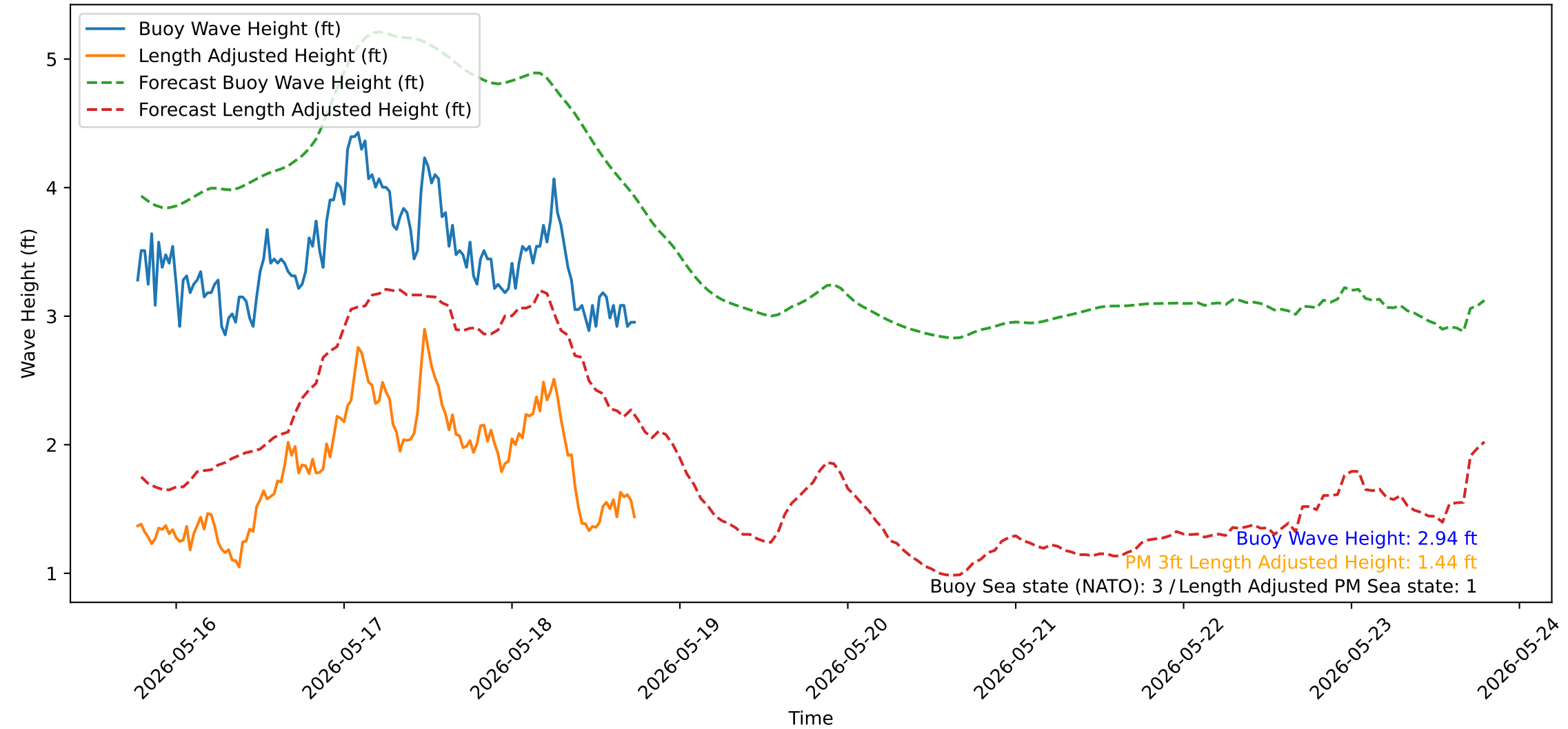
Wave Heights over Time for Green Beach at 2026-05-18 18:31:14
