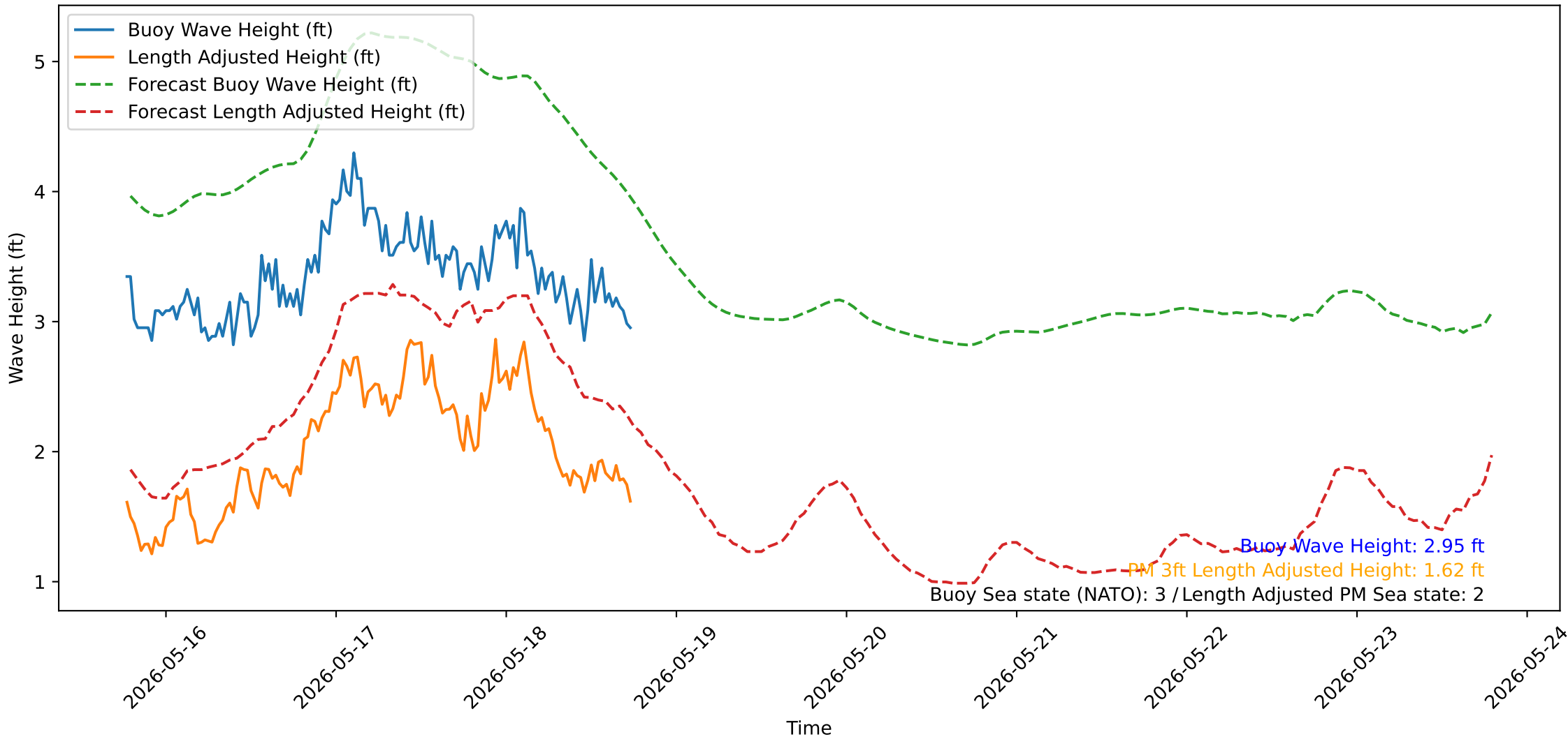
Wave Heights over Time for Oceanside Harbor at 2026-05-18 18:30:32
