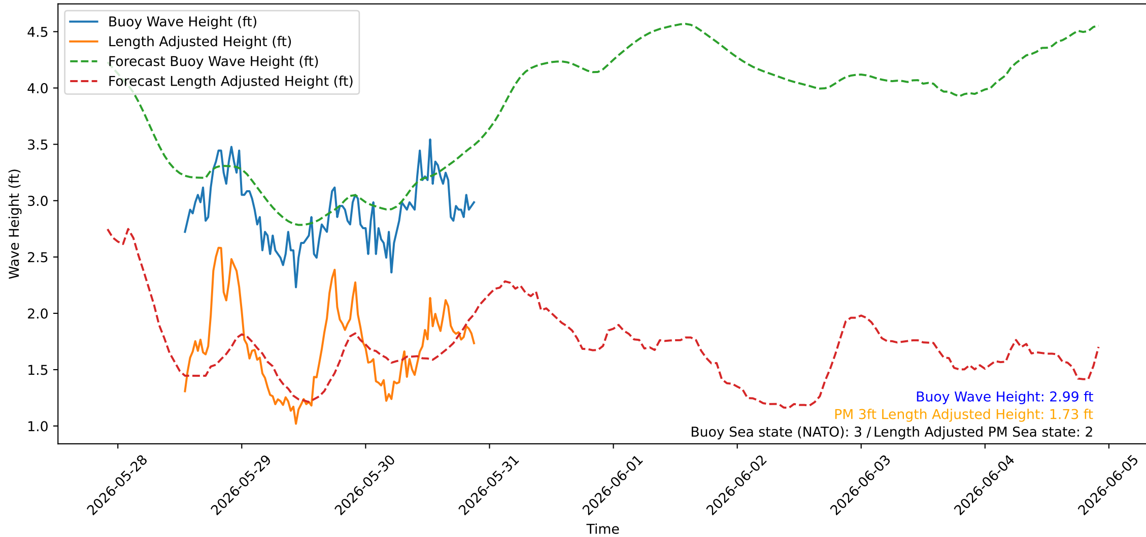
Wave Heights over Time for Oceanside Harbor at 2026-05-30 21:40:24
