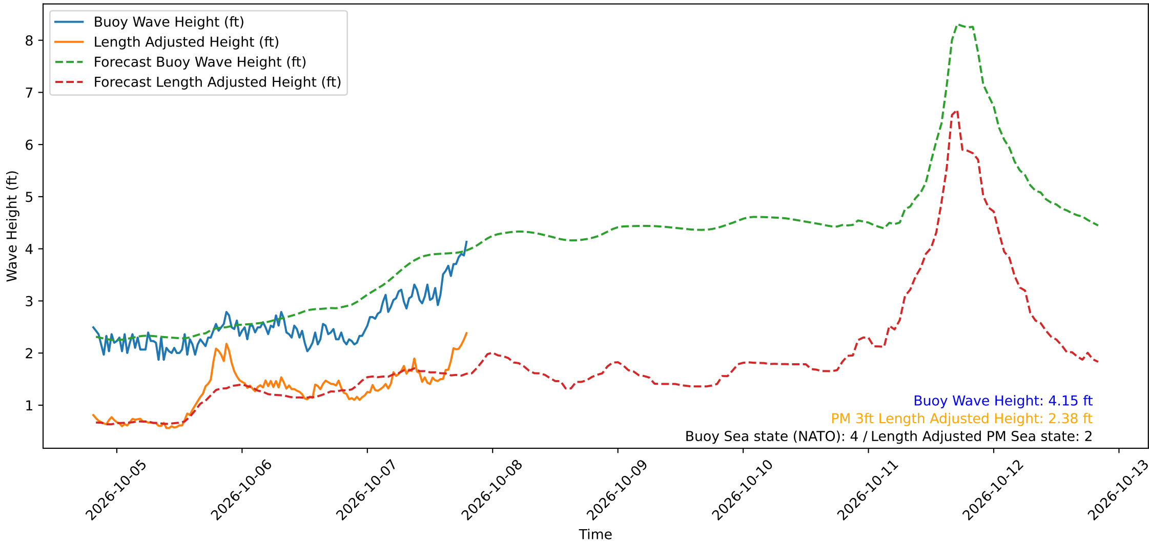
Wave Heights over Time for Oceanside Harbor at 2026-10-07 19:40:29
