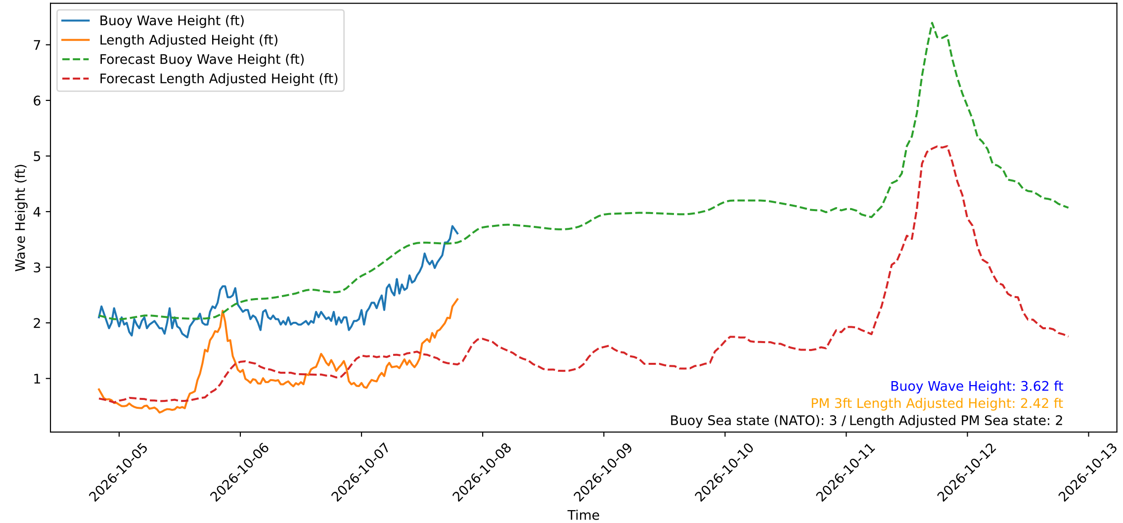
Wave Heights over Time for Red Beach at 2026-10-07 19:40:49
