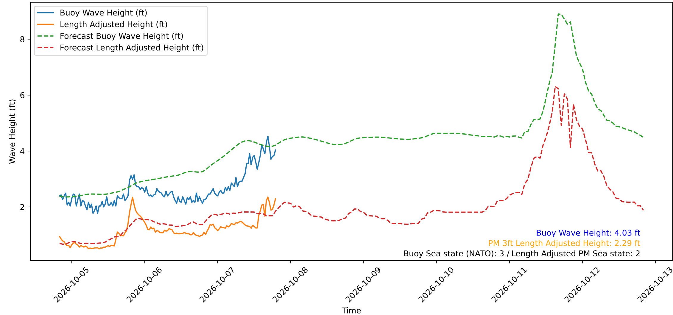
Wave Heights over Time for Green Beach at 2026-10-07 19:41:12
