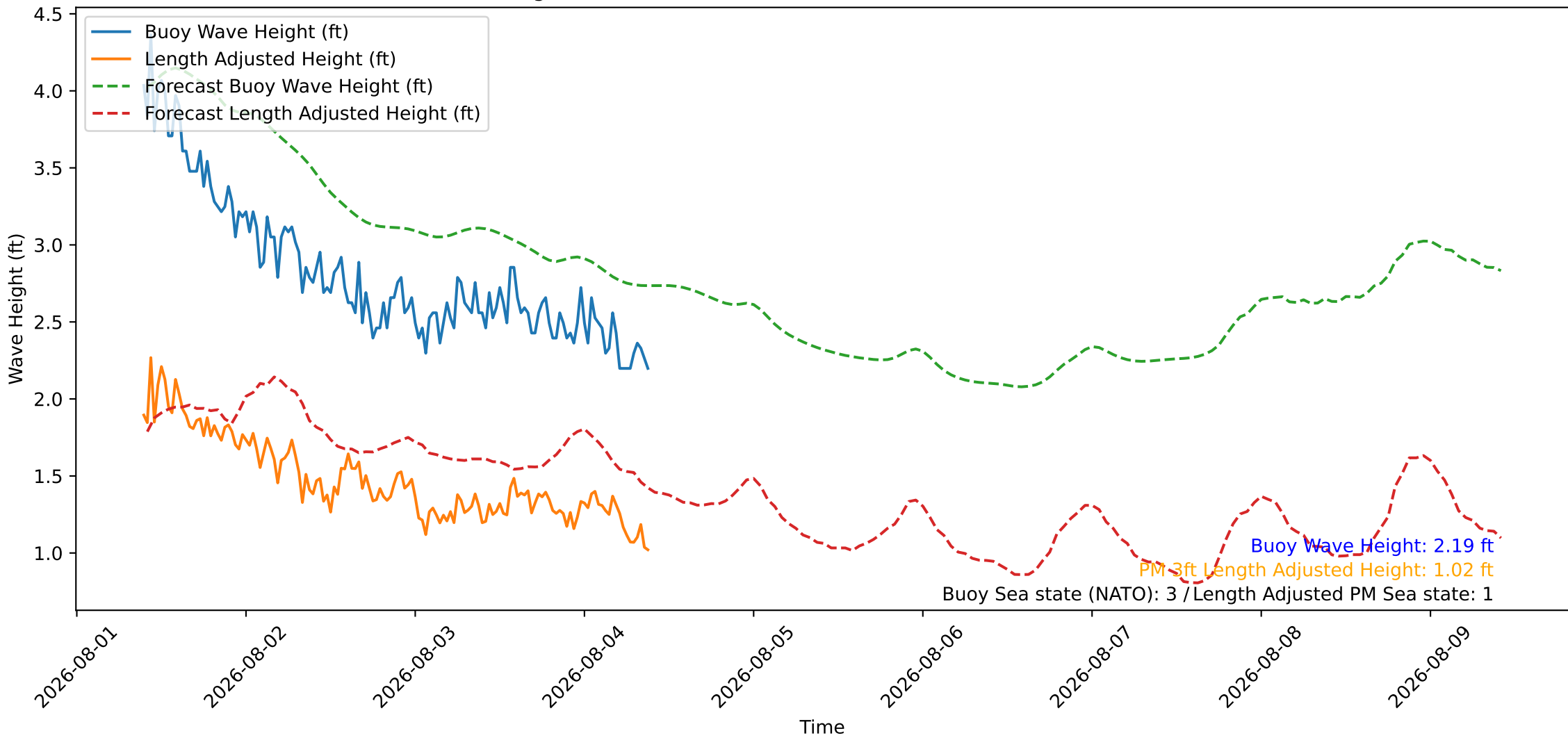
Wave Heights over Time for Oceanside Harbor at 2026-08-04 09:30:27
