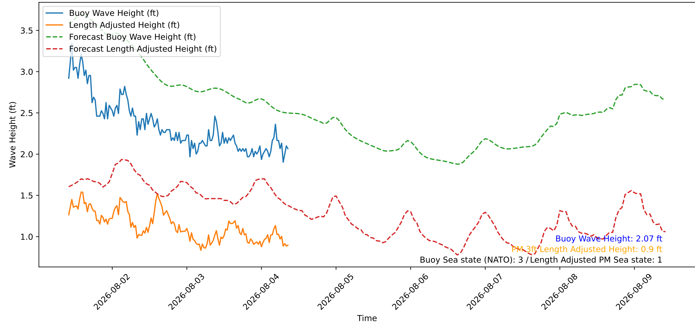
Wave Heights over Time for Red Beach at 2026-08-04 09:30:46
