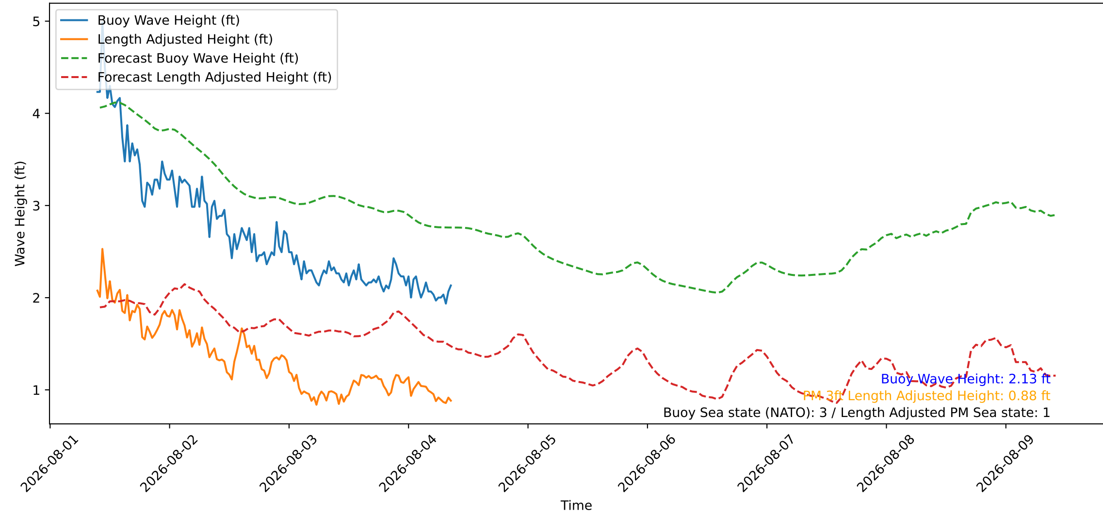
Wave Heights over Time for Green Beach at 2026-08-04 09:31:08
