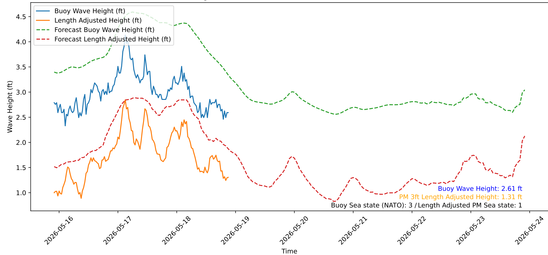
Wave Heights over Time for Red Beach at 2026-05-18 21:50:53
