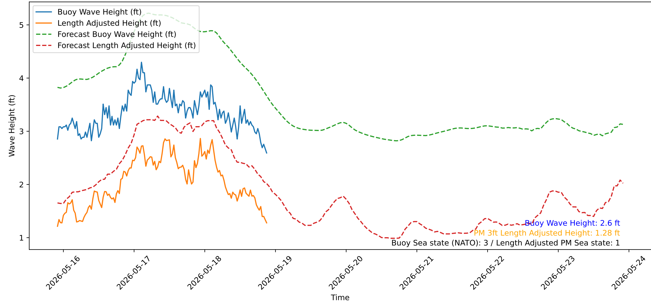
Wave Heights over Time for Oceanside Harbor at 2026-05-18 21:50:32
