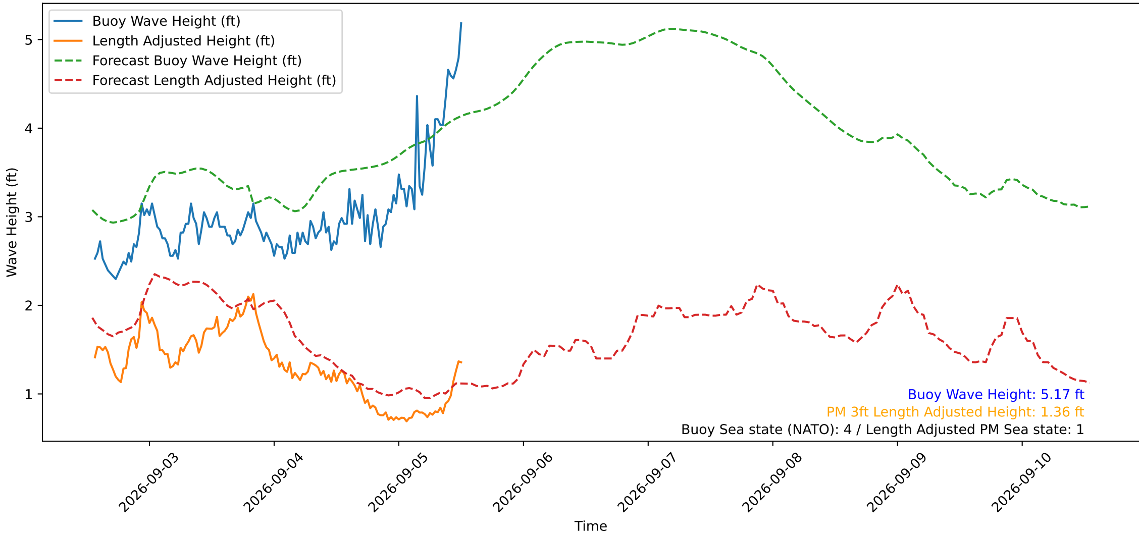
Wave Heights over Time for Red Beach at 2026-09-05 13:00:51
