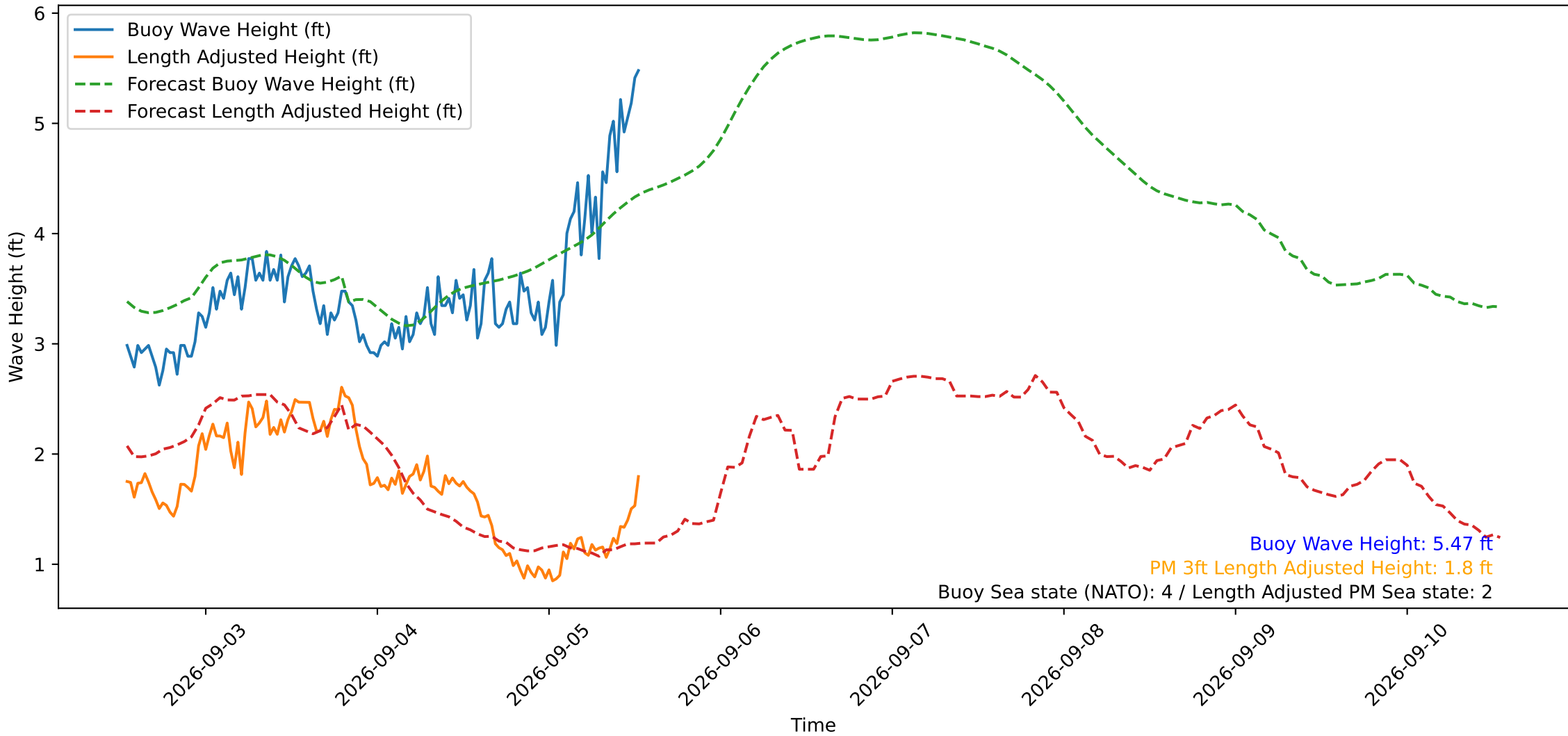
Wave Heights over Time for Oceanside Harbor at 2026-09-05 13:00:31
