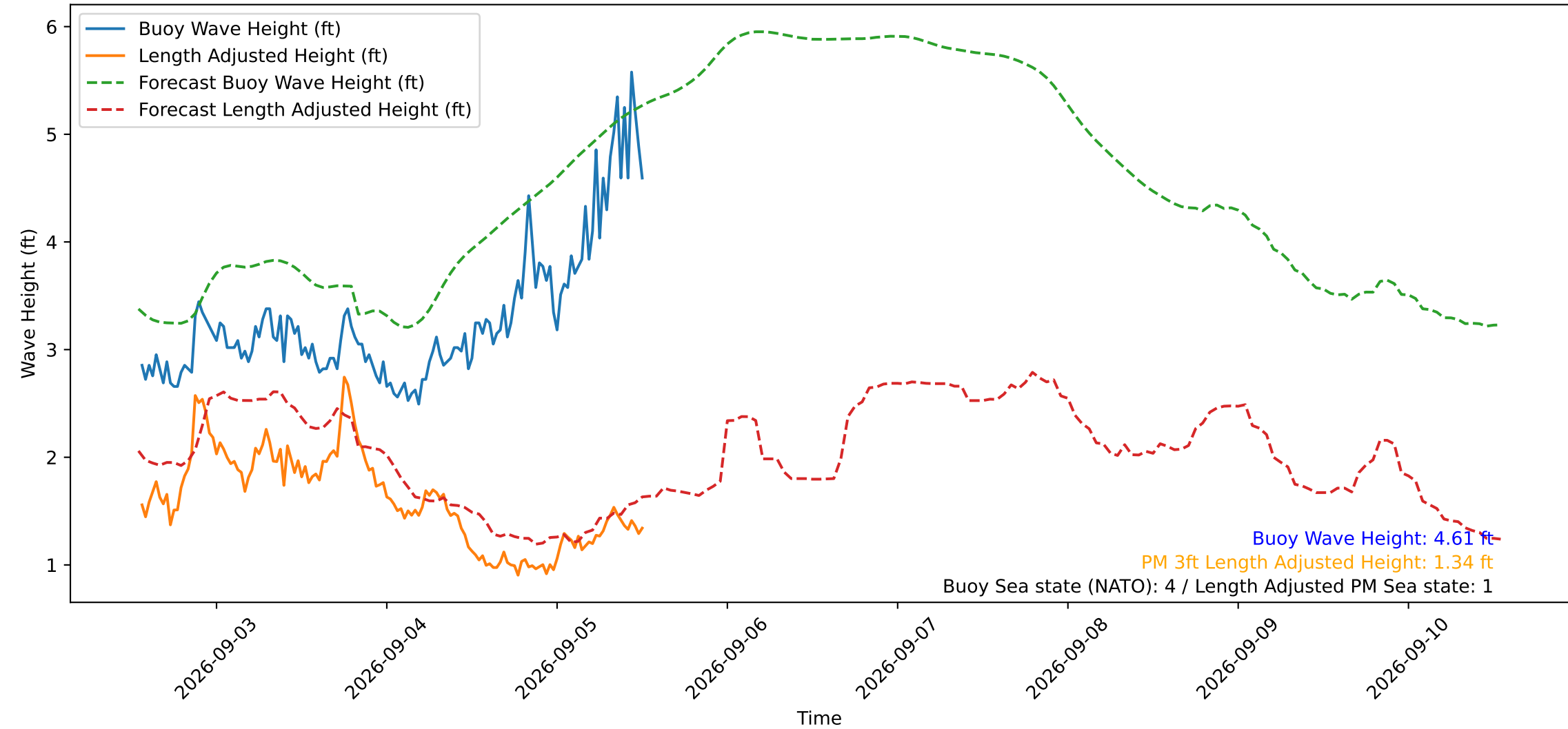
Wave Heights over Time for Green Beach at 2026-09-05 13:01:13
