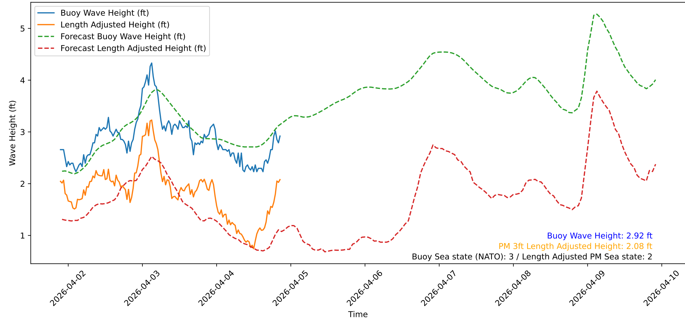
Wave Heights over Time for Green Beach at 2026-04-04 21:31:24
