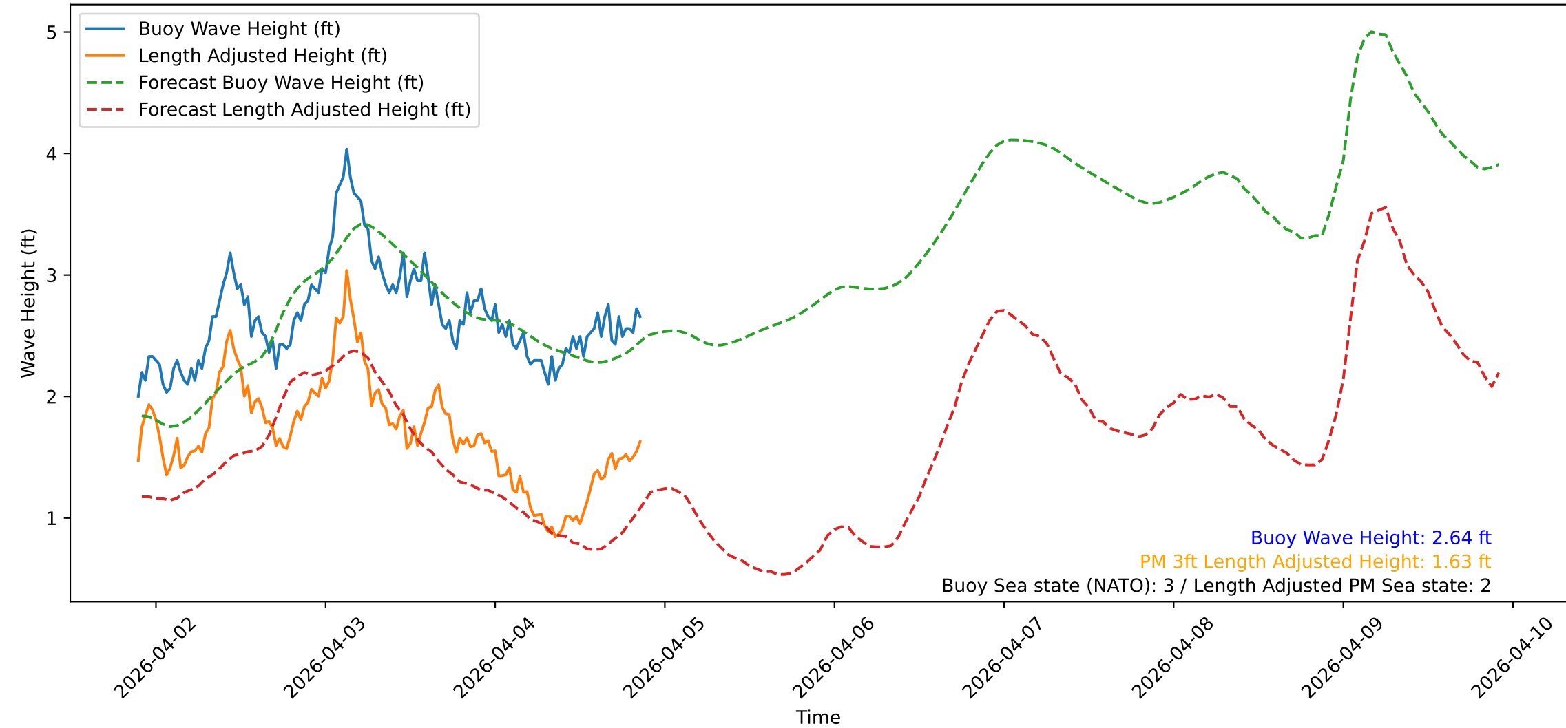
Wave Heights over Time for Oceanside Harbor at 2026-04-04 21:30:37
