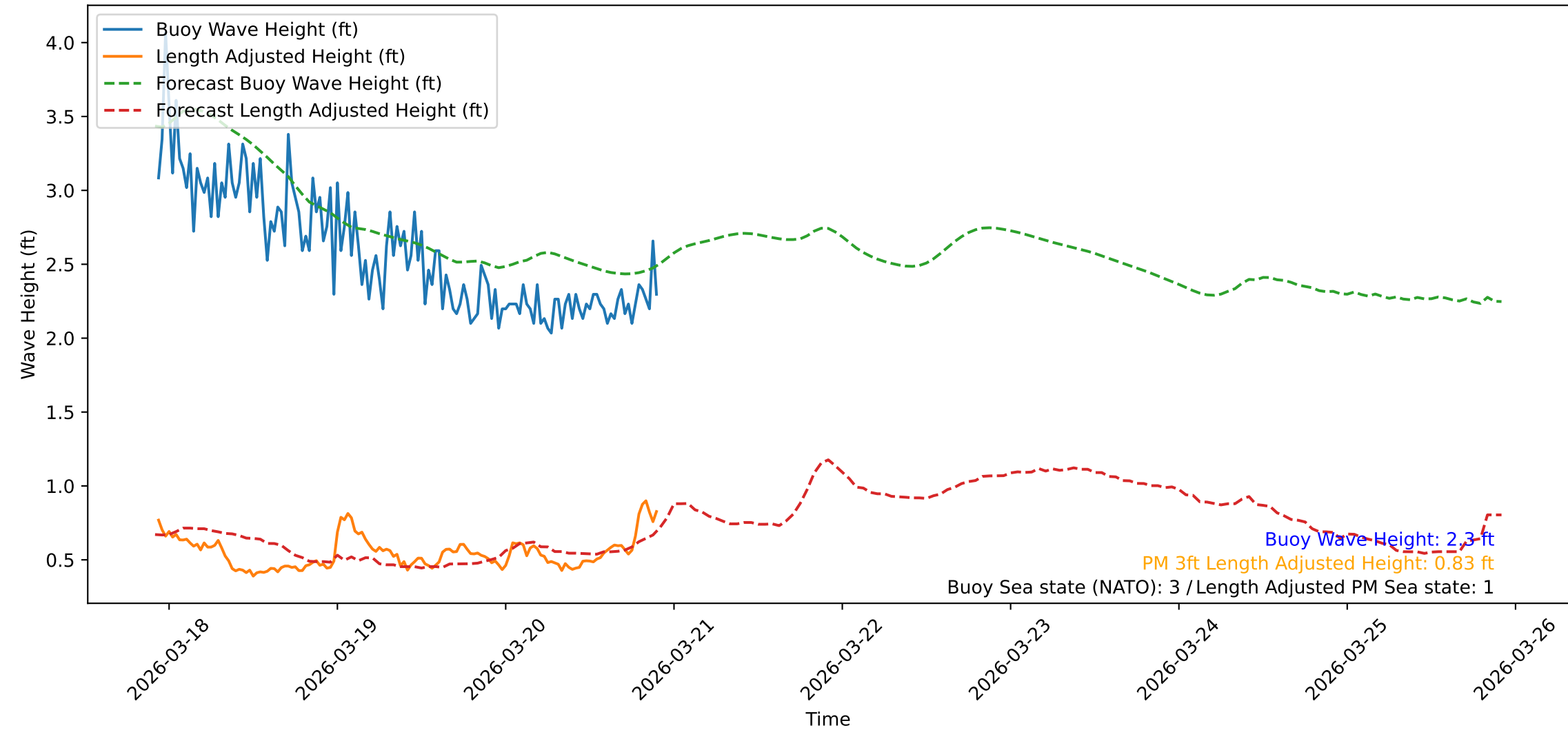
Wave Heights over Time for Green Beach at 2026-03-20 22:21:10
