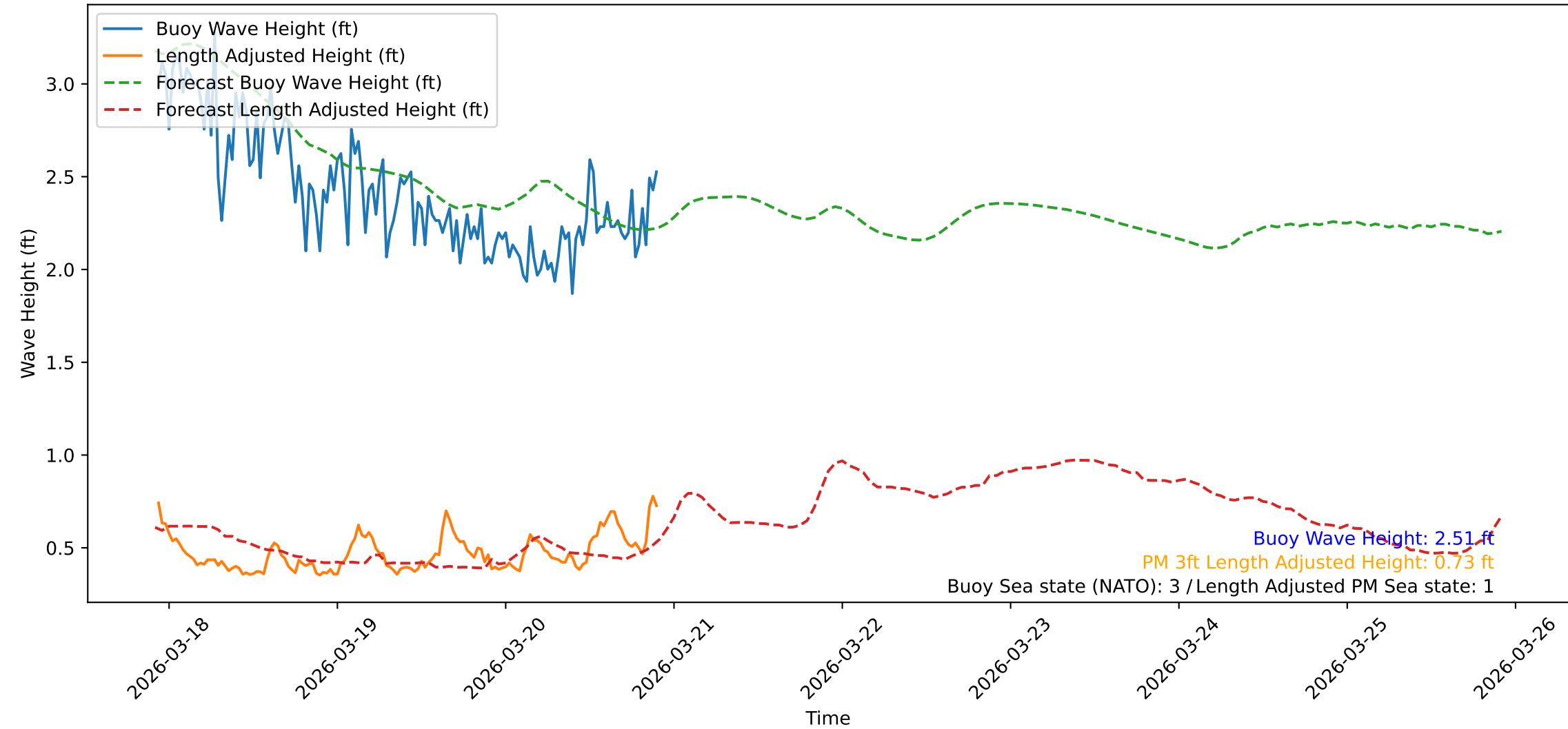
Wave Heights over Time for Red Beach at 2026-03-20 22:20:47
