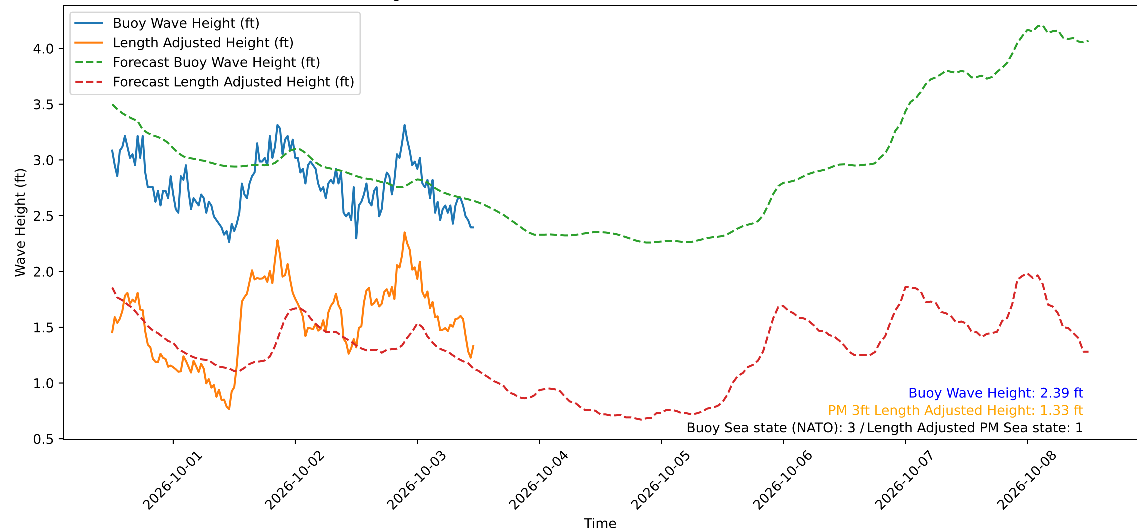
Wave Heights over Time for Oceanside Harbor at 2026-10-03 11:50:29
