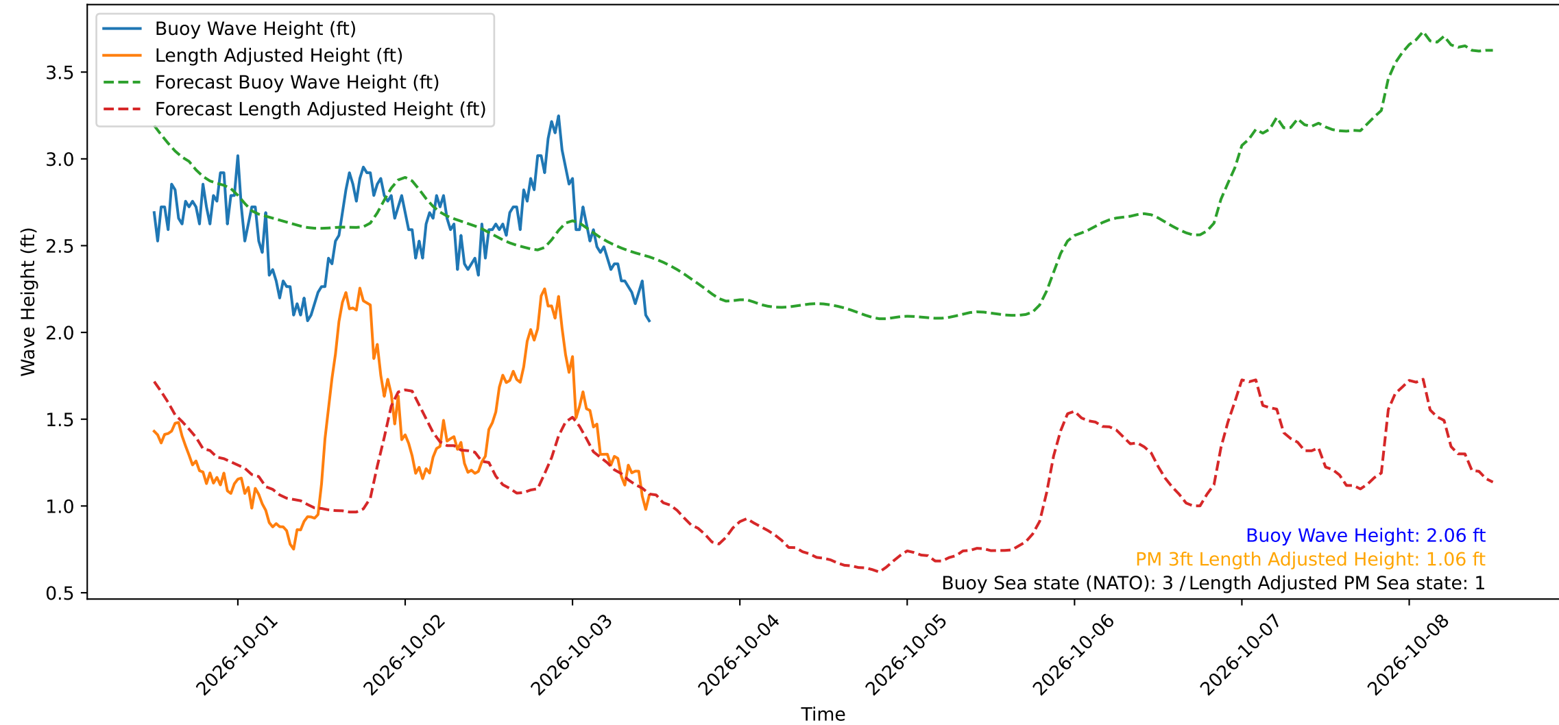
Wave Heights over Time for Red Beach at 2026-10-03 11:50:51
