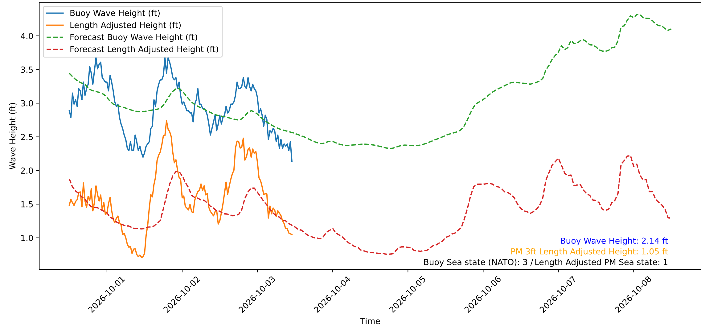
Wave Heights over Time for Green Beach at 2026-10-03 11:51:15
