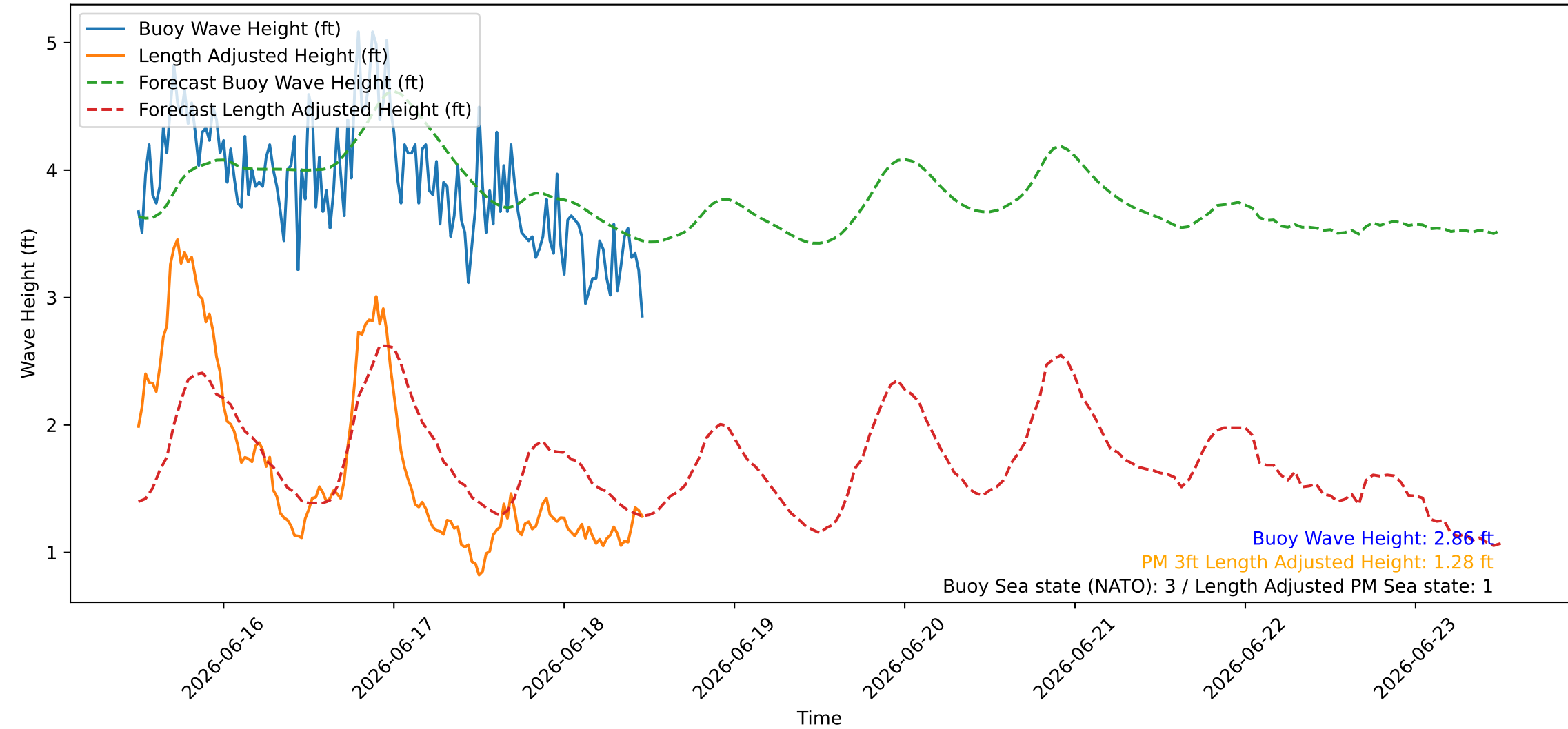
Wave Heights over Time for Green Beach at 2026-06-18 11:51:10
