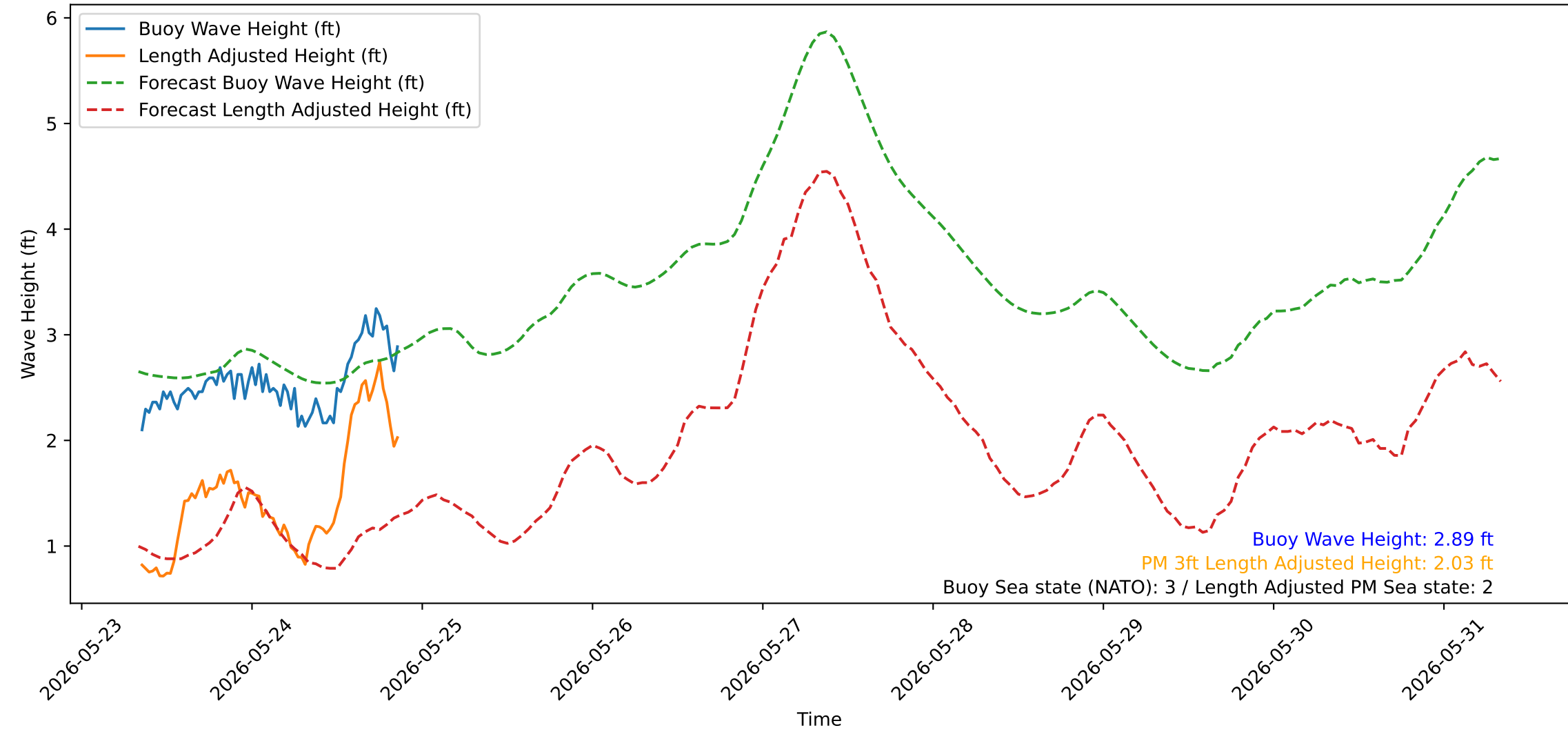
Wave Heights over Time for Oceanside Harbor at 2026-05-26 08:20:29
