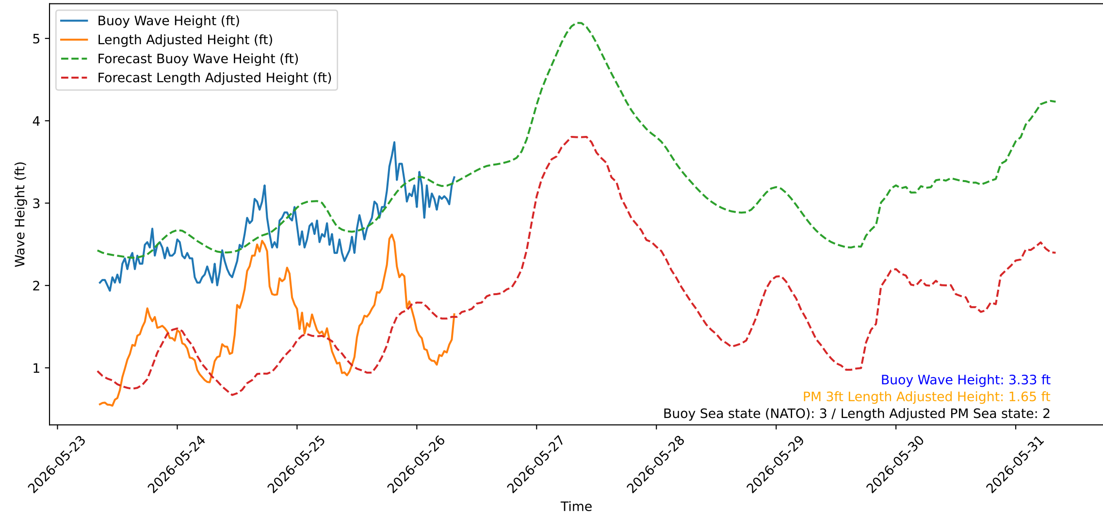
Wave Heights over Time for Red Beach at 2026-05-26 08:20:49
