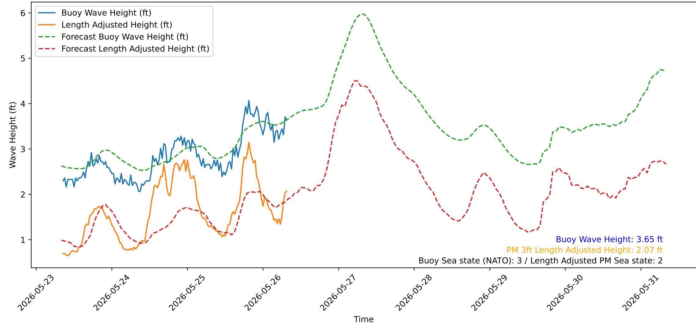
Wave Heights over Time for Green Beach at 2026-05-26 08:21:12
