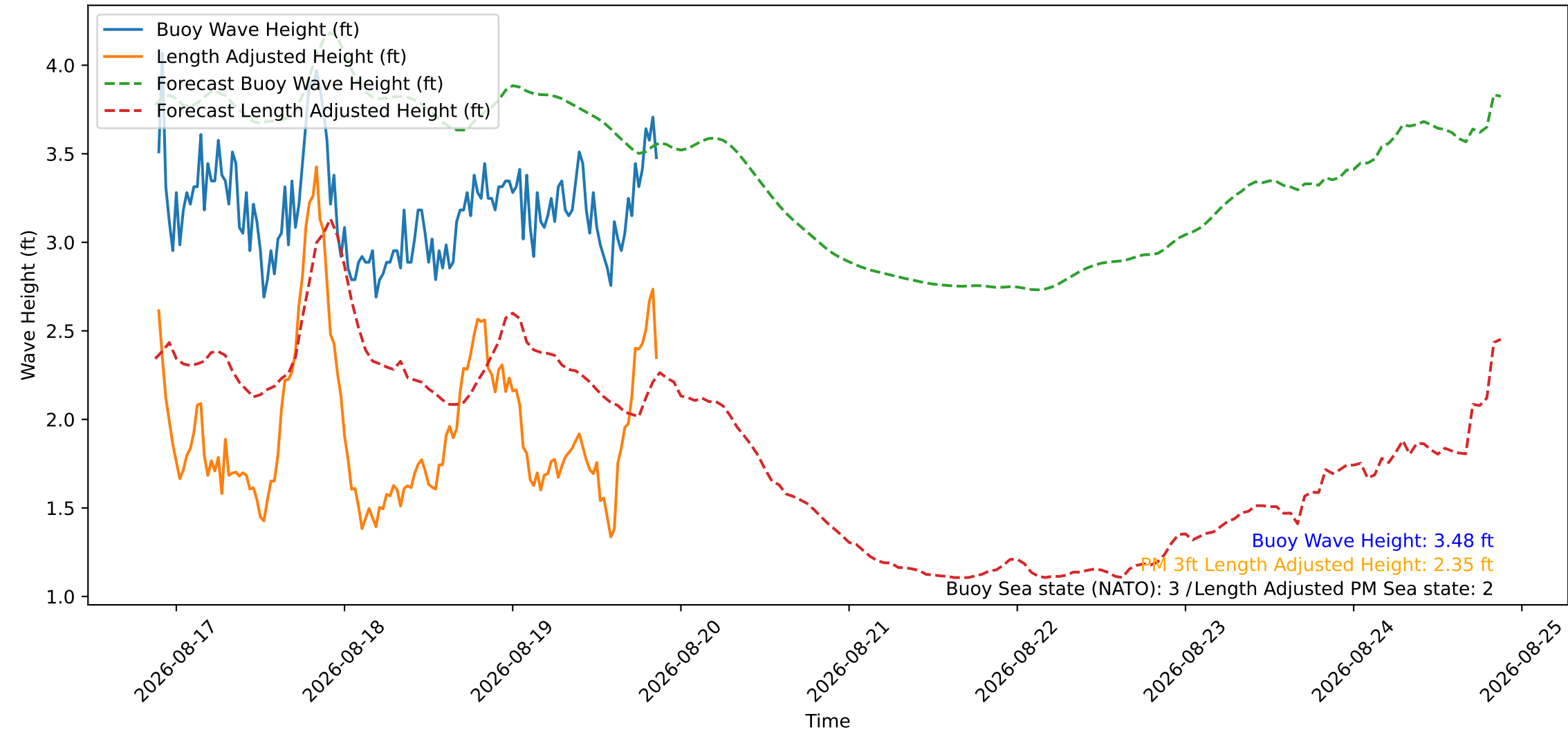
Wave Heights over Time for Green Beach at 2026-08-19 21:21:12
