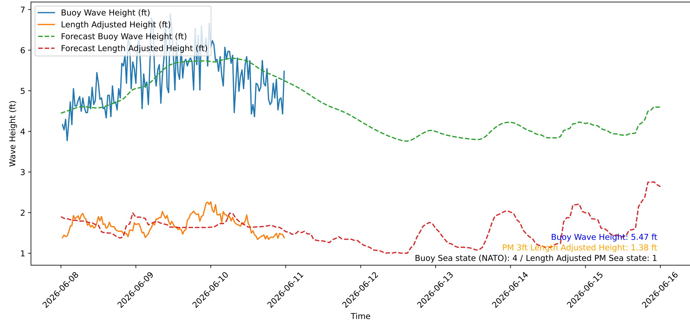
Wave Heights over Time for Green Beach at 2026-06-11 00:21:12
