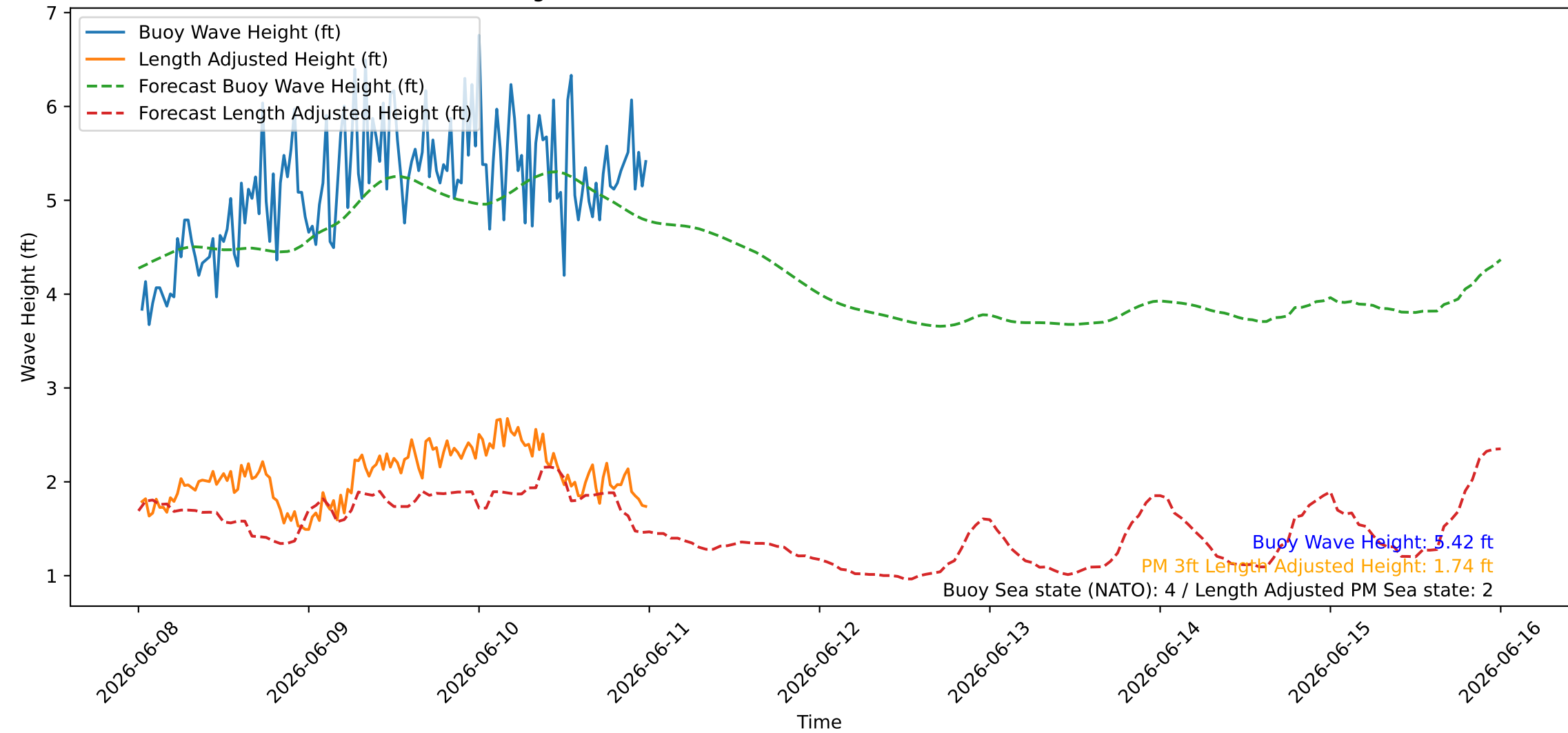
Wave Heights over Time for Oceanside Harbor at 2026-06-11 00:20:26
