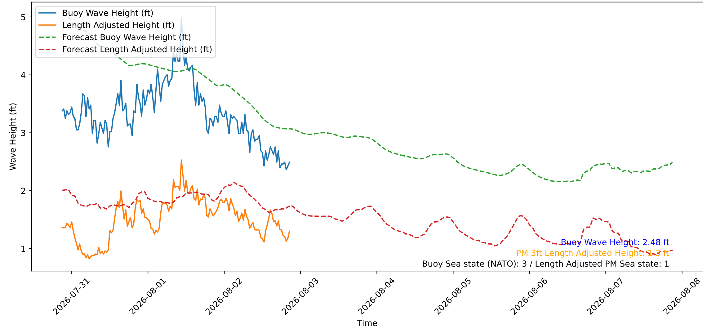
Wave Heights over Time for Green Beach at 2026-08-02 21:11:08
