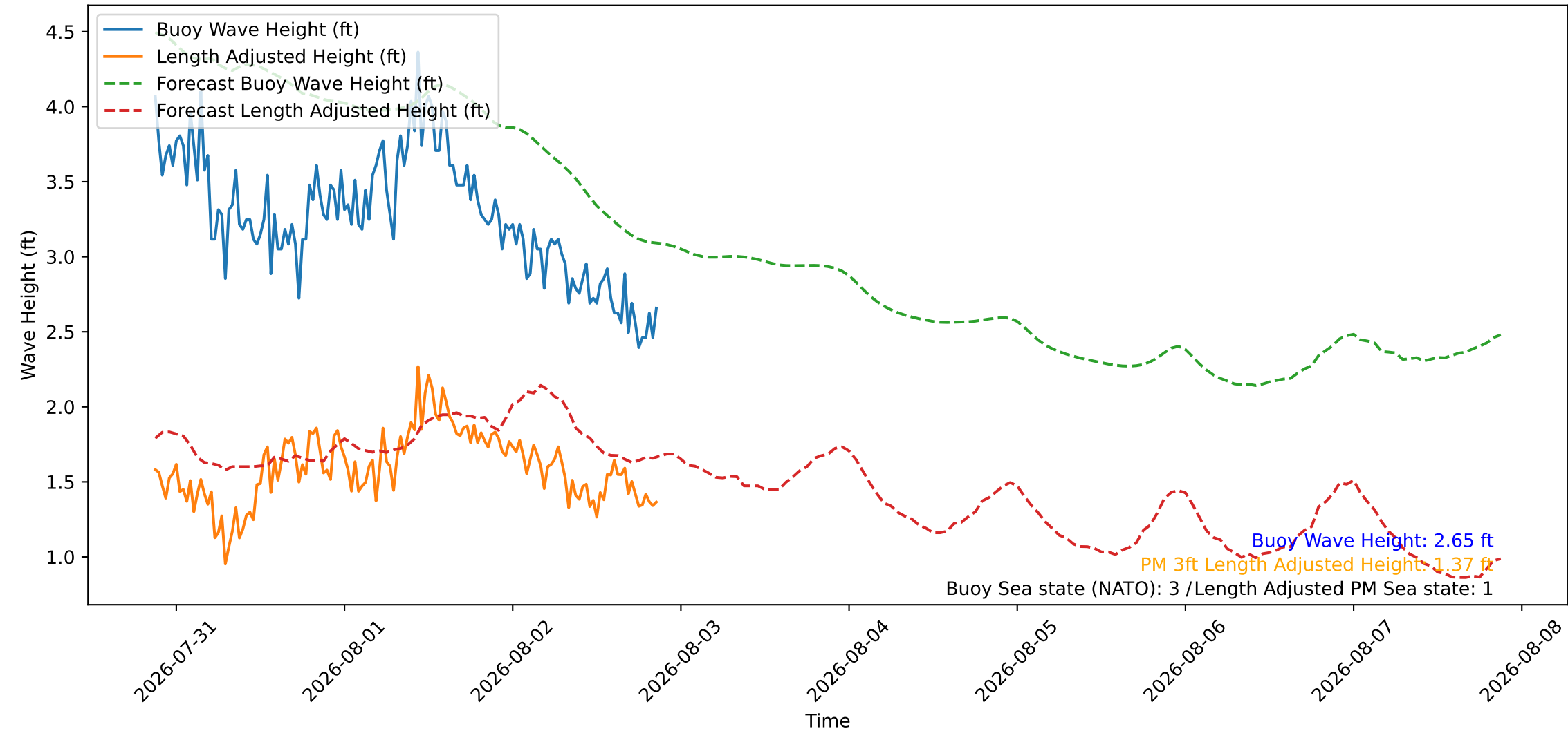
Wave Heights over Time for Oceanside Harbor at 2026-08-02 21:10:26
