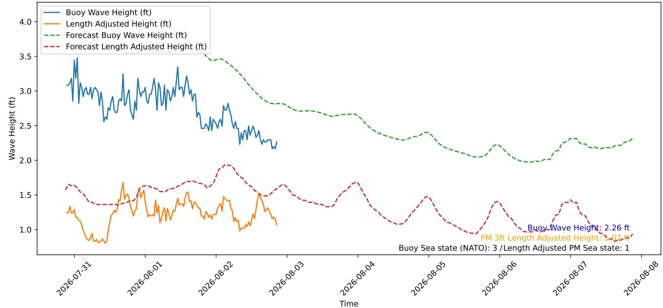
Wave Heights over Time for Red Beach at 2026-08-02 21:10:45
