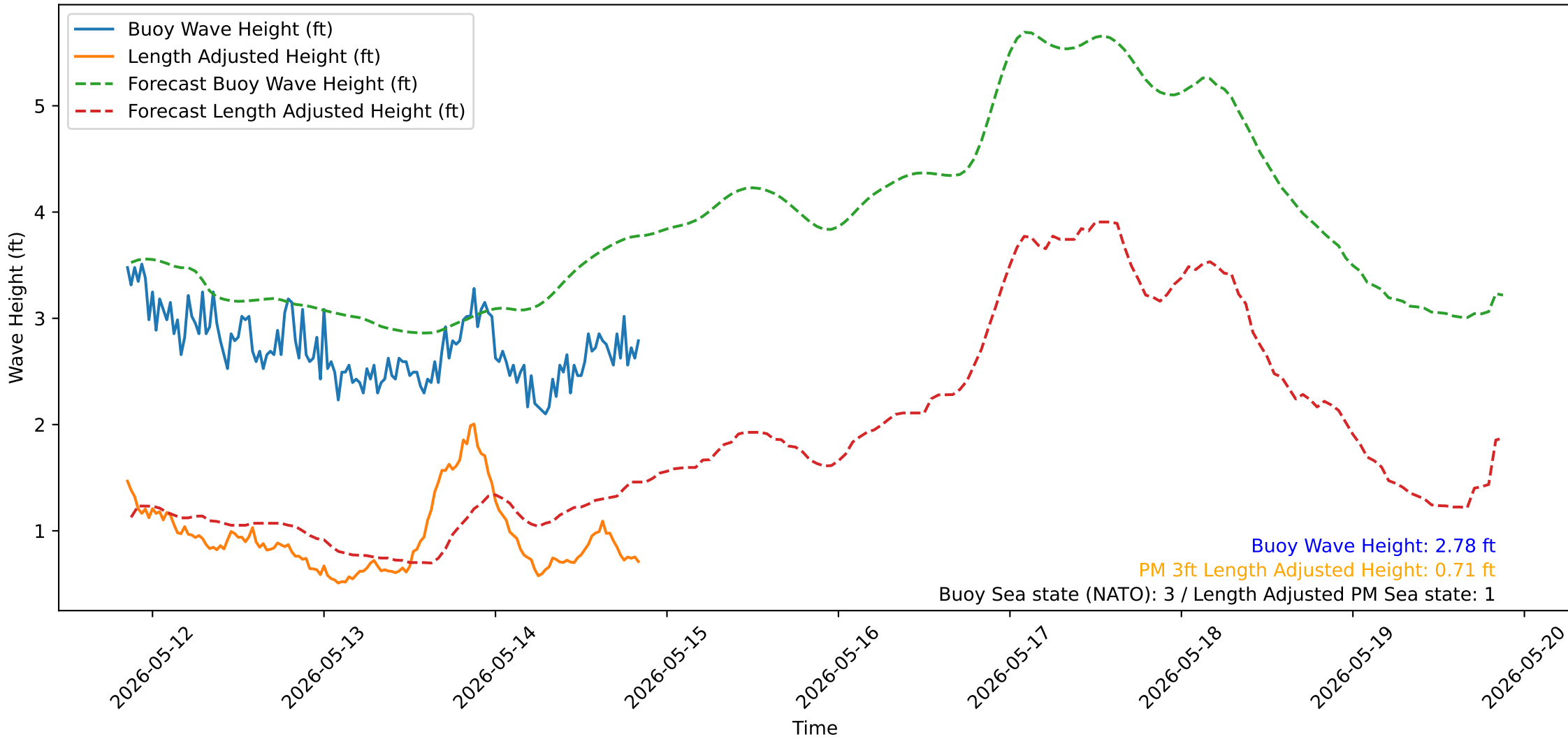
Wave Heights over Time for Green Beach at 2026-05-14 20:41:14
