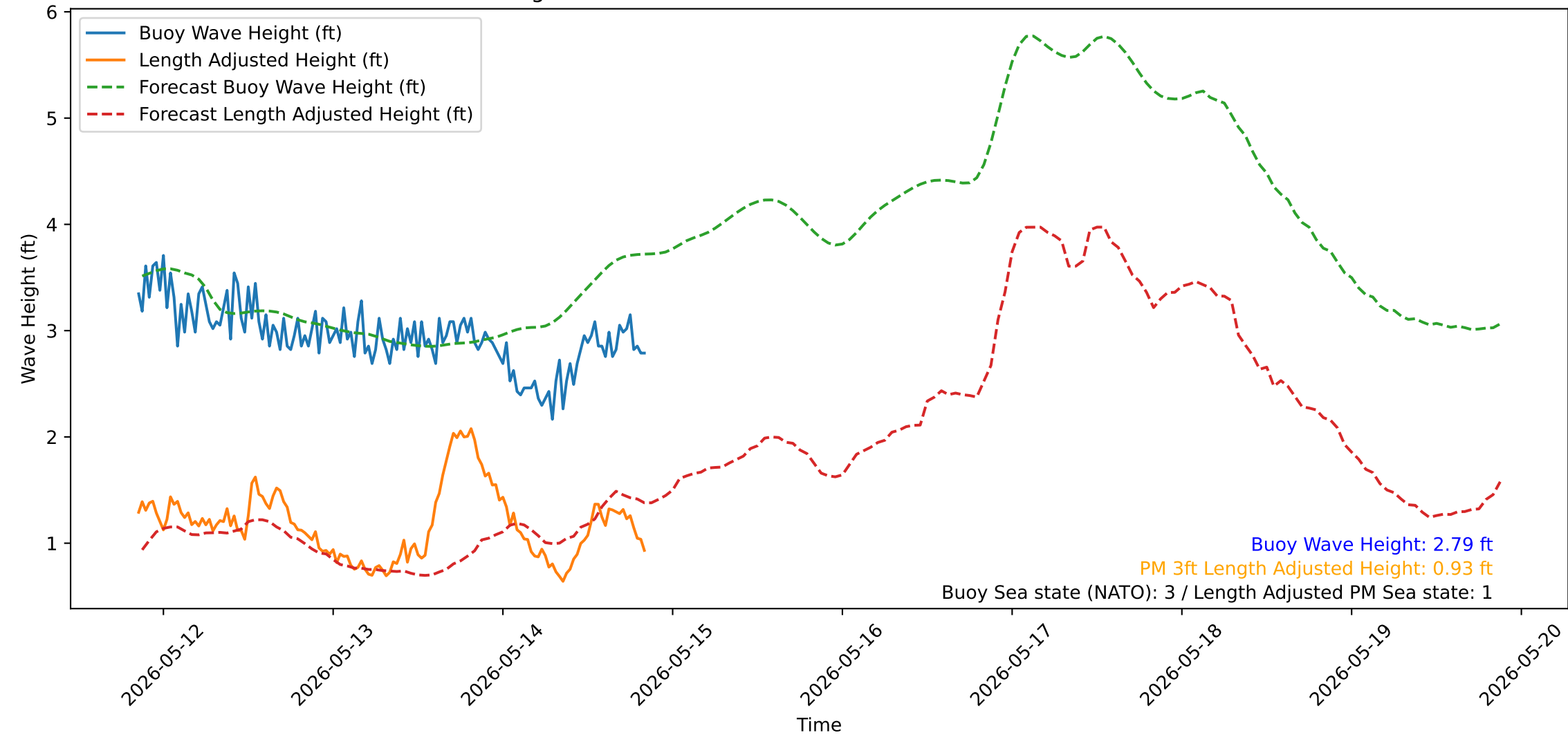
Wave Heights over Time for Oceanside Harbor at 2026-05-14 20:40:32
