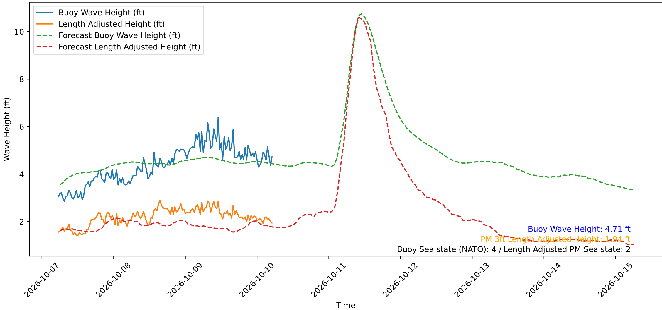
Wave Heights over Time for Oceanside Harbor at 2026-10-10 05:40:30
