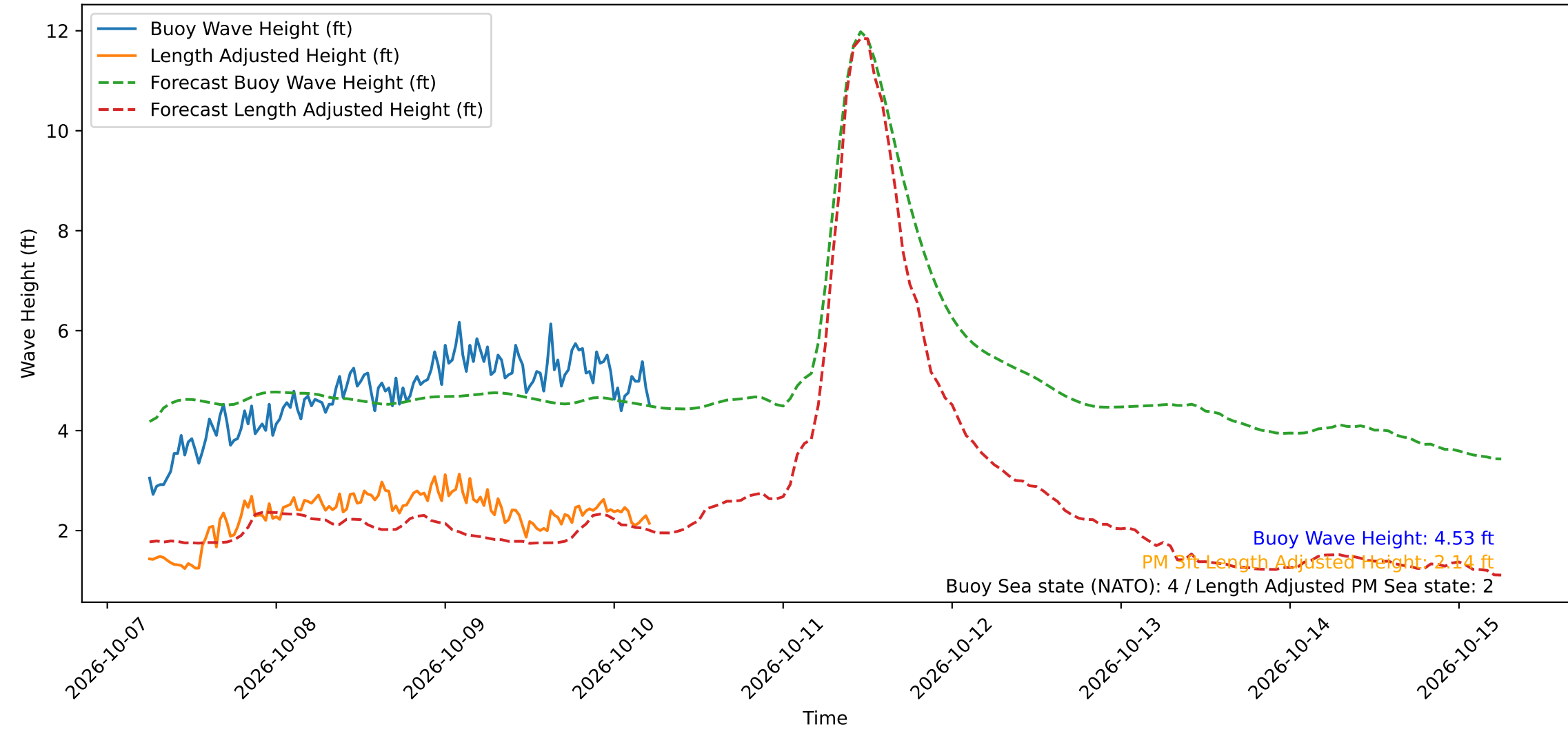
Wave Heights over Time for Green Beach at 2026-10-10 05:41:12
