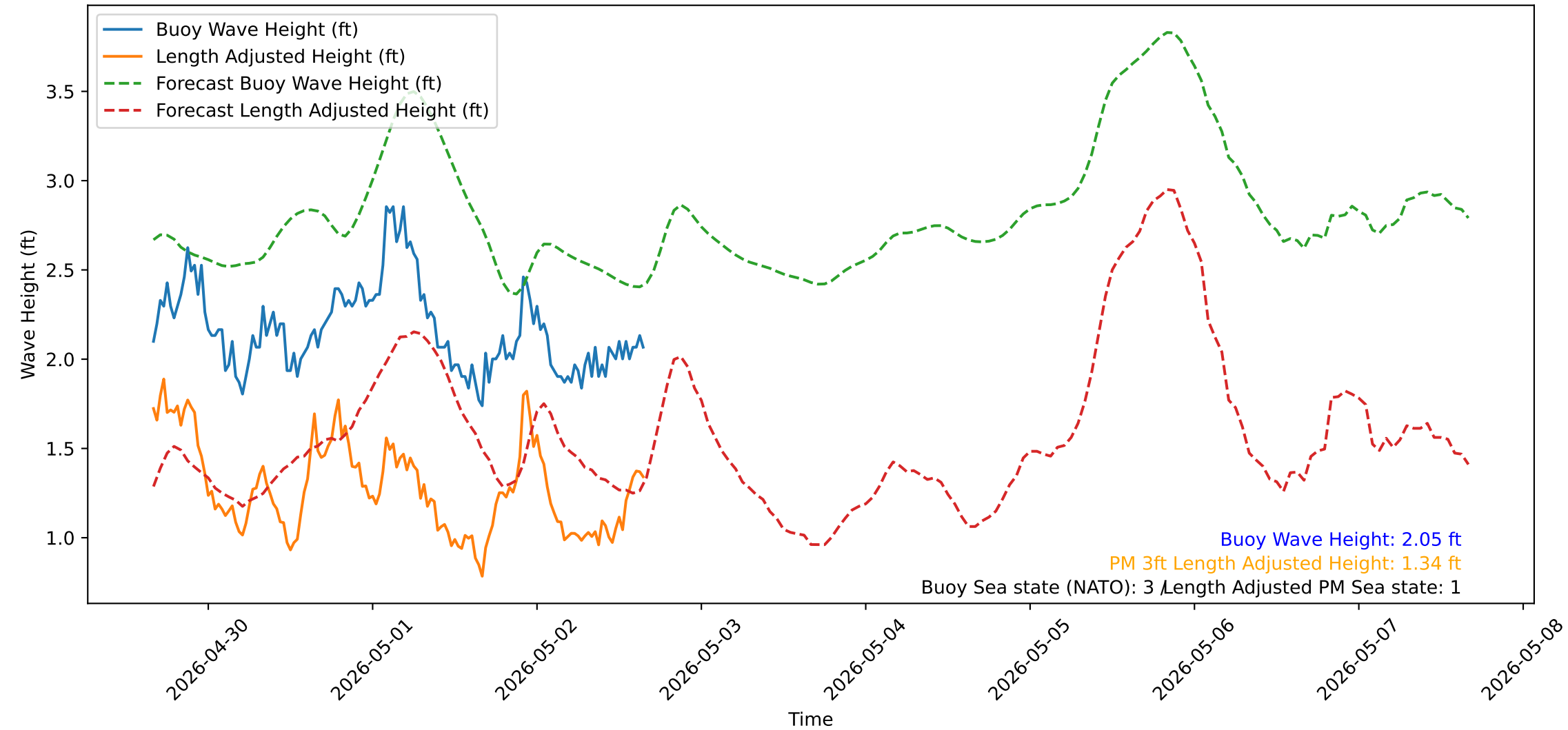
Wave Heights over Time for Green Beach at 2026-05-02 16:11:13
