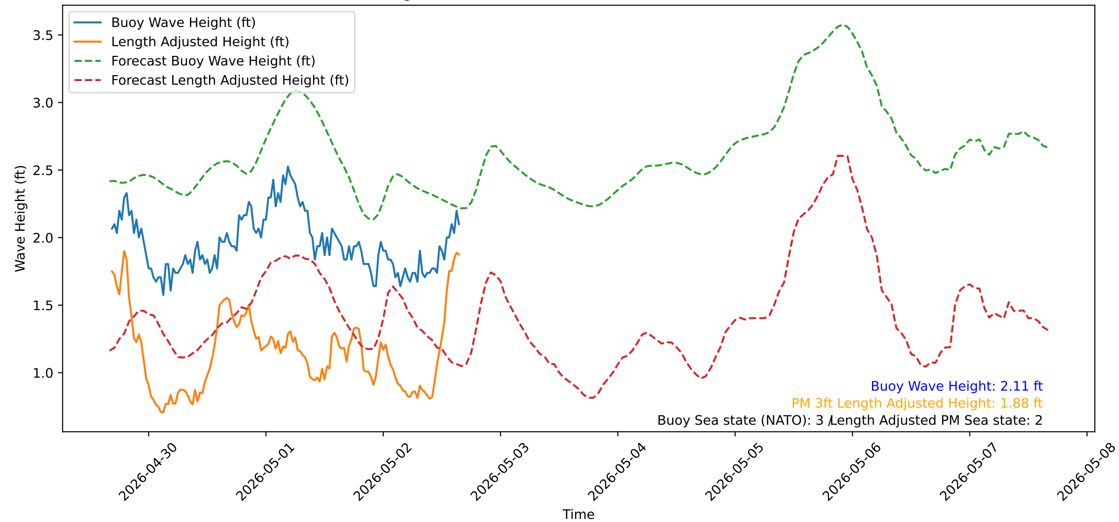
Wave Heights over Time for Red Beach at 2026-05-02 16:10:51
