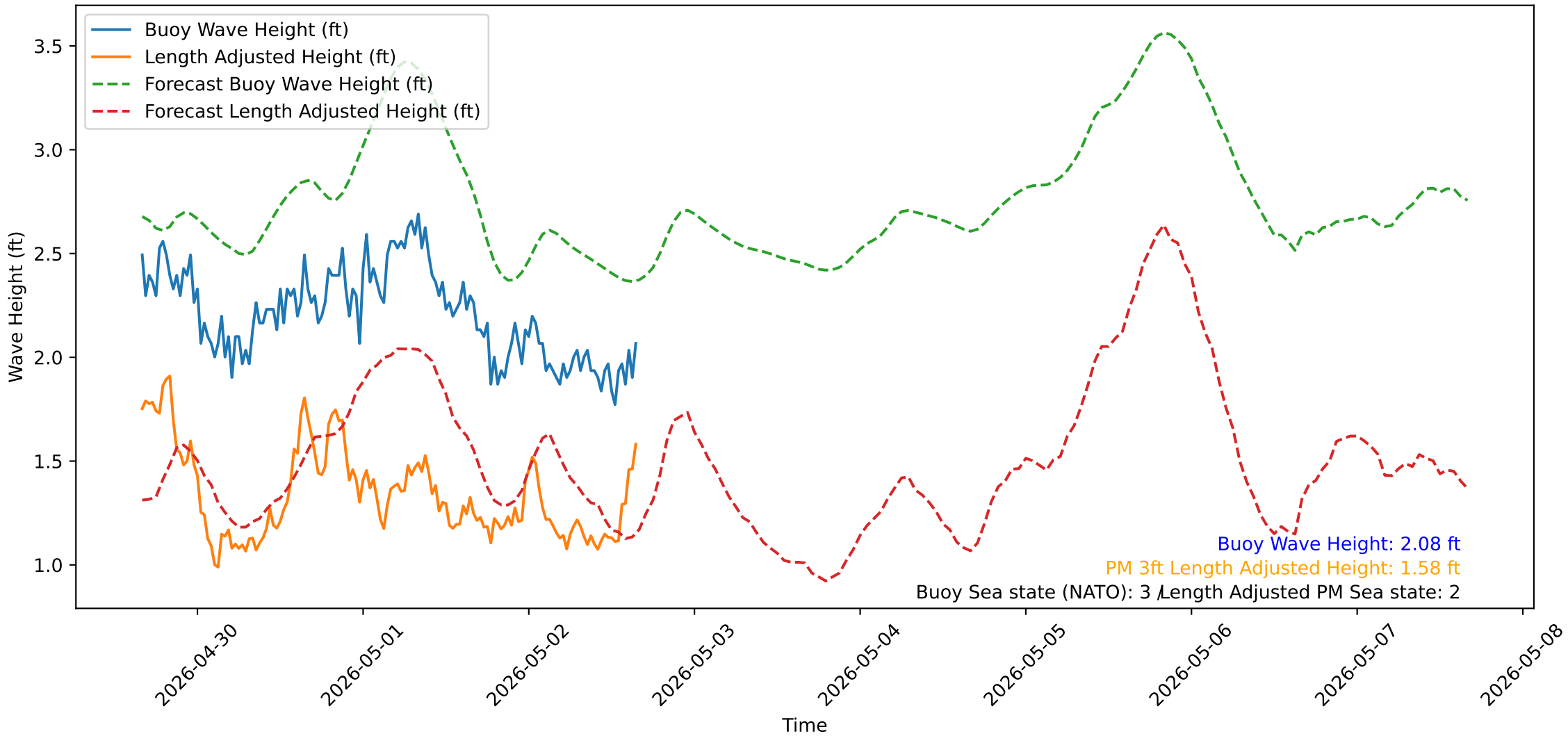
Wave Heights over Time for Oceanside Harbor at 2026-05-02 16:10:31
