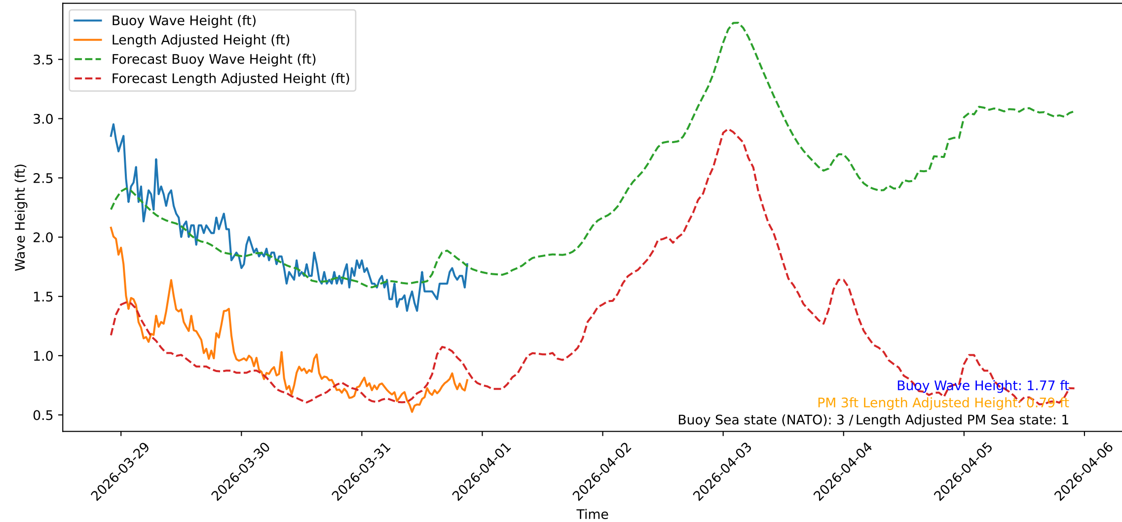
Wave Heights over Time for Red Beach at 2026-03-31 21:50:48
