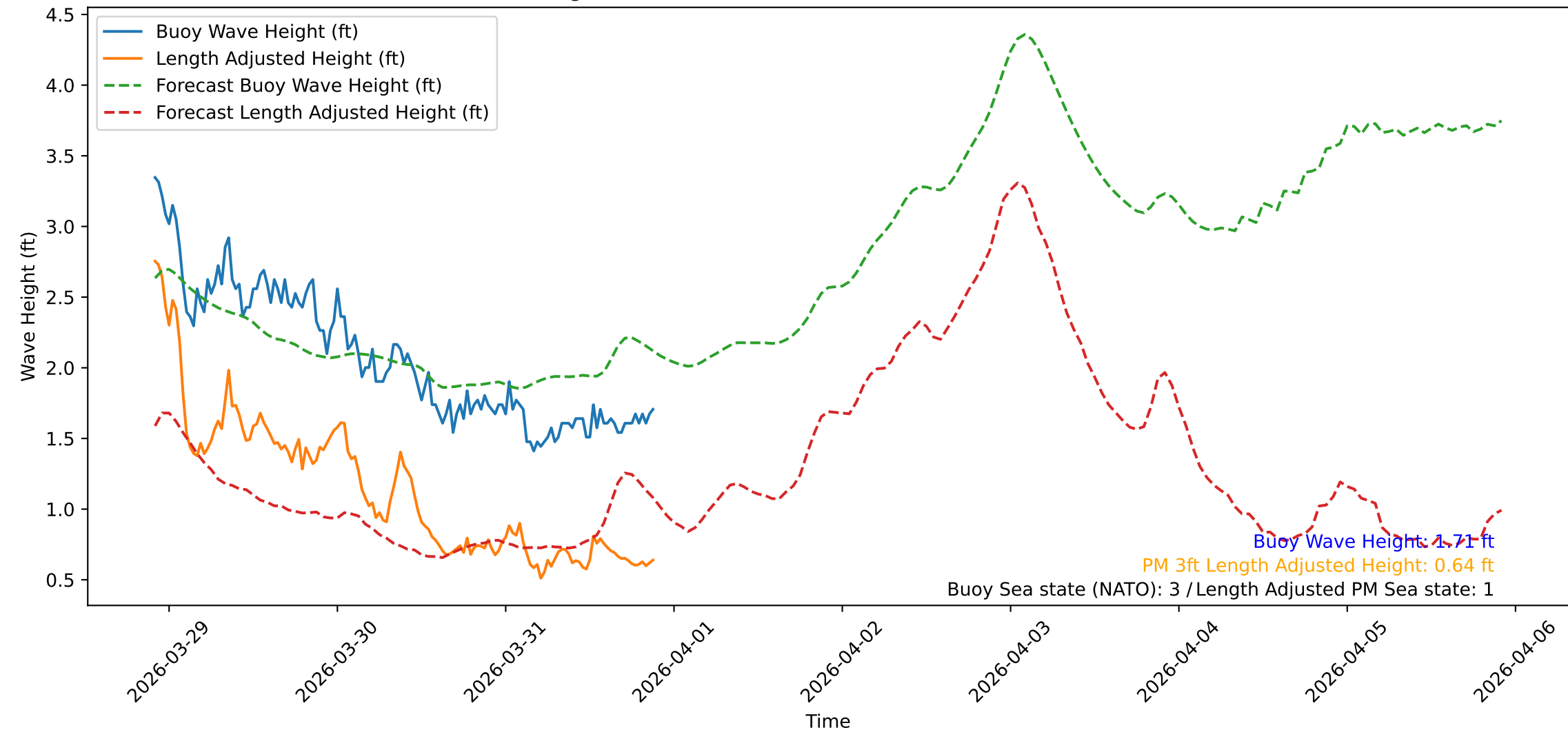
Wave Heights over Time for Green Beach at 2026-03-31 21:51:10
