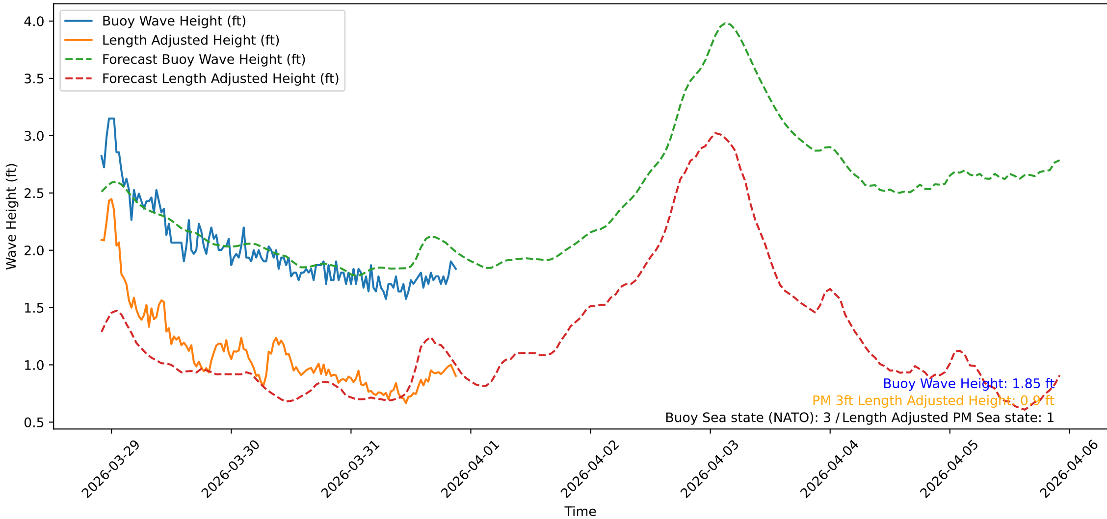
Wave Heights over Time for Oceanside Harbor at 2026-03-31 21:50:31
