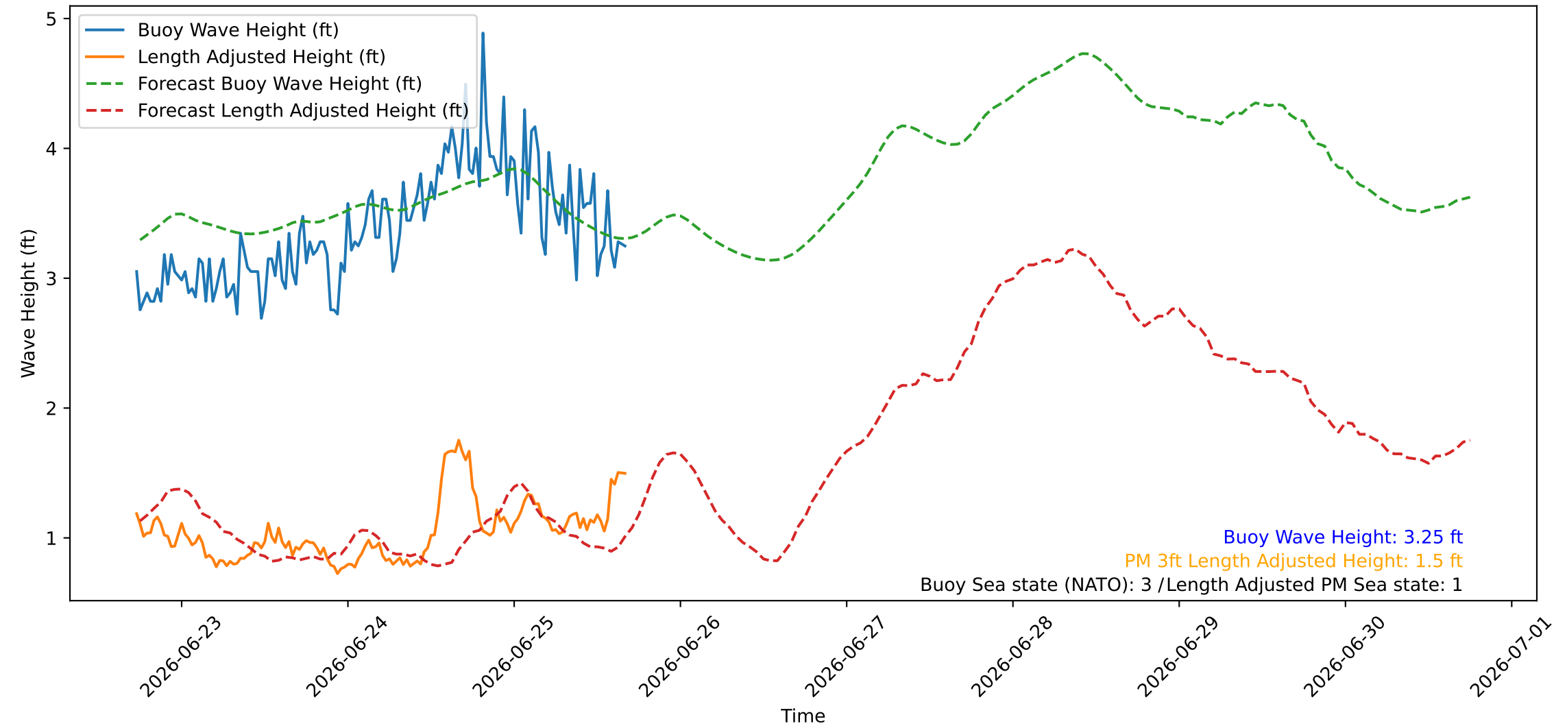
Wave Heights over Time for Oceanside Harbor at 2026-06-25 17:30:26
