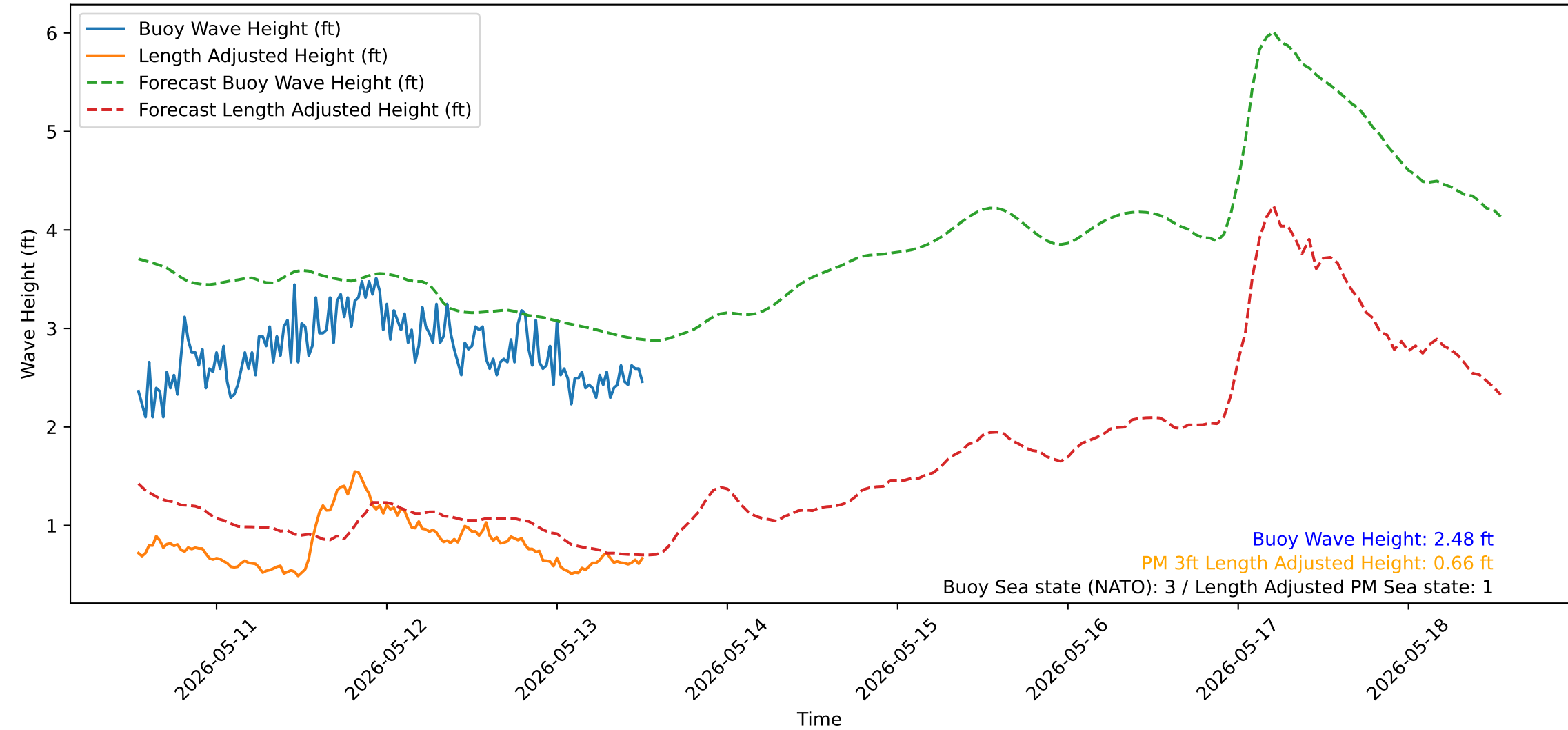
Wave Heights over Time for Green Beach at 2026-05-13 12:51:14
