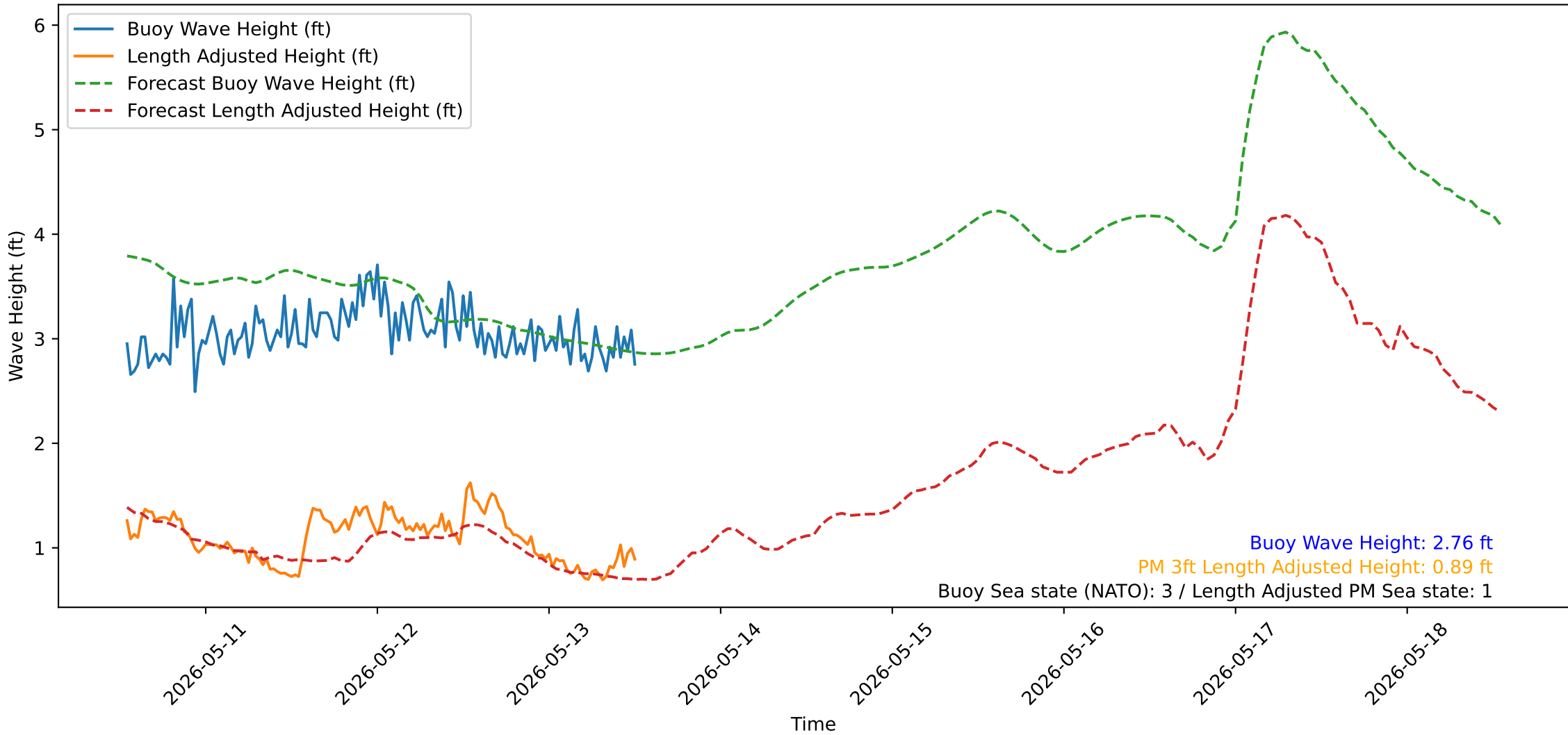
Wave Heights over Time for Oceanside Harbor at 2026-05-13 12:50:31
