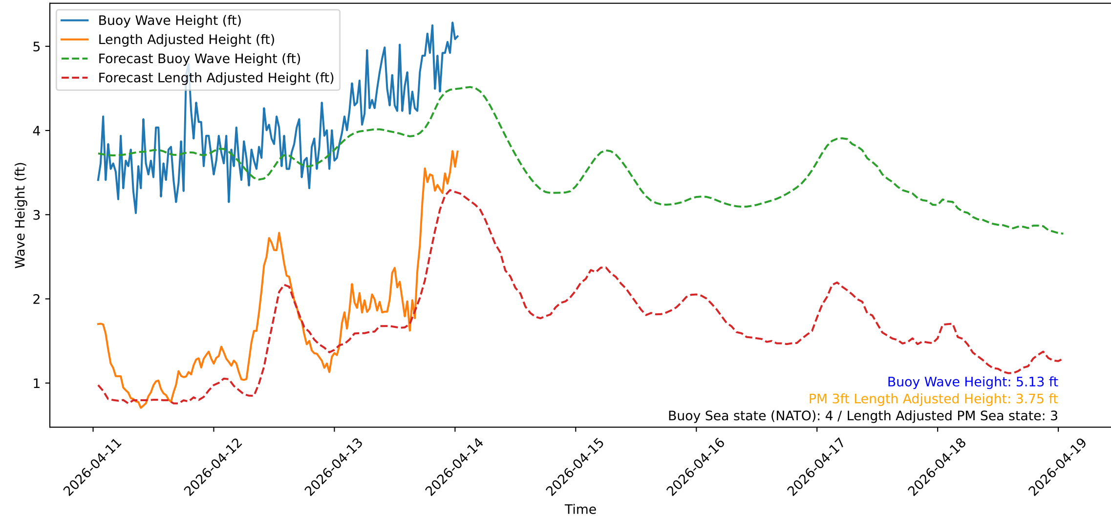
Wave Heights over Time for Oceanside Harbor at 2026-04-14 01:10:31
