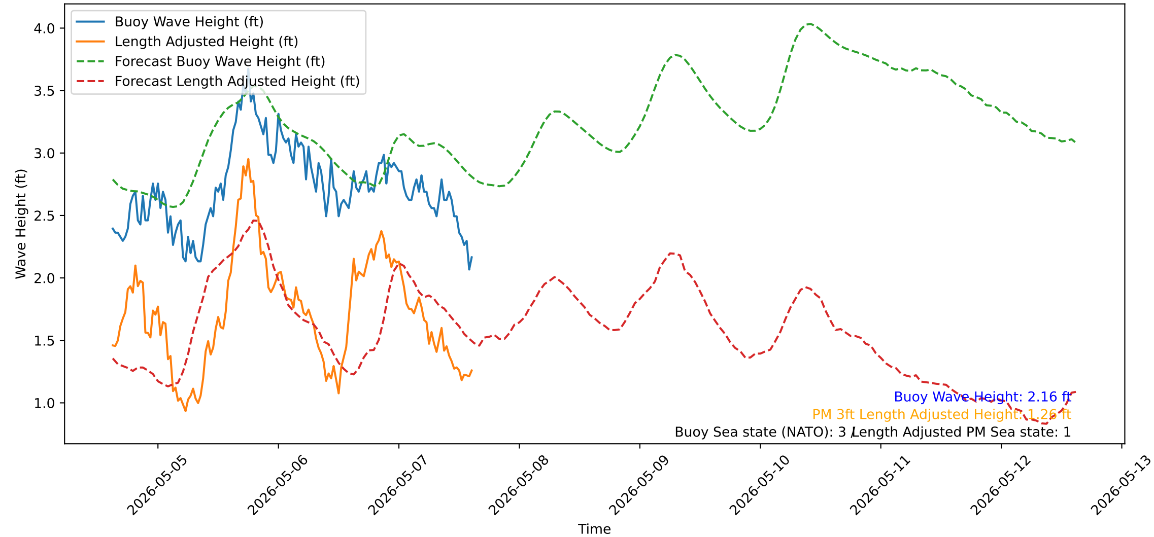
Wave Heights over Time for Green Beach at 2026-05-07 15:11:13
