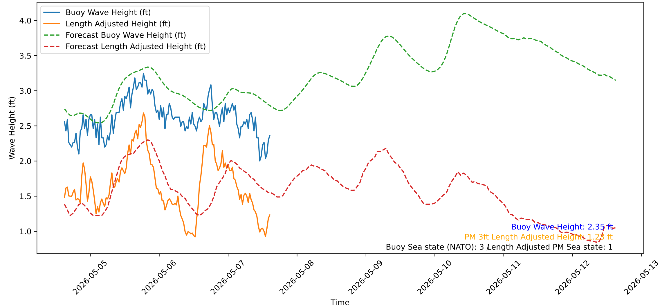
Wave Heights over Time for Oceanside Harbor at 2026-05-07 15:10:32
