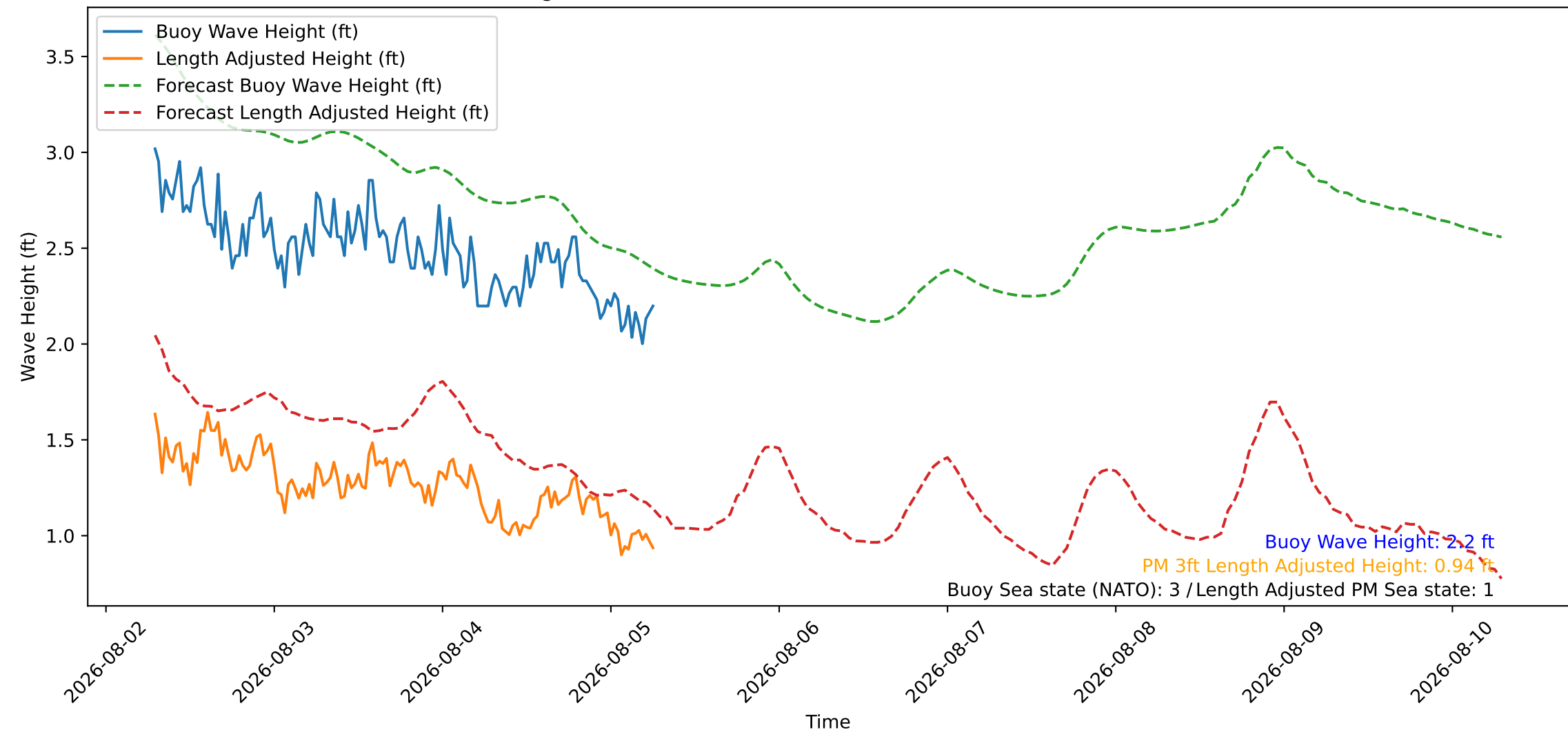
Wave Heights over Time for Oceanside Harbor at 2026-08-05 07:00:26
