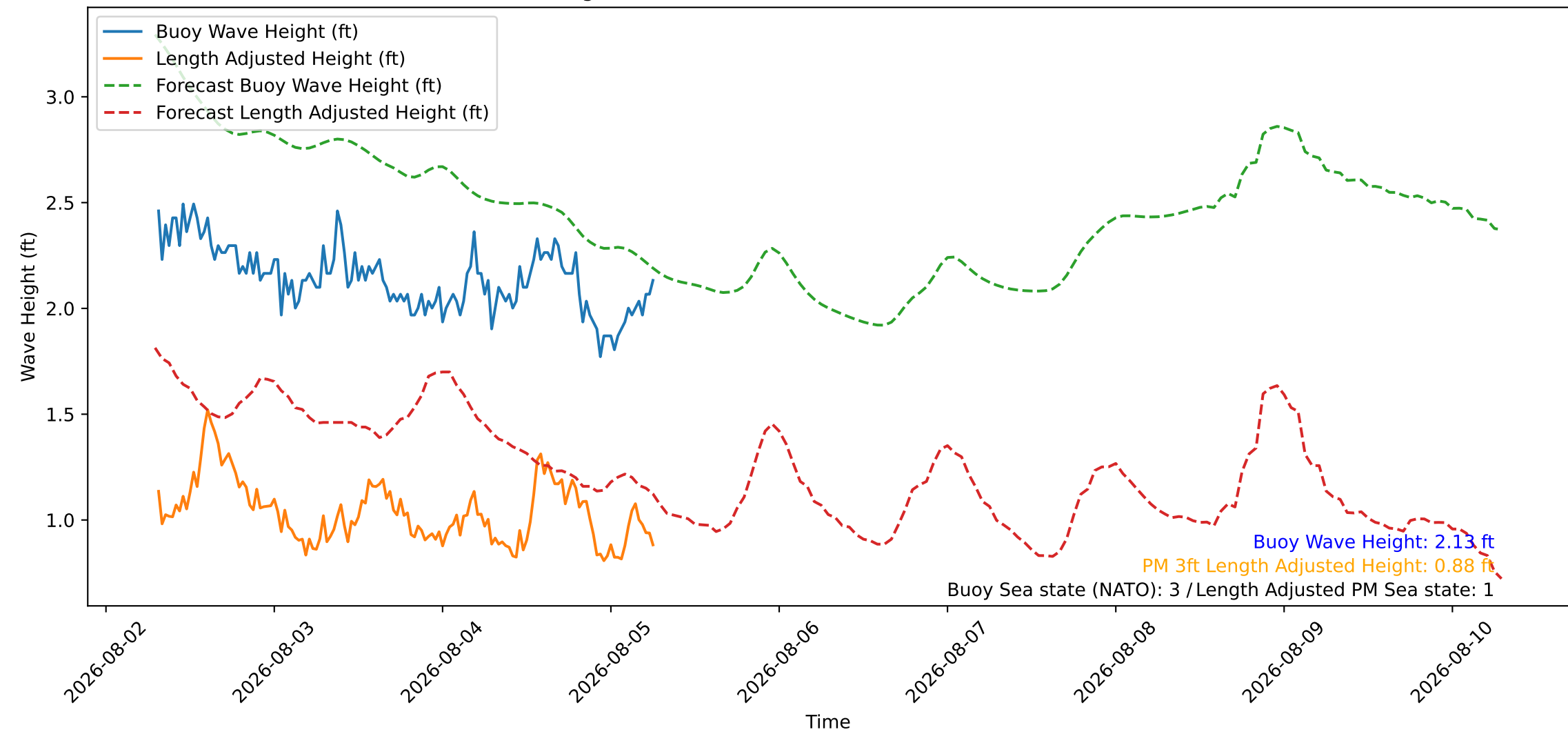
Wave Heights over Time for Red Beach at 2026-08-05 07:00:46
