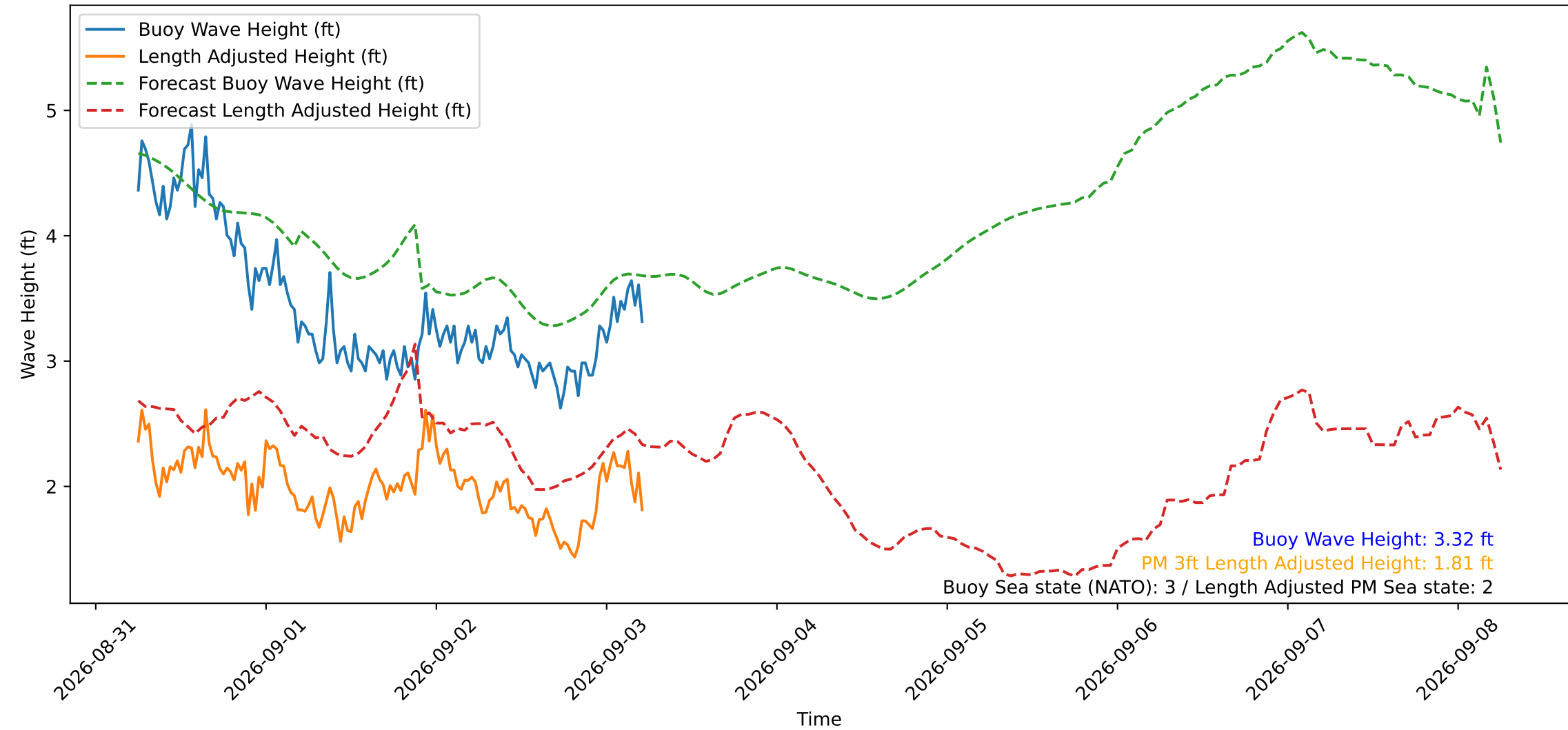
Wave Heights over Time for Oceanside Harbor at 2026-09-03 06:10:29
