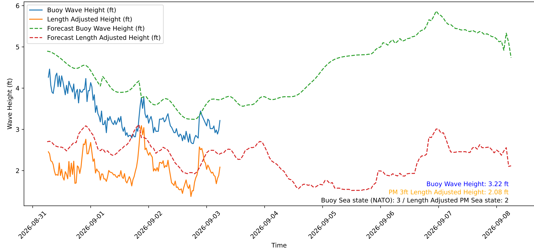
Wave Heights over Time for Green Beach at 2026-09-03 06:11:11
