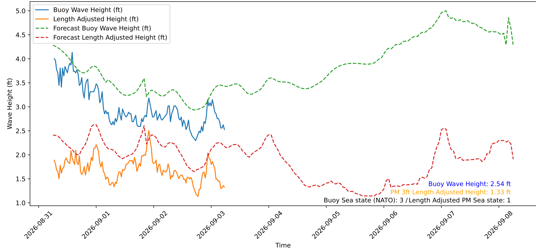
Wave Heights over Time for Red Beach at 2026-09-03 06:10:49
