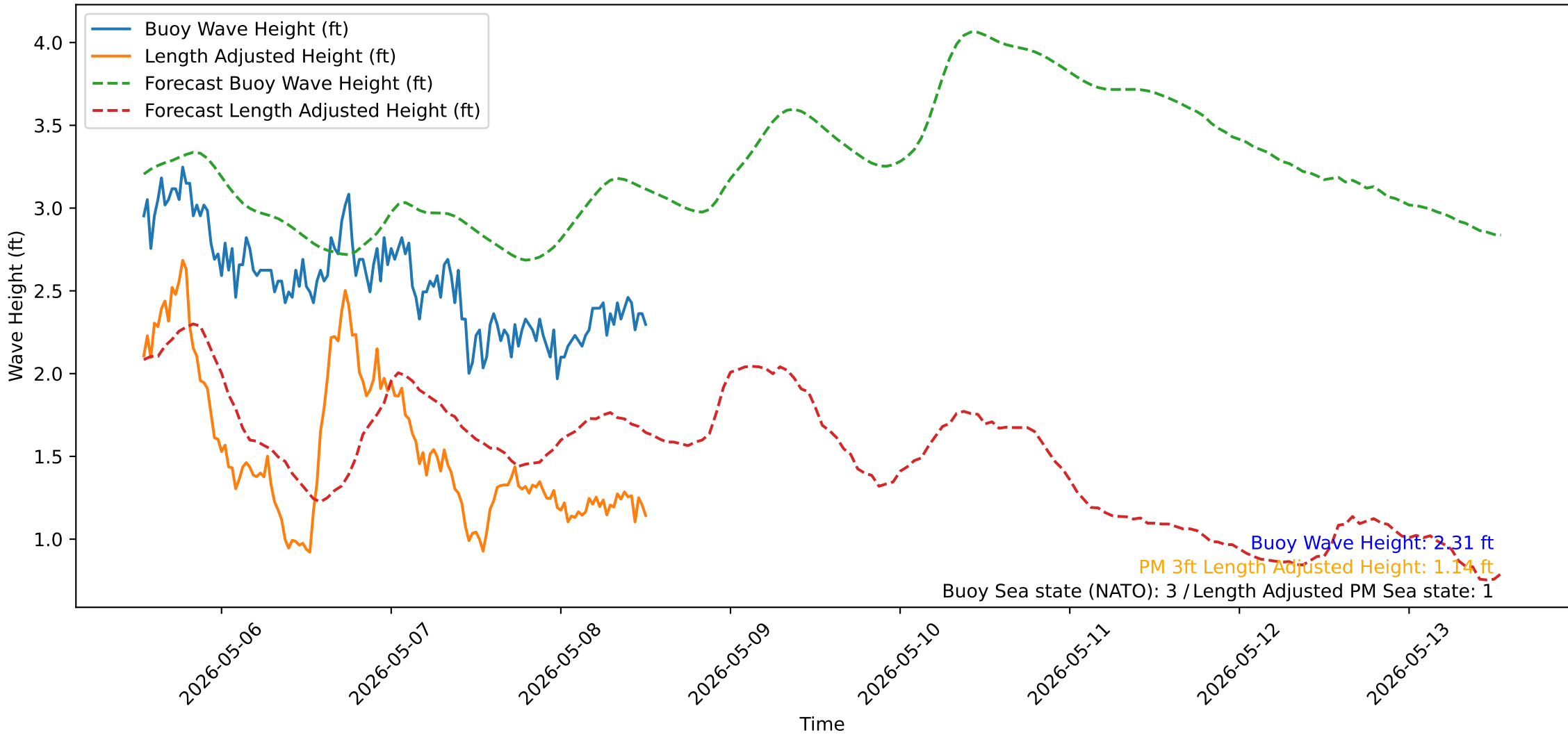
Wave Heights over Time for Oceanside Harbor at 2026-05-08 12:50:31
