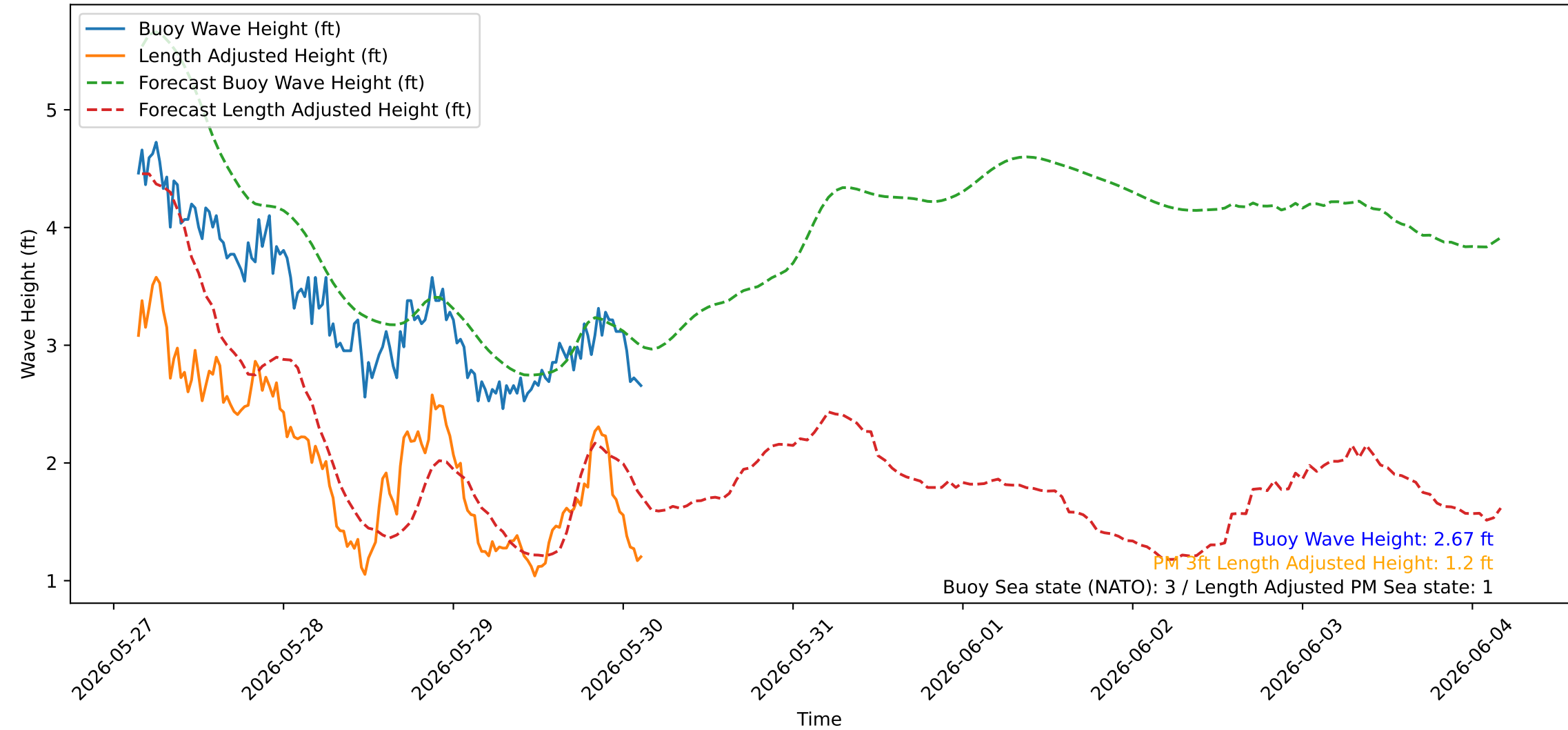
Wave Heights over Time for Green Beach at 2026-05-30 03:31:04
