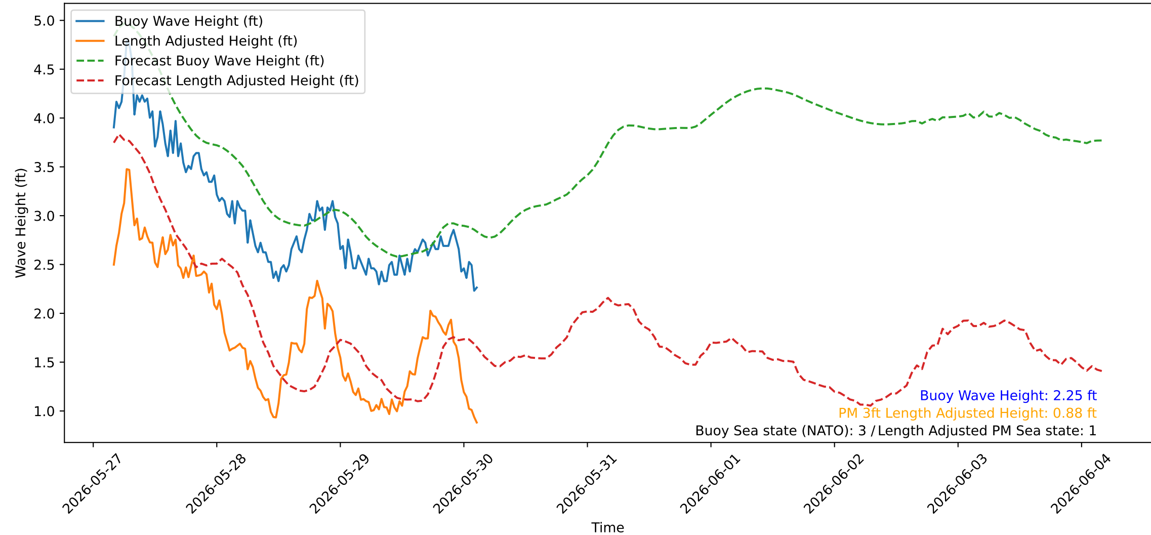
Wave Heights over Time for Red Beach at 2026-05-30 03:30:42
