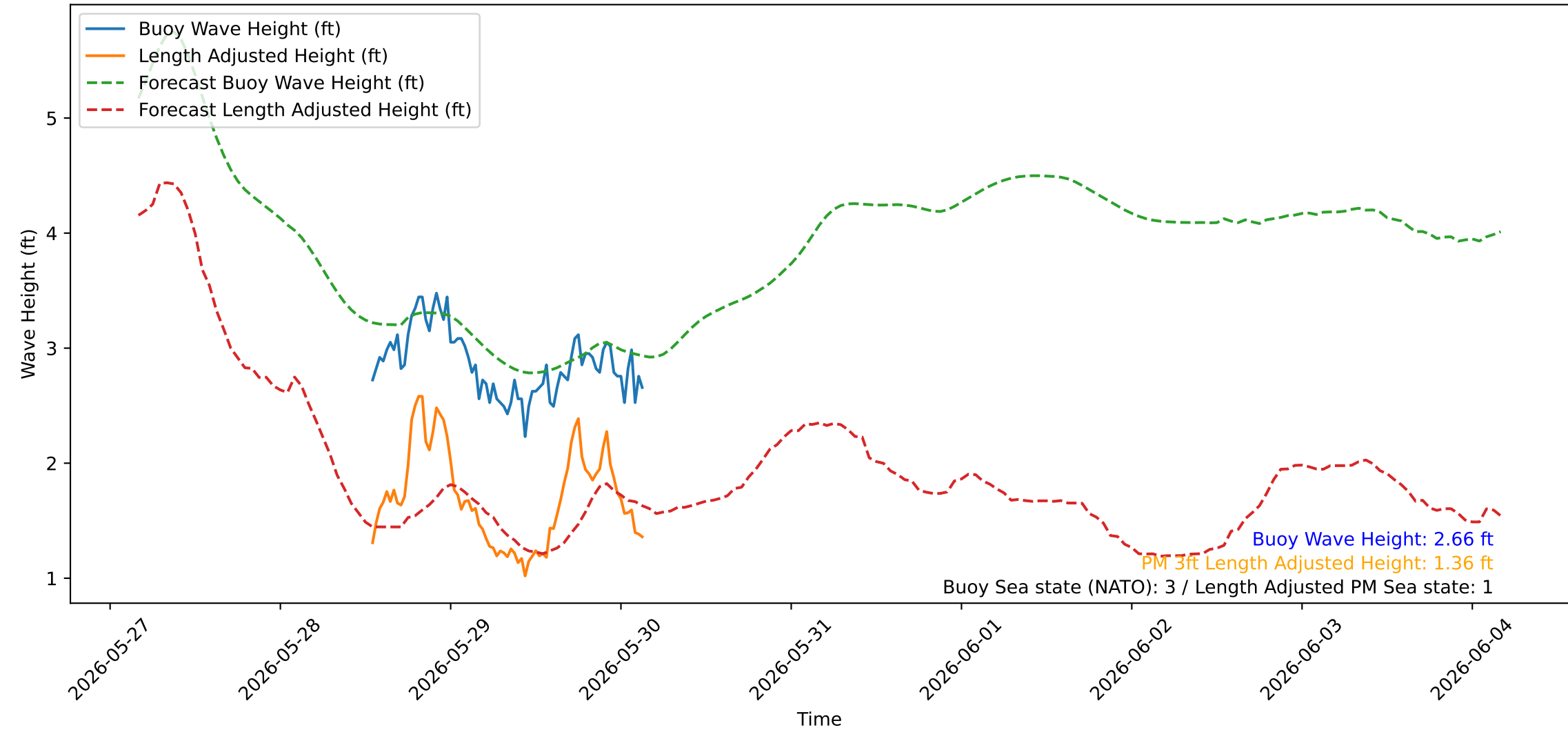
Wave Heights over Time for Oceanside Harbor at 2026-05-30 03:30:23
