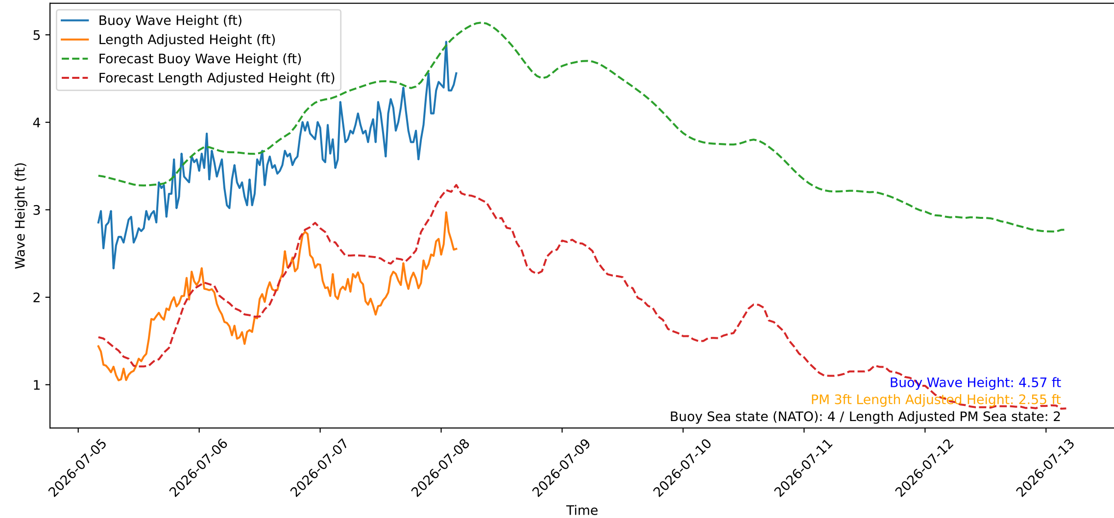
Wave Heights over Time for Oceanside Harbor at 2026-07-08 03:50:26
