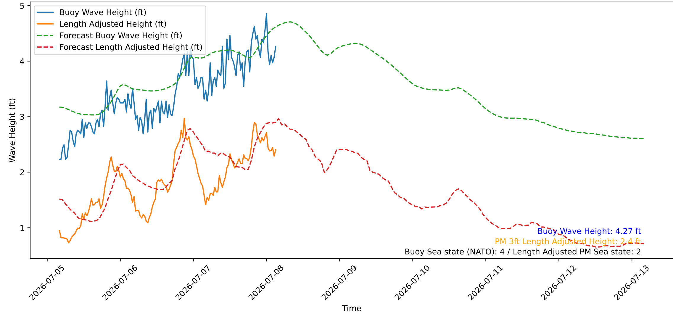
Wave Heights over Time for Red Beach at 2026-07-08 03:50:47
