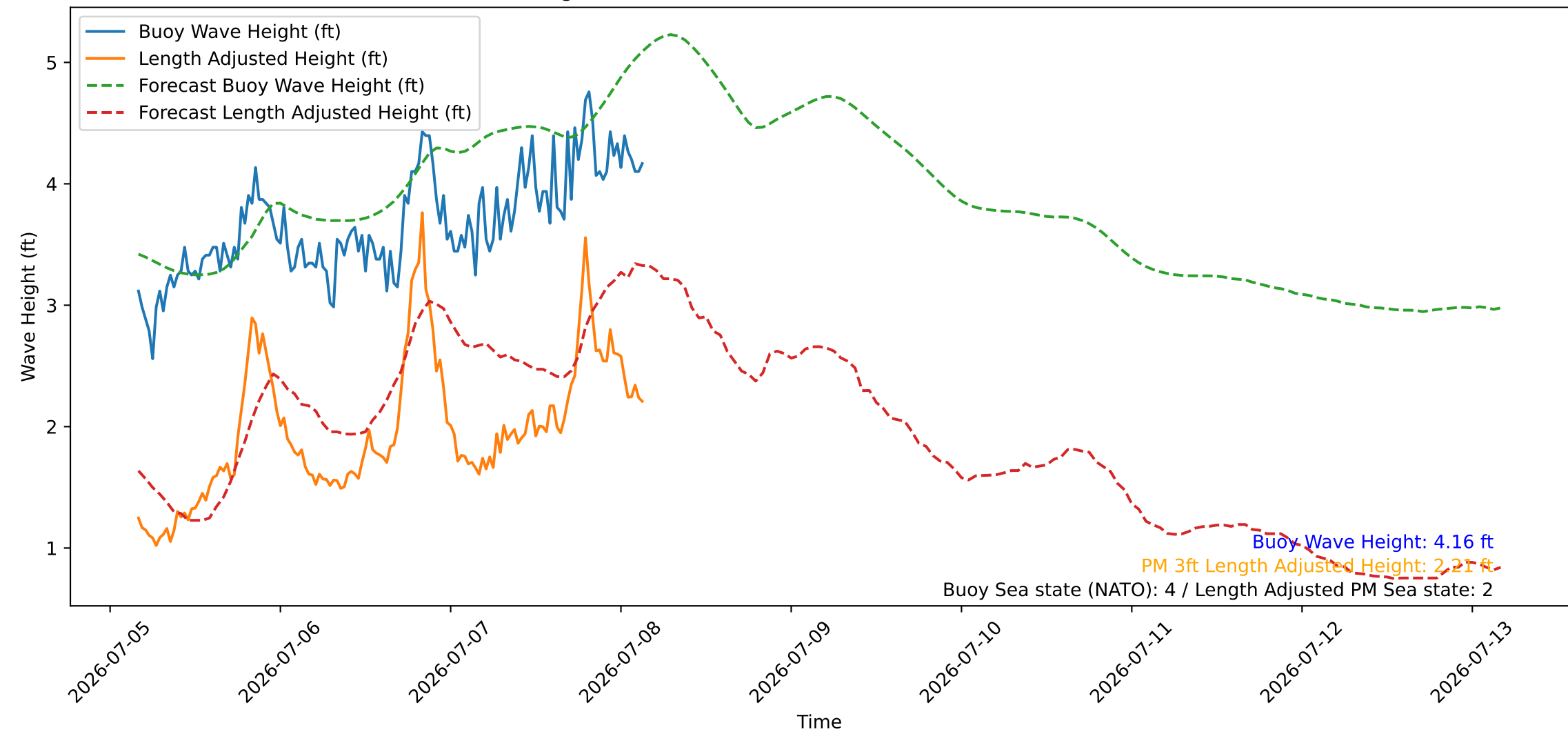
Wave Heights over Time for Green Beach at 2026-07-08 03:51:09
