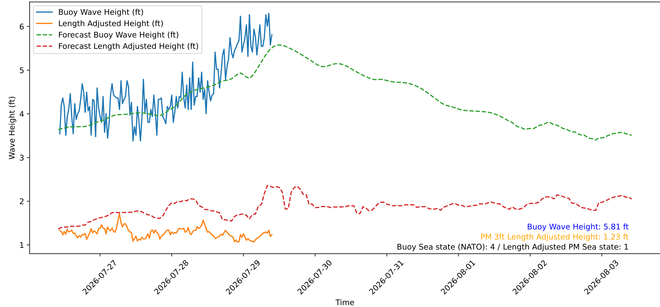
Wave Heights over Time for Green Beach at 2026-07-29 10:21:10
