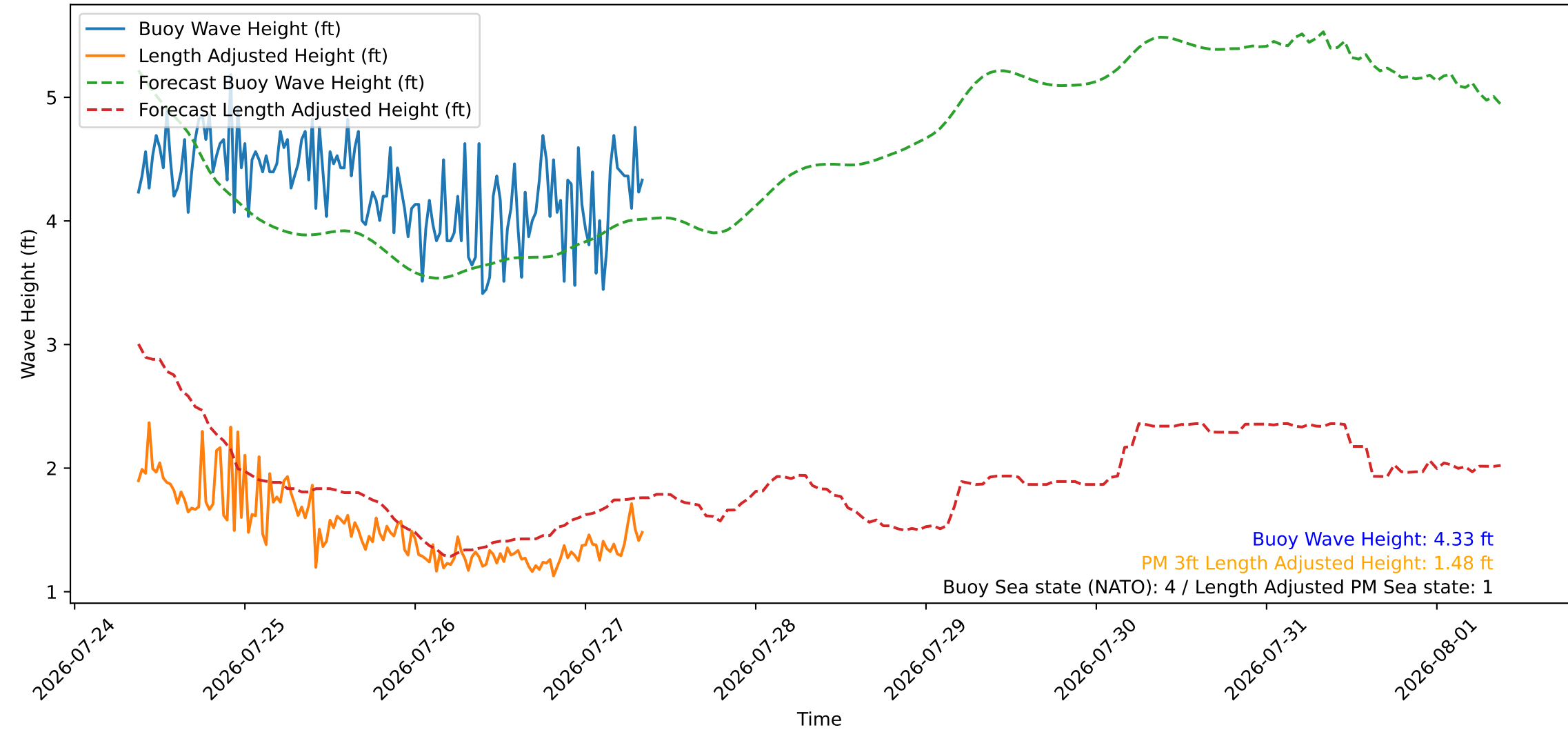
Wave Heights over Time for Green Beach at 2026-07-27 09:01:11
