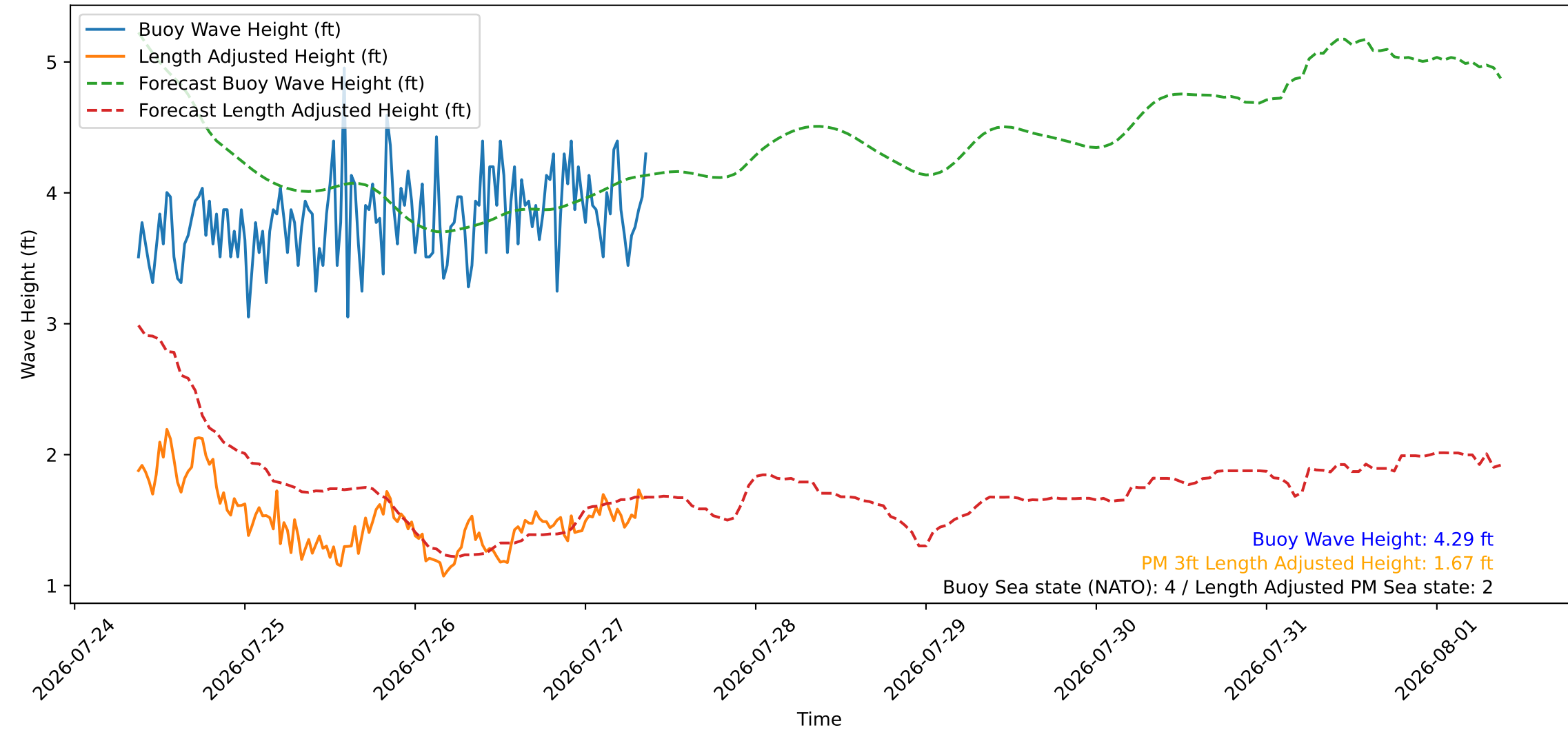
Wave Heights over Time for Oceanside Harbor at 2026-07-27 09:00:29
