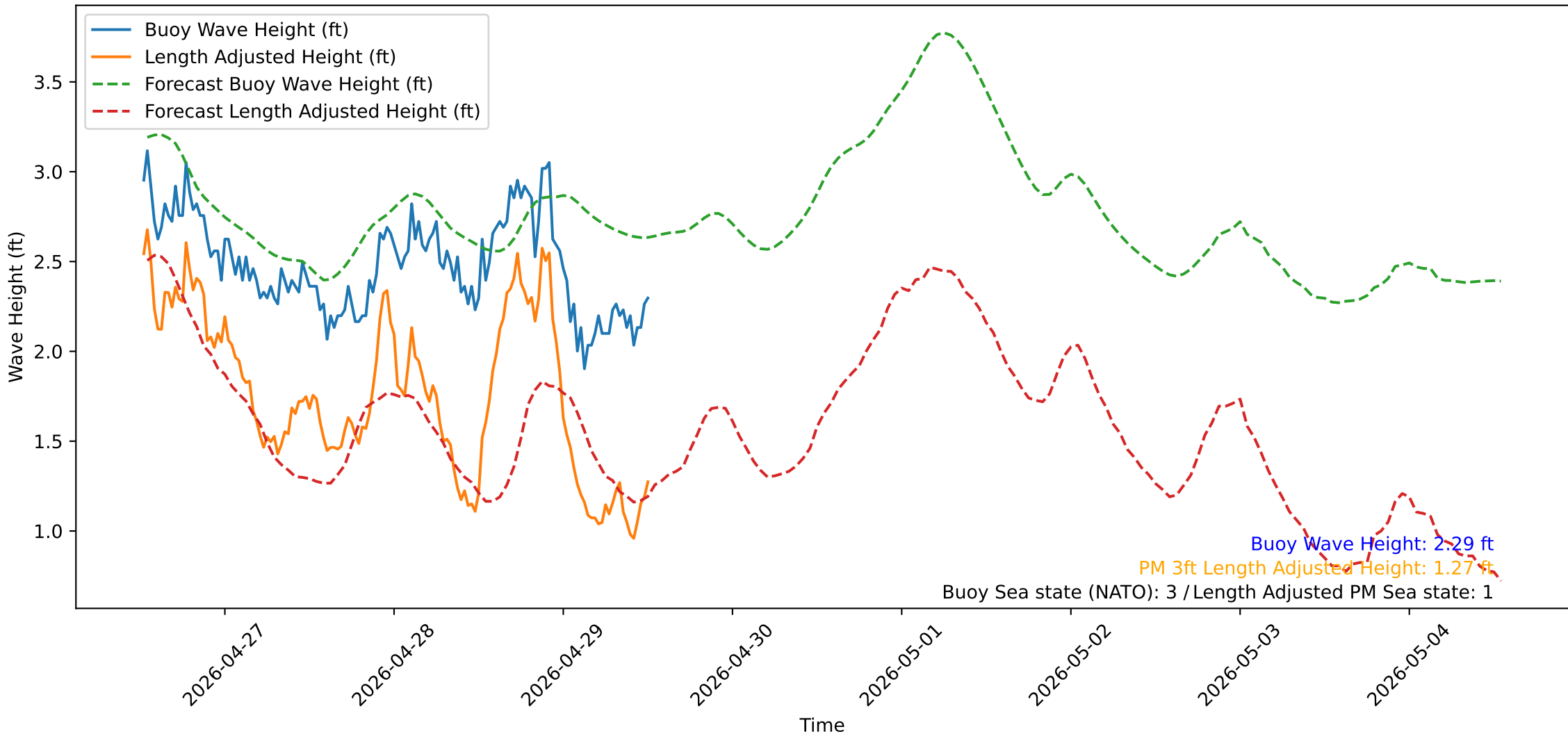
Wave Heights over Time for Oceanside Harbor at 2026-04-29 12:30:32
