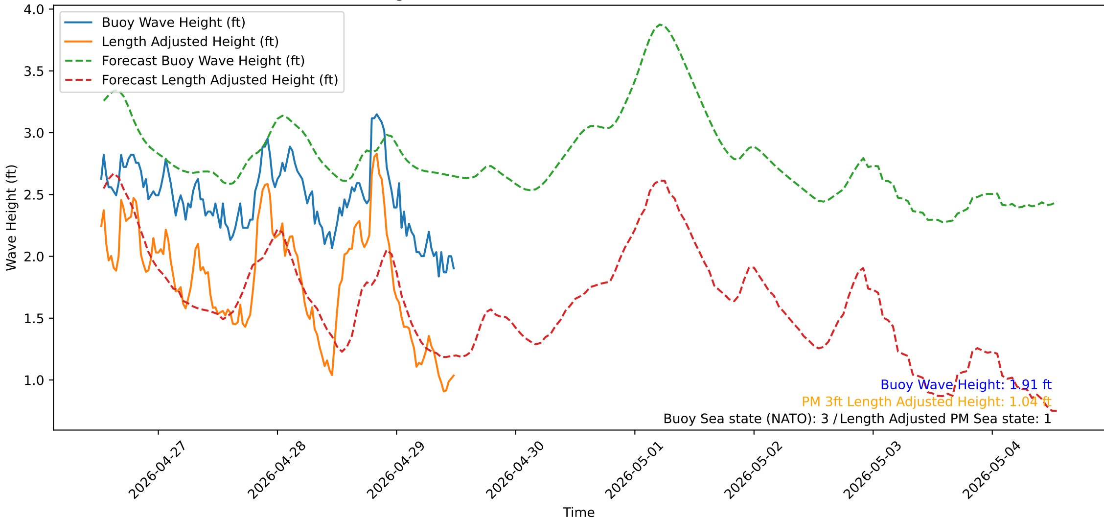
Wave Heights over Time for Green Beach at 2026-04-29 12:31:15
