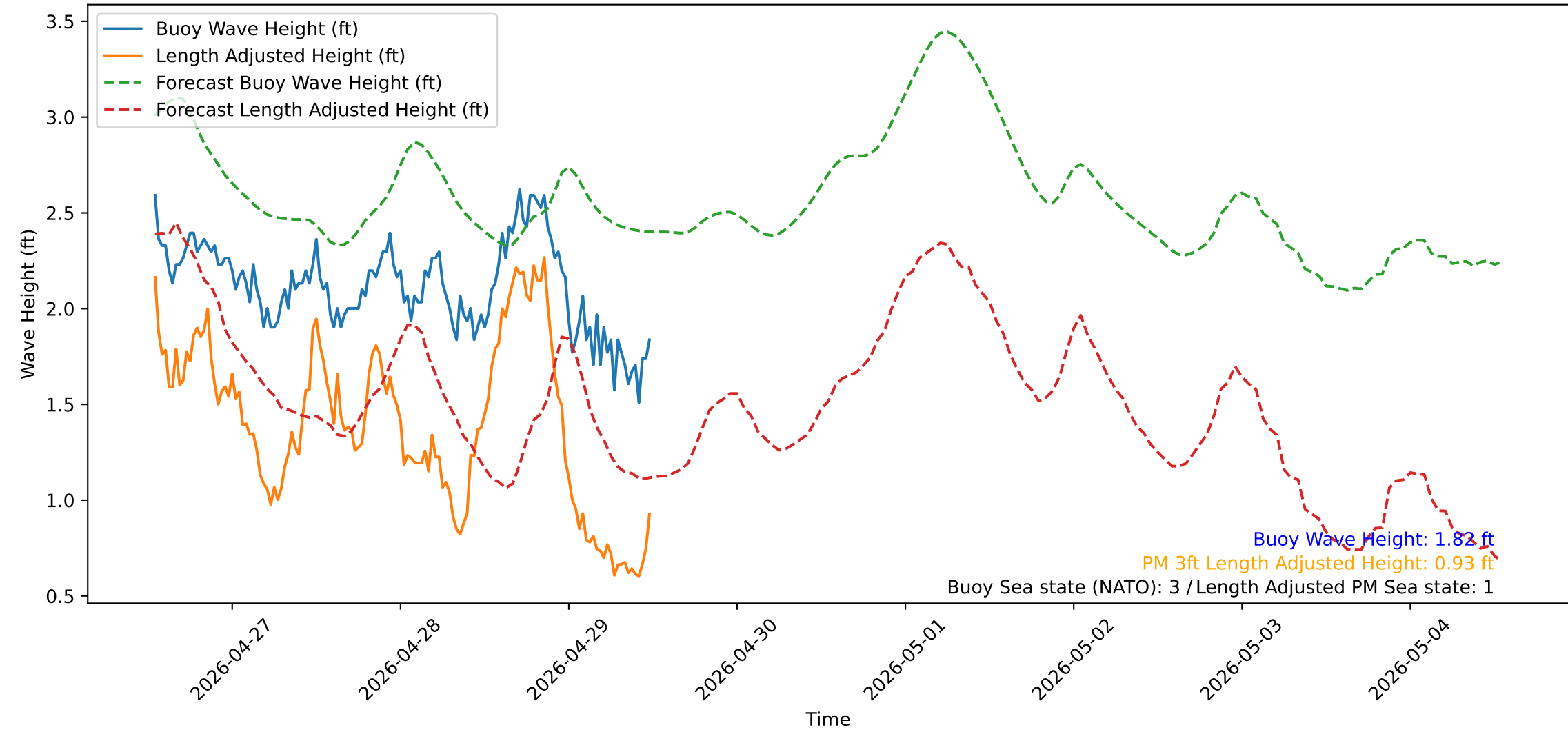
Wave Heights over Time for Red Beach at 2026-04-29 12:30:52
