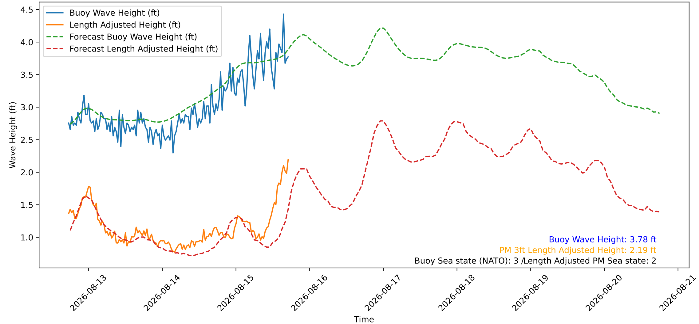
Wave Heights over Time for Oceanside Harbor at 2026-08-15 17:30:27
