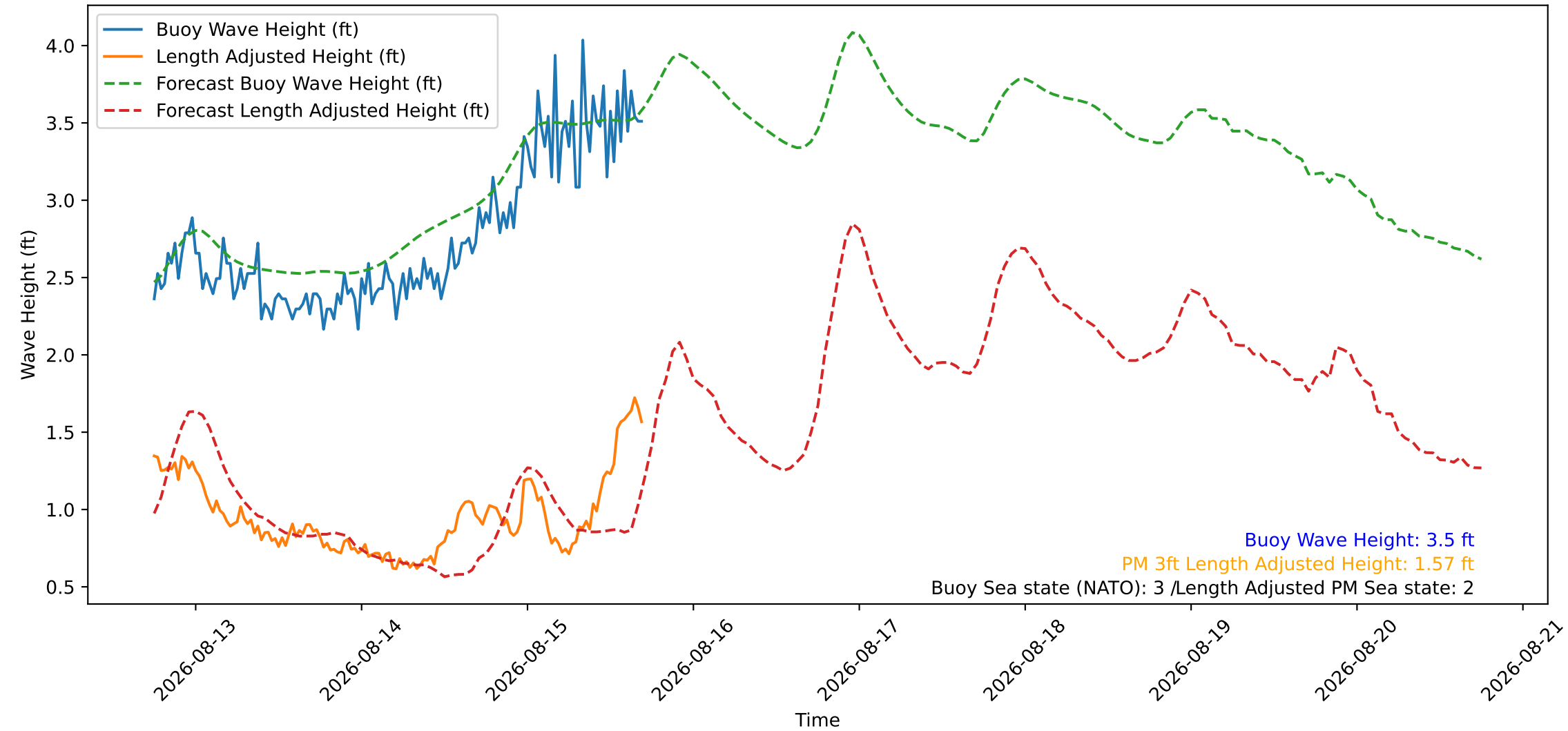
Wave Heights over Time for Red Beach at 2026-08-15 17:30:46
