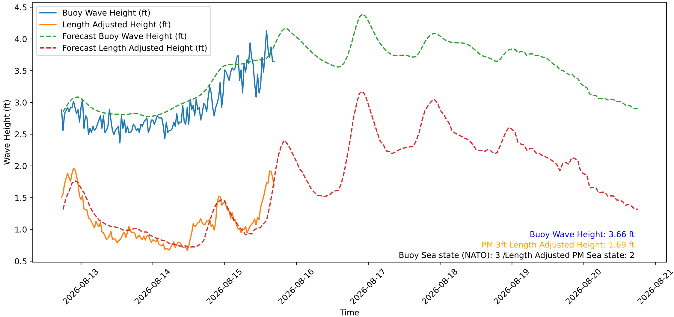
Wave Heights over Time for Green Beach at 2026-08-15 17:31:08
