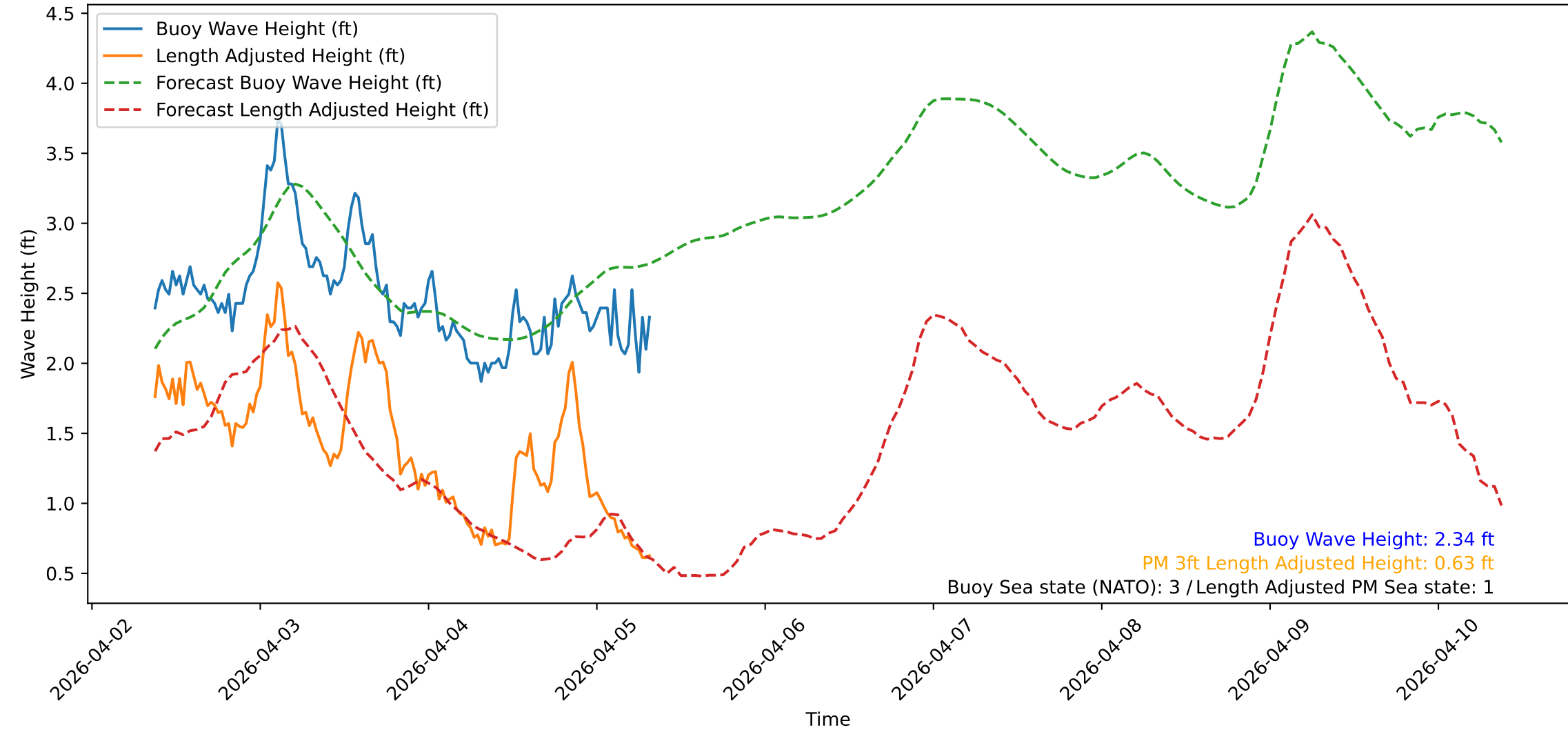
Wave Heights over Time for Red Beach at 2026-04-05 08:30:47
