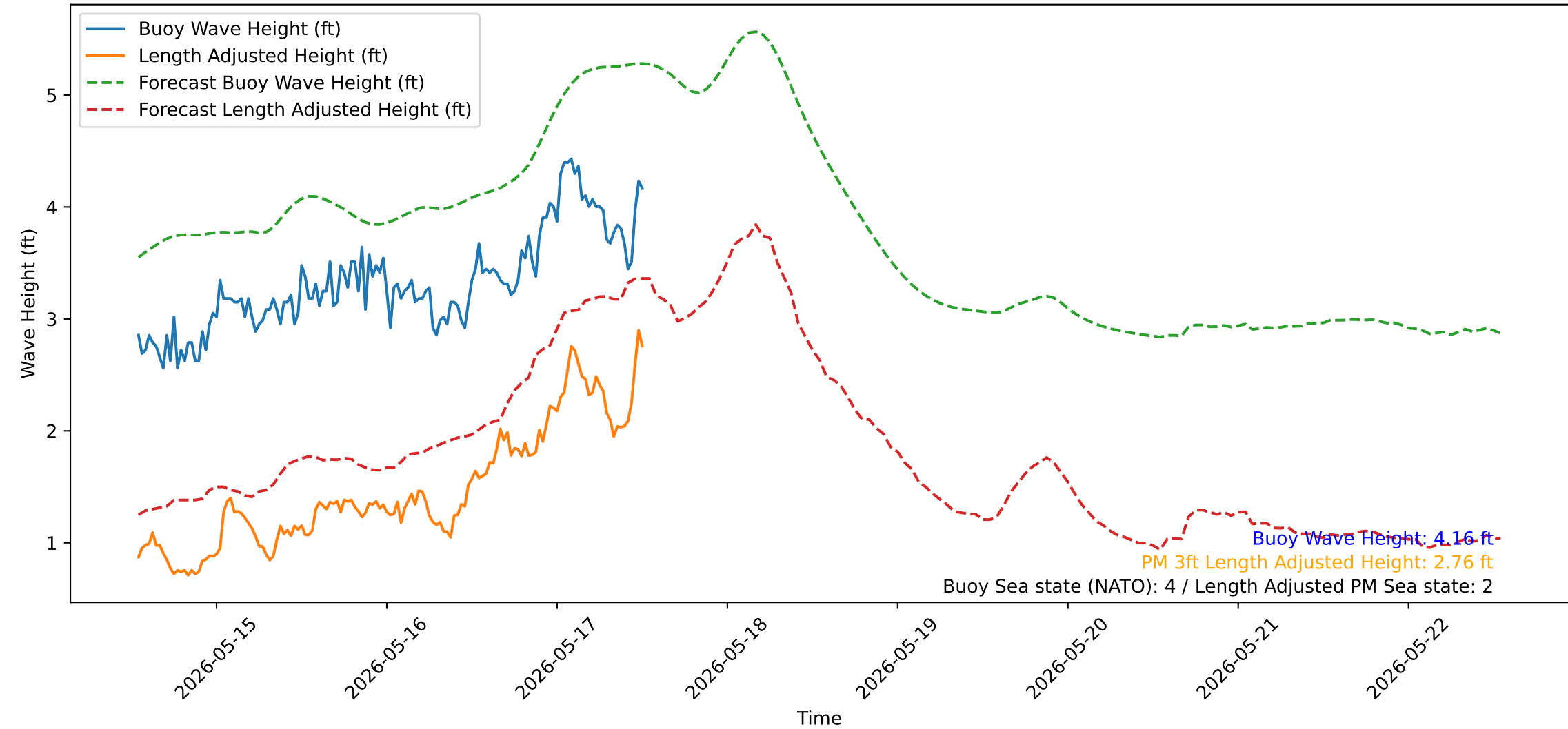
Wave Heights over Time for Green Beach at 2026-05-17 12:51:14
