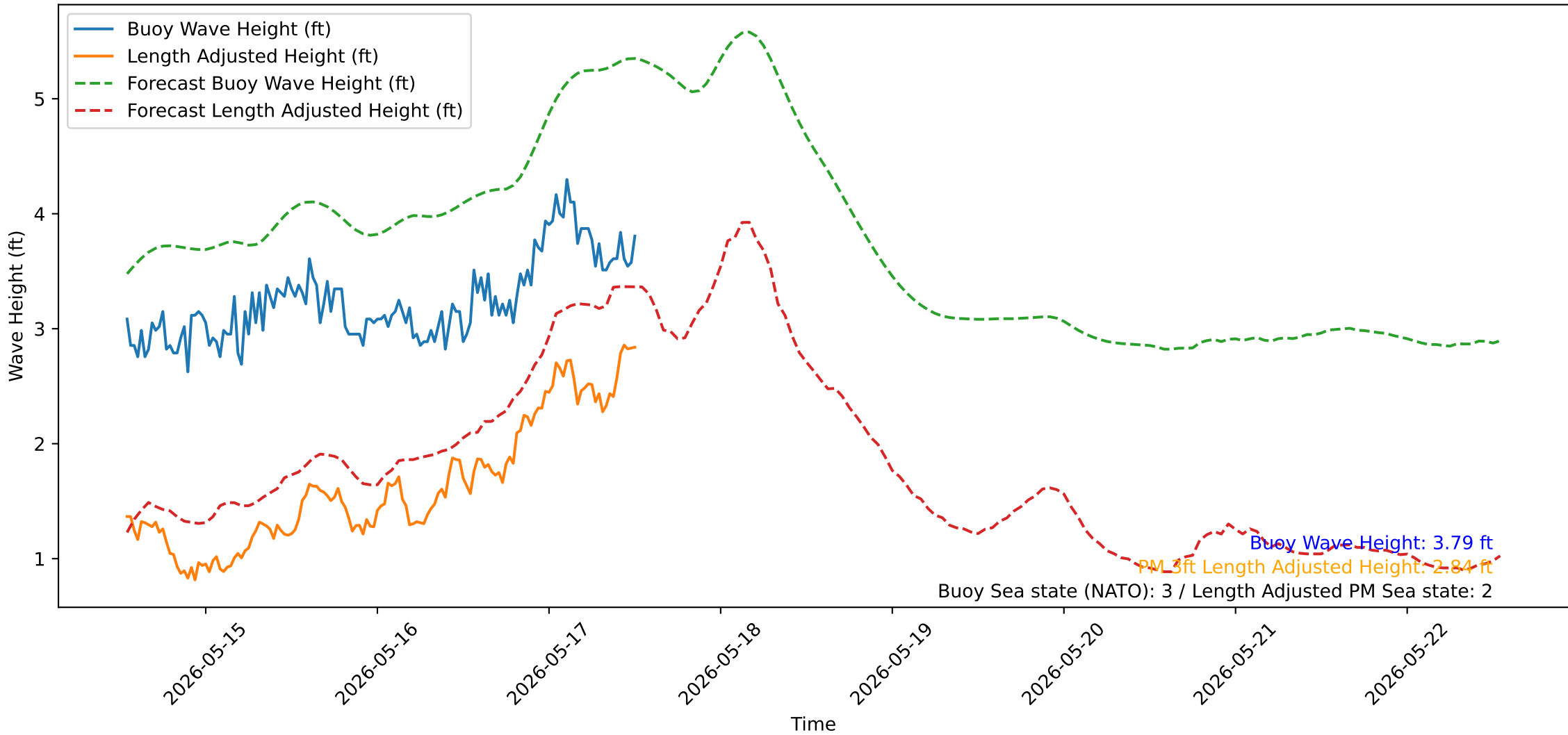
Wave Heights over Time for Oceanside Harbor at 2026-05-17 12:50:31
