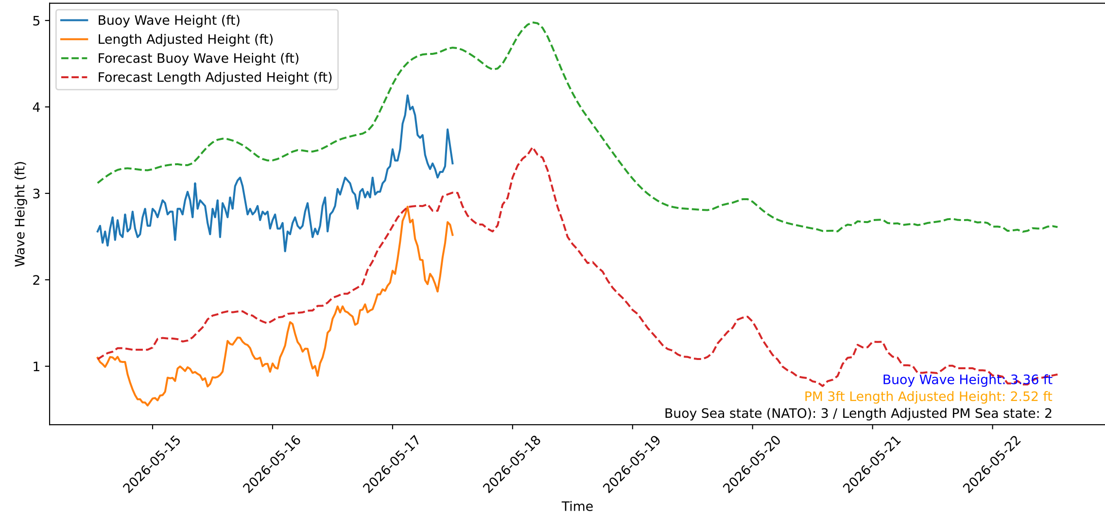
Wave Heights over Time for Red Beach at 2026-05-17 12:50:51
