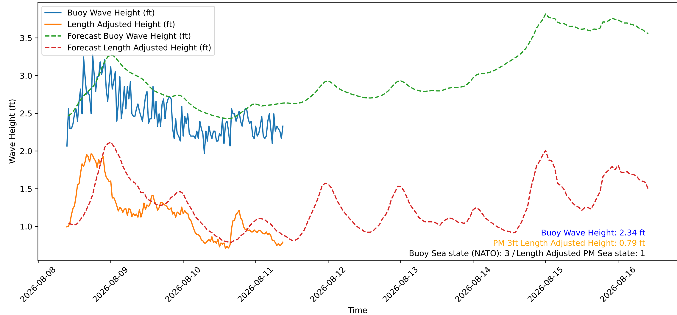
Wave Heights over Time for Oceanside Harbor at 2026-08-11 09:40:26
