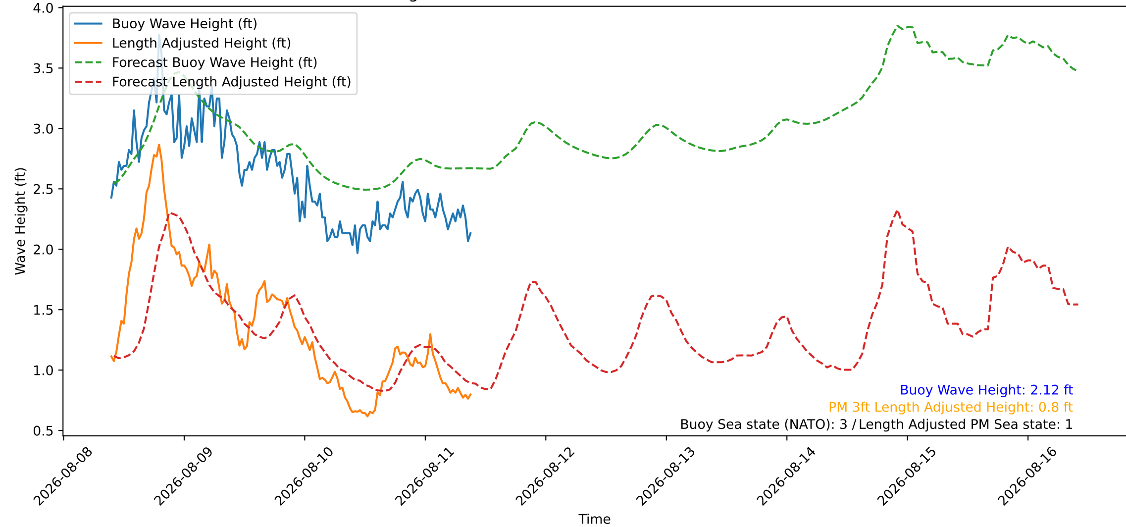
Wave Heights over Time for Green Beach at 2026-08-11 09:41:08
